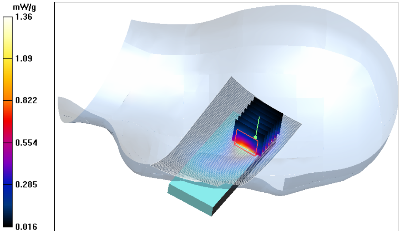
Figure 37 Left Hand Touch Cheek GSM 1900 Channel 661
