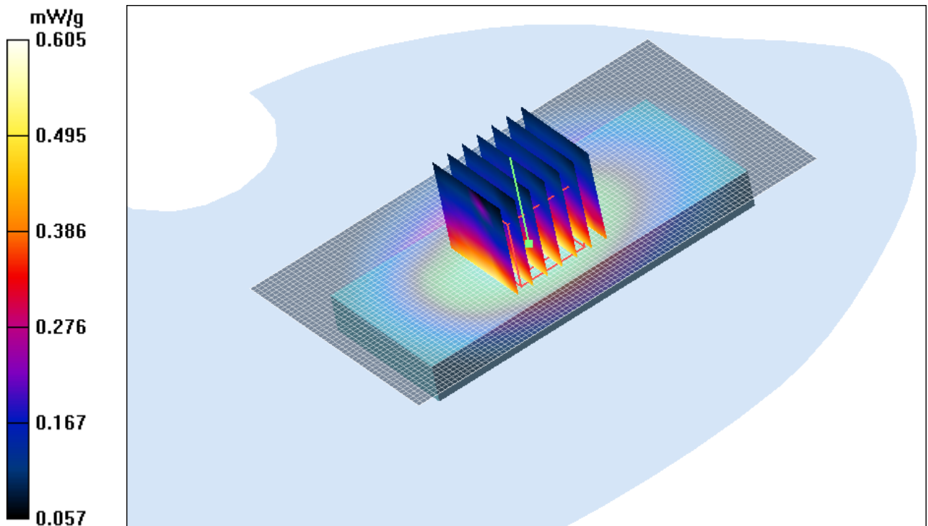
Figure 31 Body, Towards Ground, GSM 850 Channel 128
