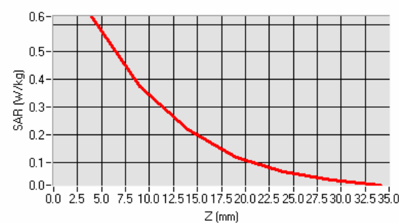
SAR, Z Axis Scan (X = -8, Y = -8)
