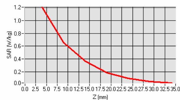
SAR, Z Axis Scan (X = 1, Y = 38)
