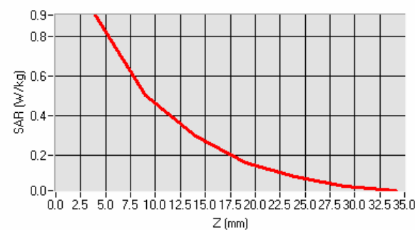
SAR, Z Axis Scan (X = -16, Y = 1)
