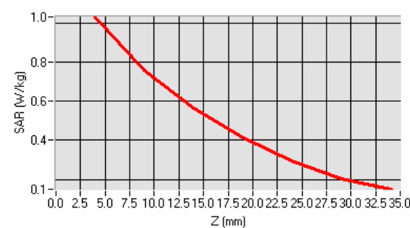
SAR, Z Axis Scan (X = -17, Y = -6)
