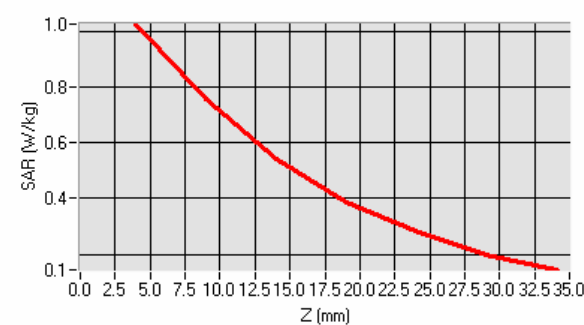
SAR, Z Axis Scan (X = -14, Y = -5)
