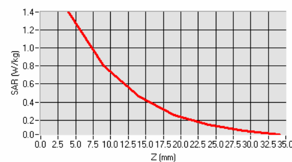
SAR, Z Axis Scan (X = -22, Y = 0)
