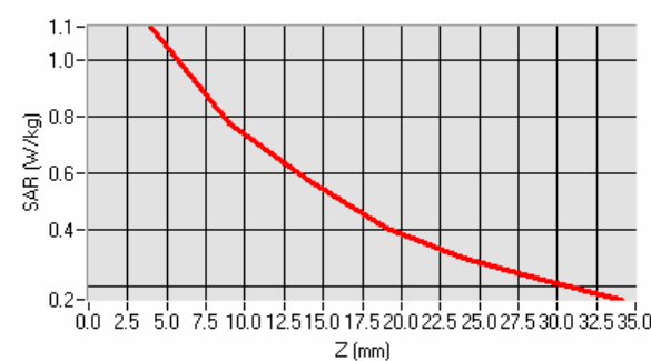
SAR, Z Axis Scan (X = -21, Y = -7)
