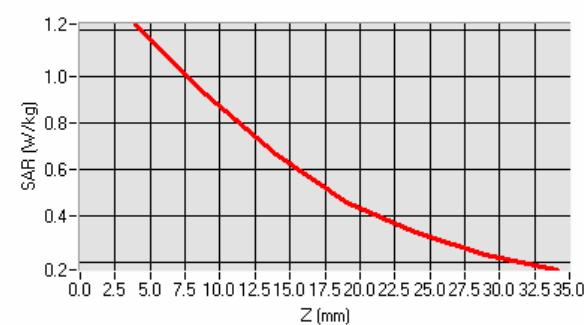
SAR, Z Axis Scan (X = -20, Y = -9)
