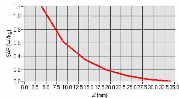
SAR, Z Axis Scan (X = -17, Y = 5)
