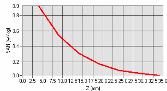
SAR, Z Axis Scan (X = -14, Y = -7)
