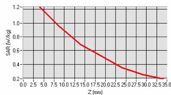
SAR, Z Axis Scan (X = -23, Y = -8)
