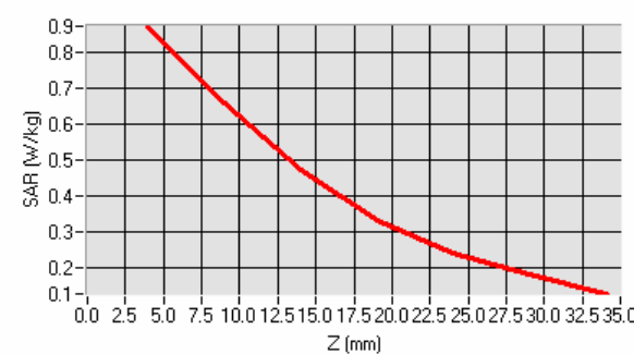
SAR, Z Axis Scan (X = -15, Y = -6)
