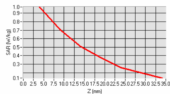
SAR, Z Axis Scan (X = -15, Y = -5)
