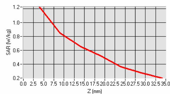
SAR, Z Axis Scan (X = -22, Y = -7)
