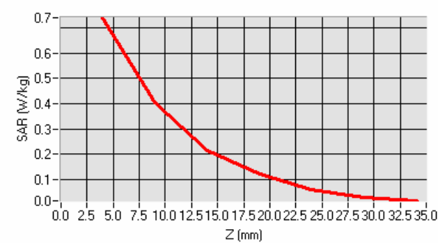
SAR, Z Axis Scan (X = -7, Y = 7)
