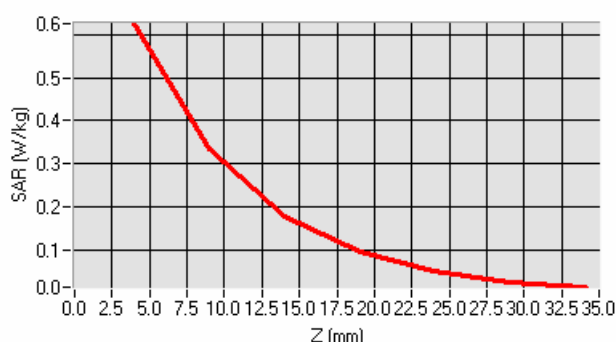
SAR, Z Axis Scan (X = -1, Y = -5)
