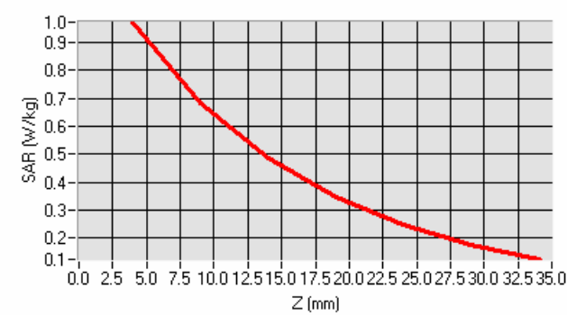
SAR, Z Axis Scan (X = -26, Y = -14)
