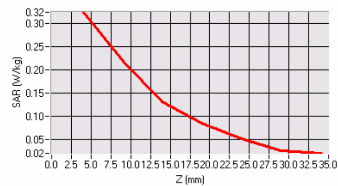
SAR, Z Axis Scan (X = -8,Y = -24)
