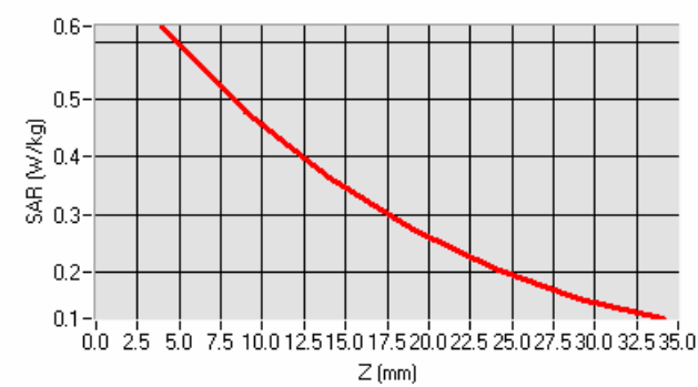
SAR, Z Axis Scan (X = -2, Y = 15)
