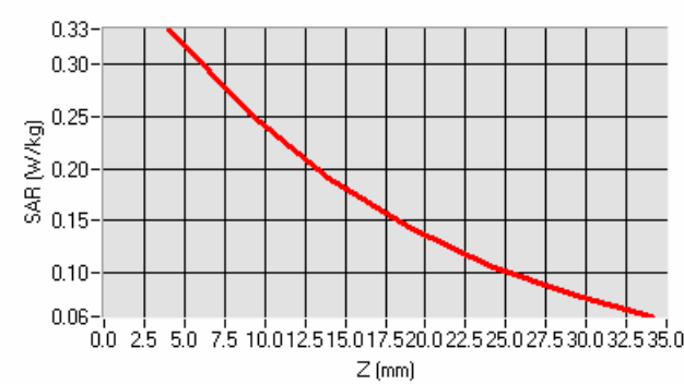
SAR, Z Axis Scan (X = -6, Y = 14)
