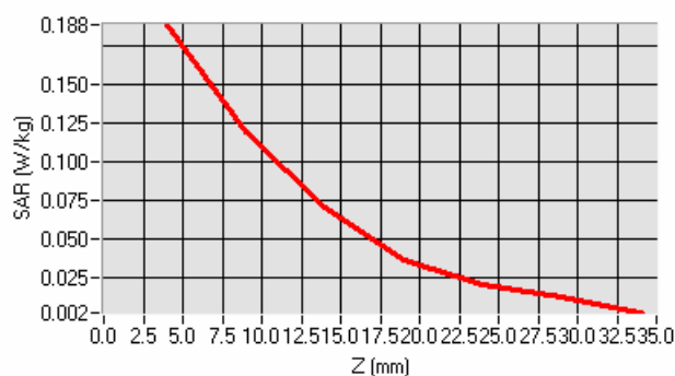
SAR, Z Axis Scan (X = 13, Y = 29)
