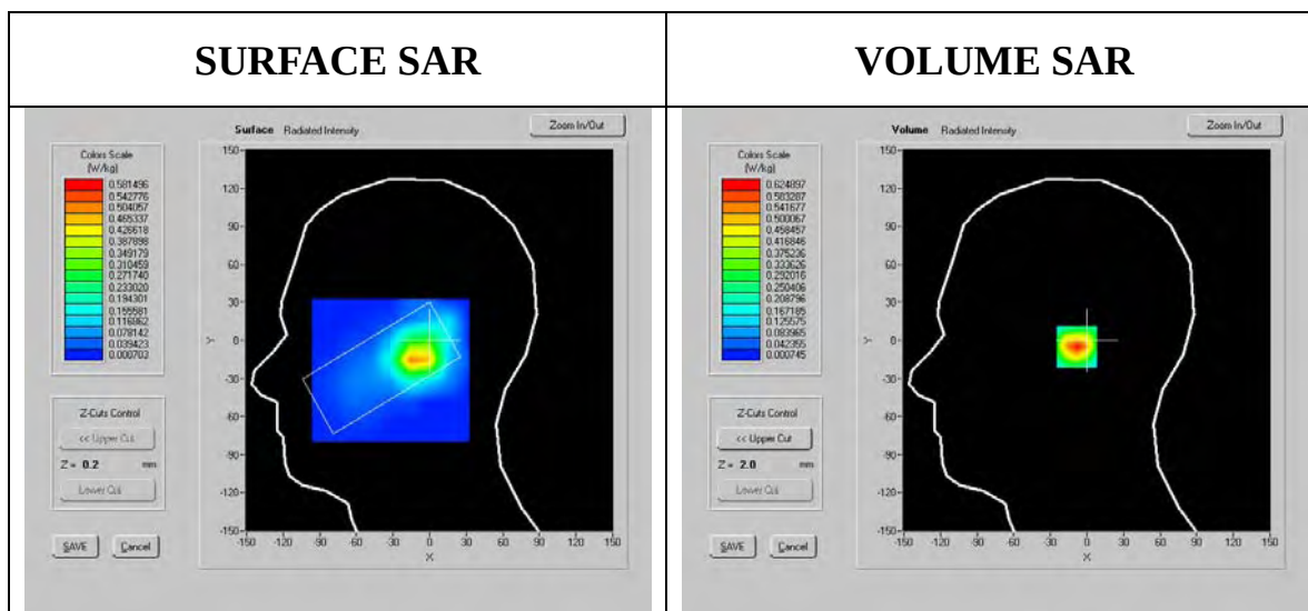
SAR, Z Axis Scan (X = -1, Y = -5)
