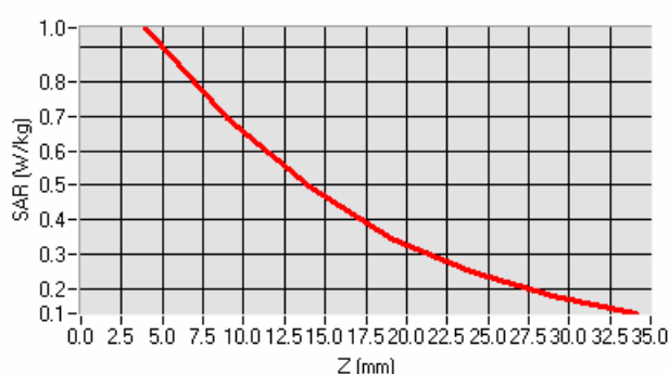
SAR, Z Axis Scan (X = -24, Y = -8)
