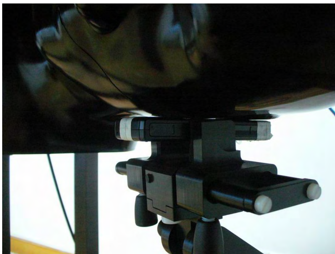
Figure B.4 EUT Left Head Touch Cheek Position
