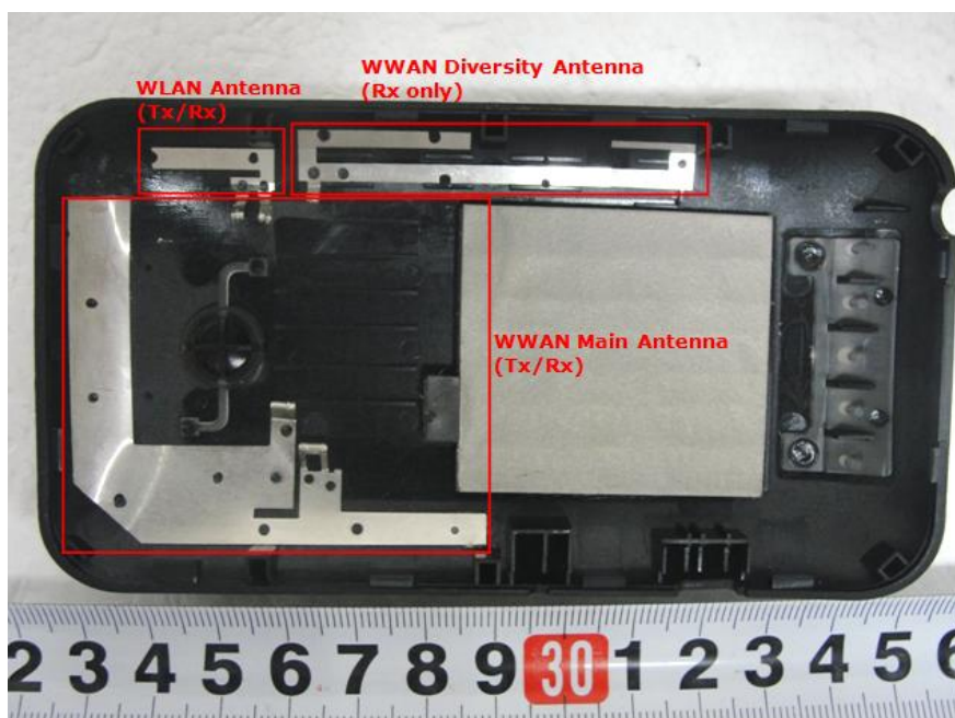
Antenna Location
