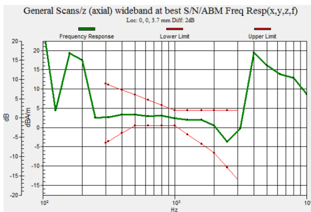
Fig 8.1 GSM850 Ch128
