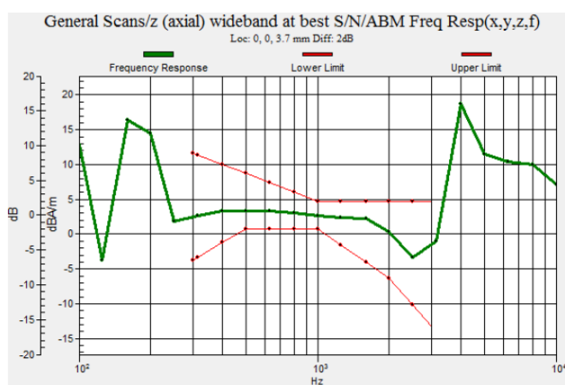
Fig 8.5 GSM1900 Ch661
