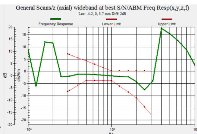
Fig 8.6 GSM1900 Ch810
