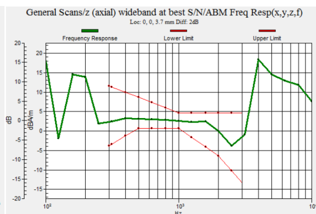
Fig 8.4 GSM1900 Ch512
