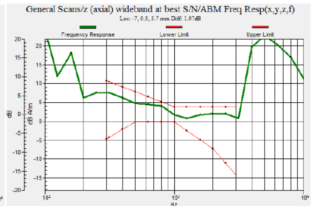
Fig 8.6 GSM1900 Ch810
