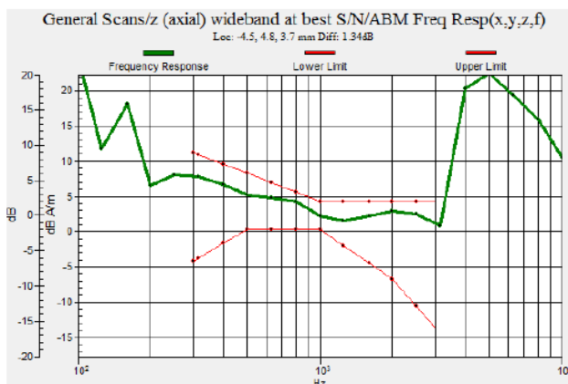
Fig 8.5 GSM1900 Ch661
