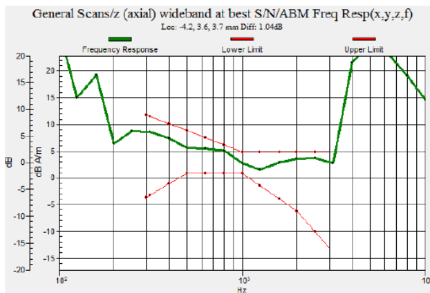
Fig 8.3 GSM850 Ch251
