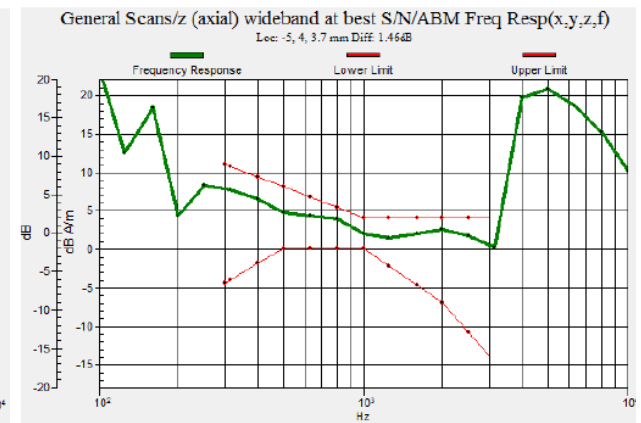
Fig 8.4 GSM1900 Ch512
