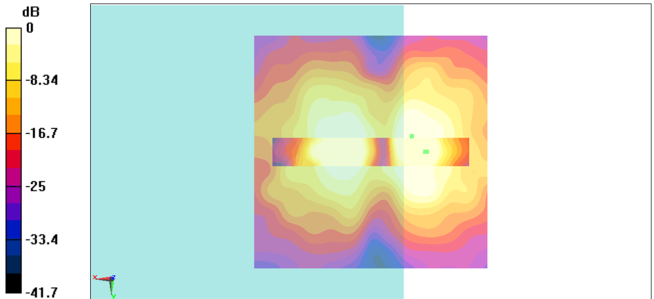
Fig B.10 T-Coil WCDMA 1900
