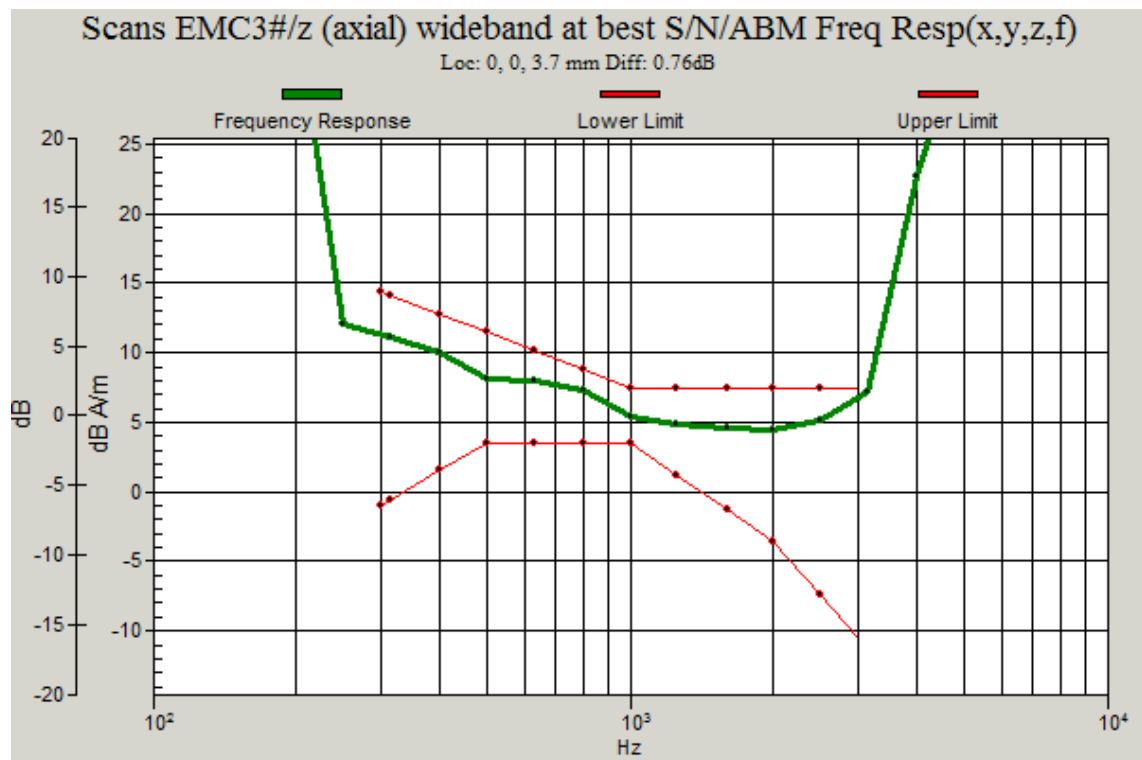
Figure C.3 Frequency Response of WCDMA 850
