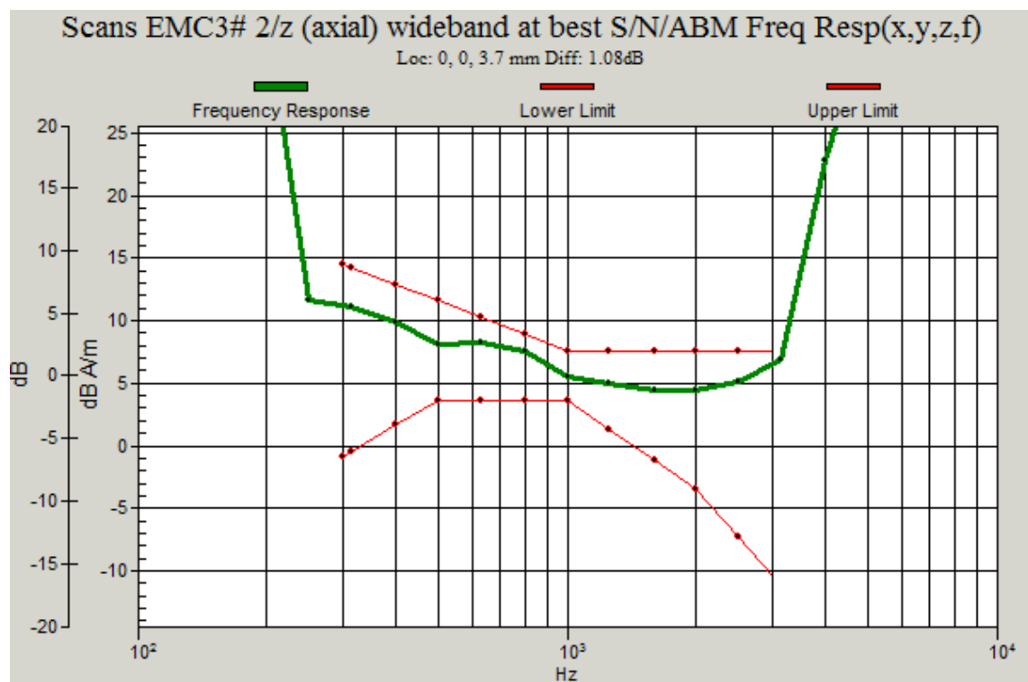
Figure C.4 Frequency Response of WCDMA 1900
