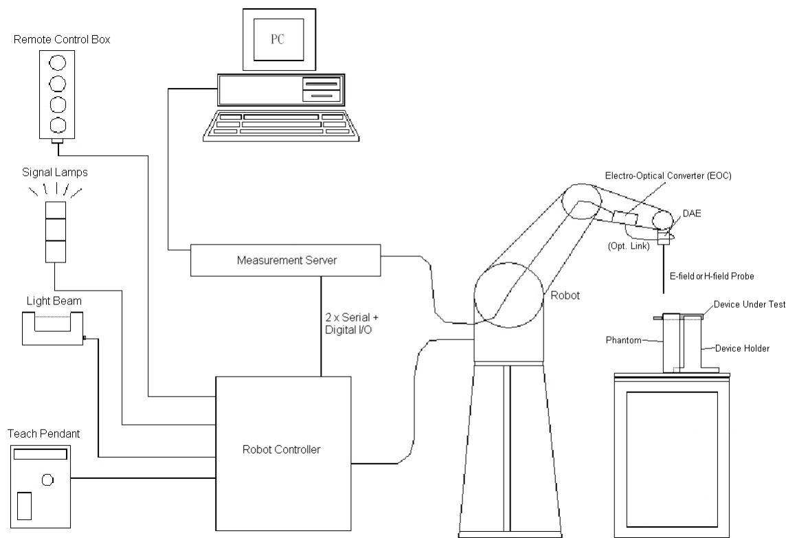
Fig 5.1 SPEAG DASY5 System Configurations
