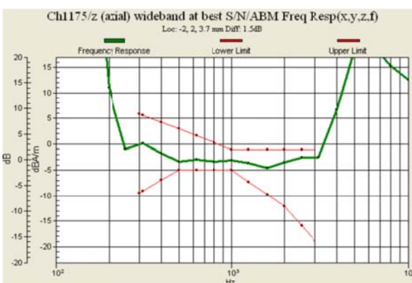
Fig 8.6 CDMA2000 BC1 Ch1175
