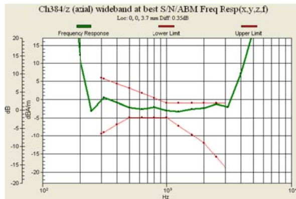
Fig 8.2 CDMA2000 BC0 Ch384
