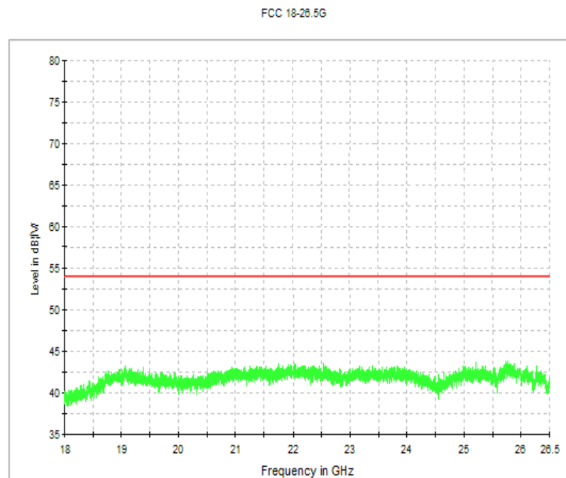
Fig.69. Radiated emission: GFSK, 18 GHz - 26 GHz
