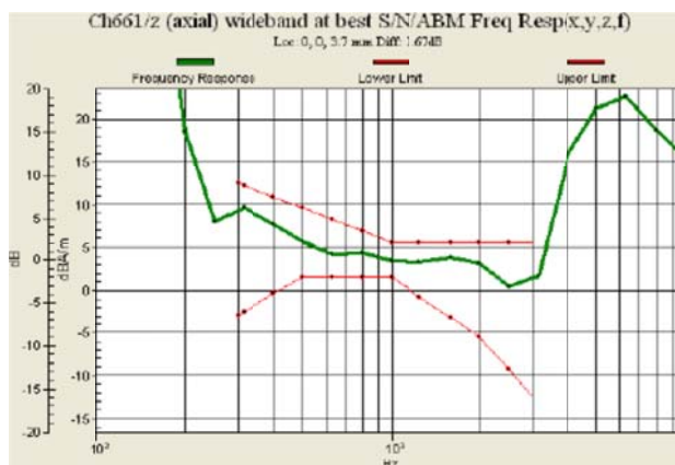
Fig 8.5 GSM1900 Ch661
