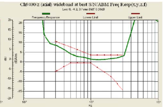
Fig. 8.14 WCDMA Band II Ch9400
