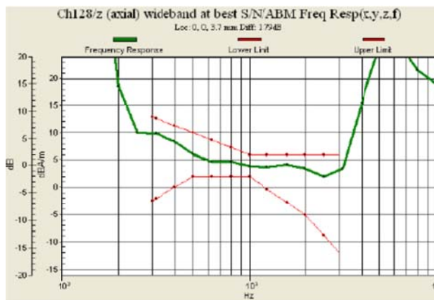
Fig 8.1 GSM850 Ch128
