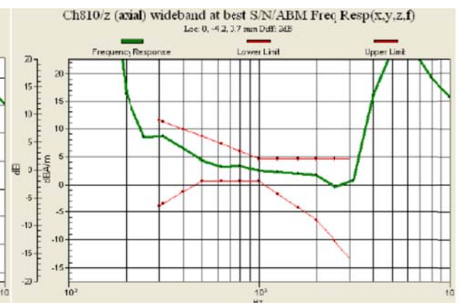
Fig 8.6 GSM1900 Ch810
