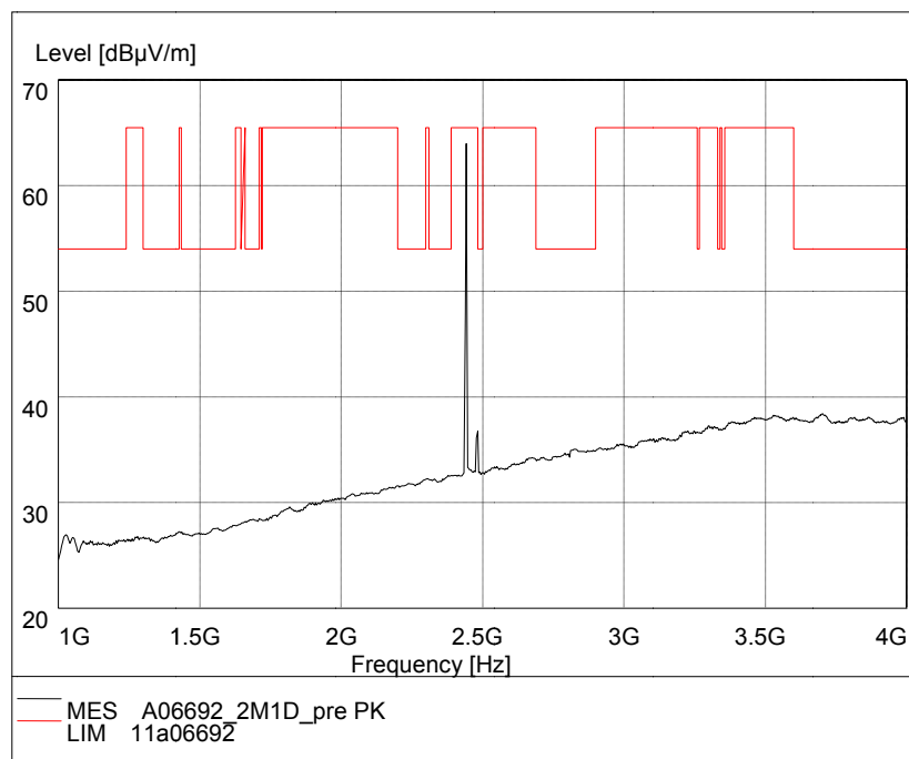
Fig.62. Radiated emission: GFSK, Channel 39, 1 GHz - 4 GHz
