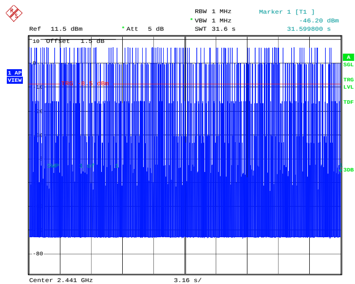
Fig.96. Time of occupancy (Dwell Time): Channel 39, Packet DH3
