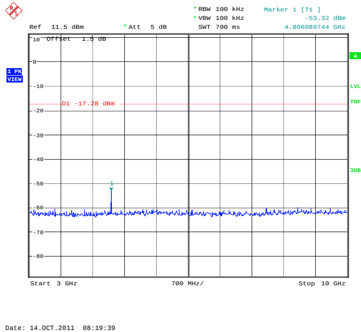
Fig.31. Conducted spurious emission: \pi/4 DQPSK, Channel 0, 3GHz - 10GHz
