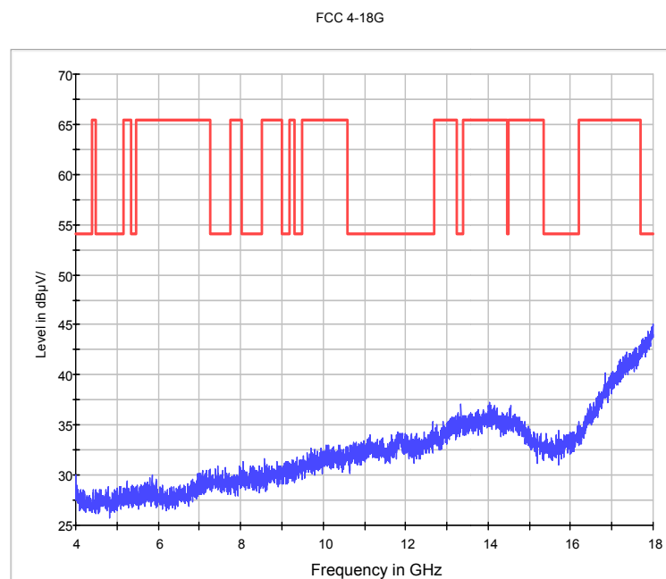
Fig.63. Radiated emission: GFSK, Channel 39, 4 GHz - 18 GHz
