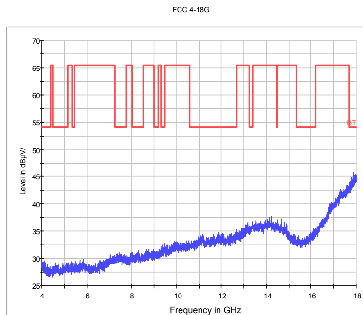
Fig.87. Radiated emission: 8DPSK, Channel 39, 4 GHz - 18 GHz
