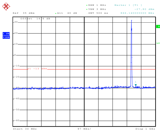
Conducted Emission Plot between 30MHz ~ 1GHz
