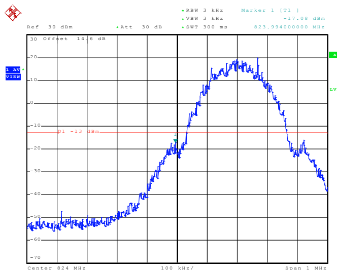
Lower Band Edge Plot on Channel 128
