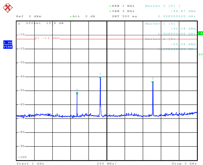
Conducted Emission Plot between 1GHz ~ 3GHz
