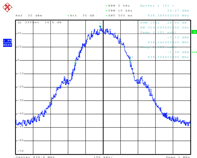
26dB Bandwidth Plot on Channel 189
