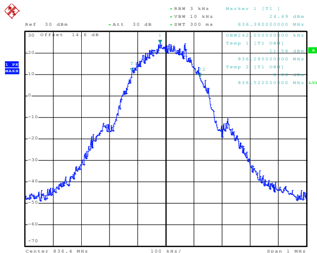
99% Occupied Bandwidth Plot on Channel 189
