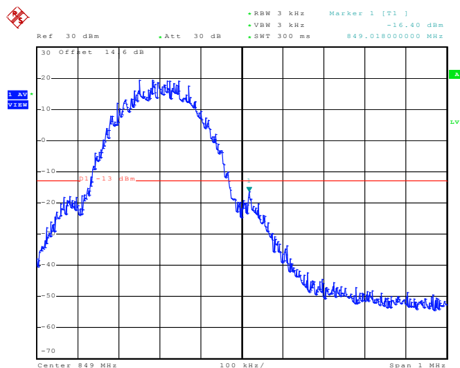
Higher Band Edge Plot on Channel 251
