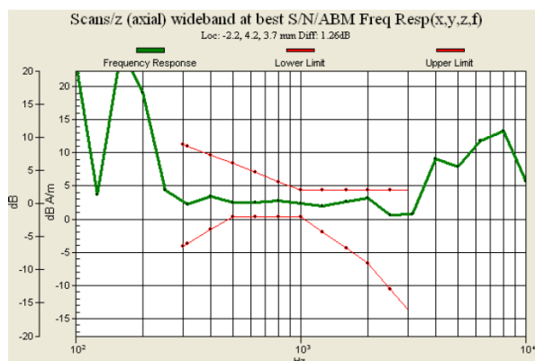
Fig. 9.5 GSM1900 Ch661
