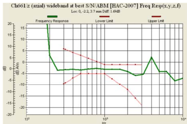
Fig. 9.5 GSM1900 Ch661
