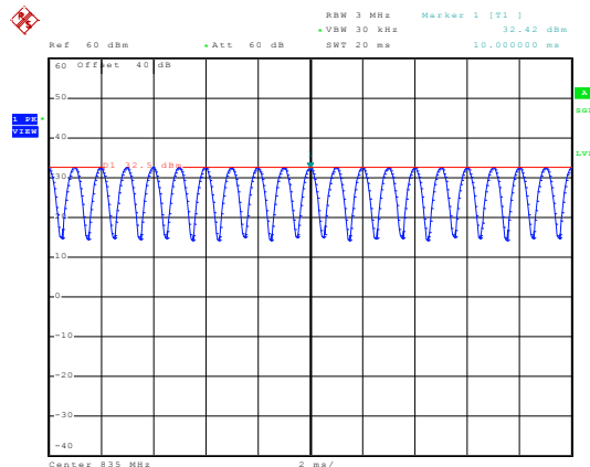
835MHz - 80% AM
