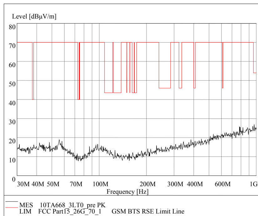
Fig.62 Radiated emission: 8DPSK, Channel 0, 30 MHz - 1 GHz
