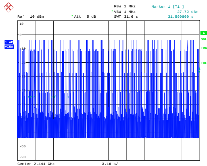
Fig.77 Time of occupancy (Dwell Time): Channel 39, Packet DH5
