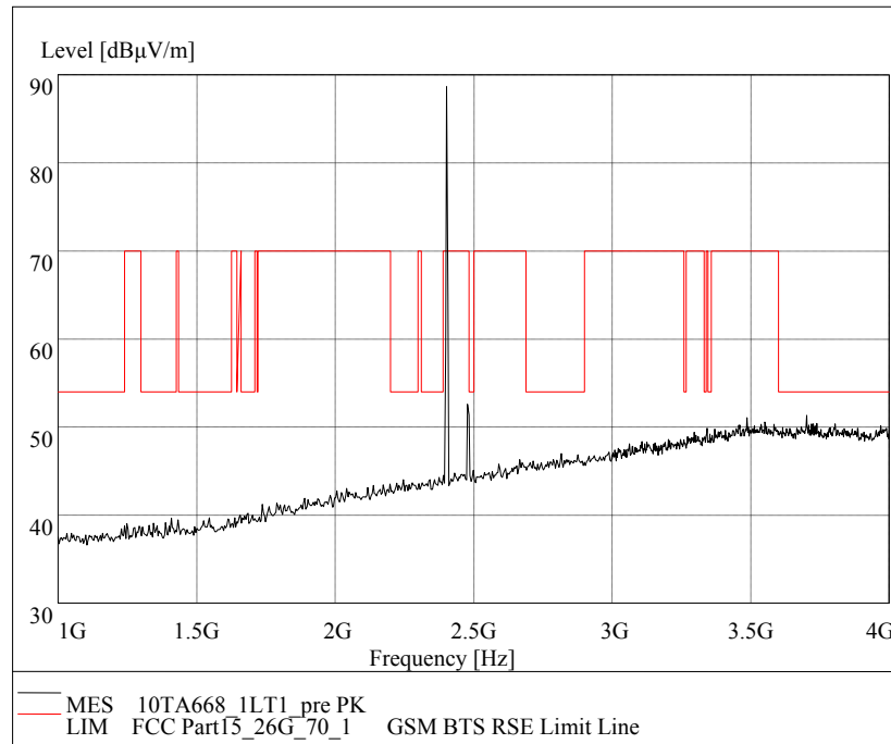
Fig.41 Radiated emission: GFSK, Channel 0, 1 GHz - 4 GHz
