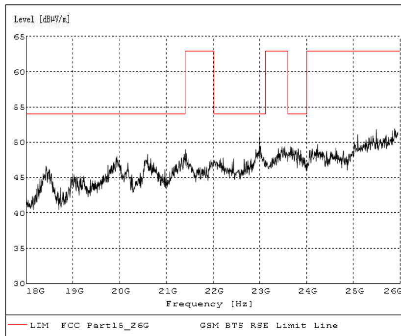
Fig.61 Radiated emission: \pi/4 DQPSK, 18 GHz - 26 GHz
