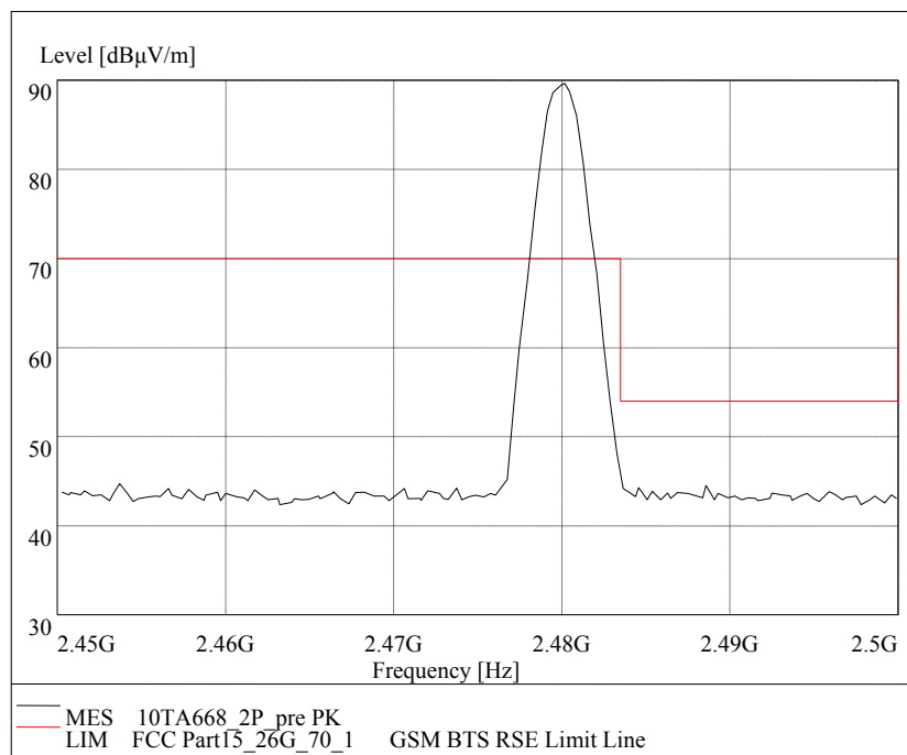
Fig.60 Radiated emission (Power): \pi/4 DQPSK
