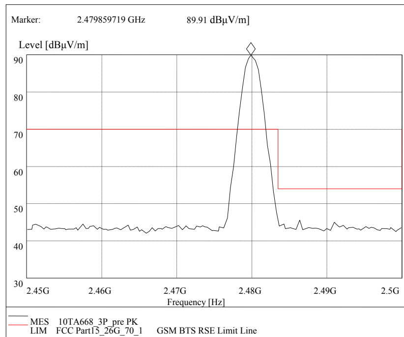
Fig.71 Radiated emission (Power): 8DPSK
