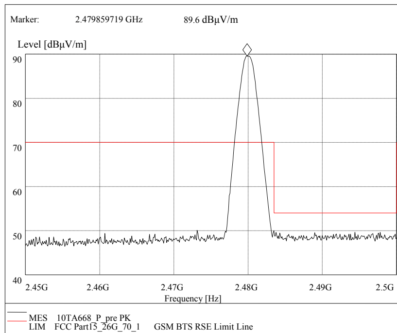
Fig.49 Radiated emission (Power): GFSK
