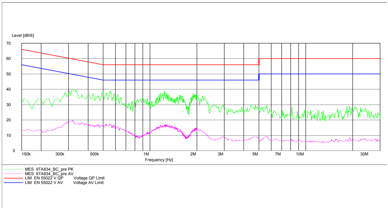
Fig. 109 AC Powerline Conducted Emission with charger
