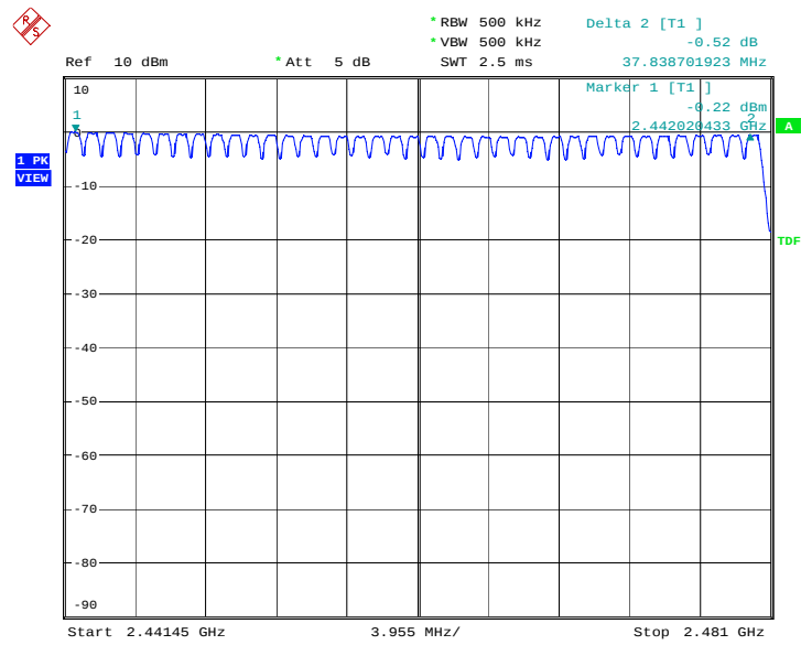
Fig. 103 Number of hopping frequencies: GFSK, Channel 0 - 39
