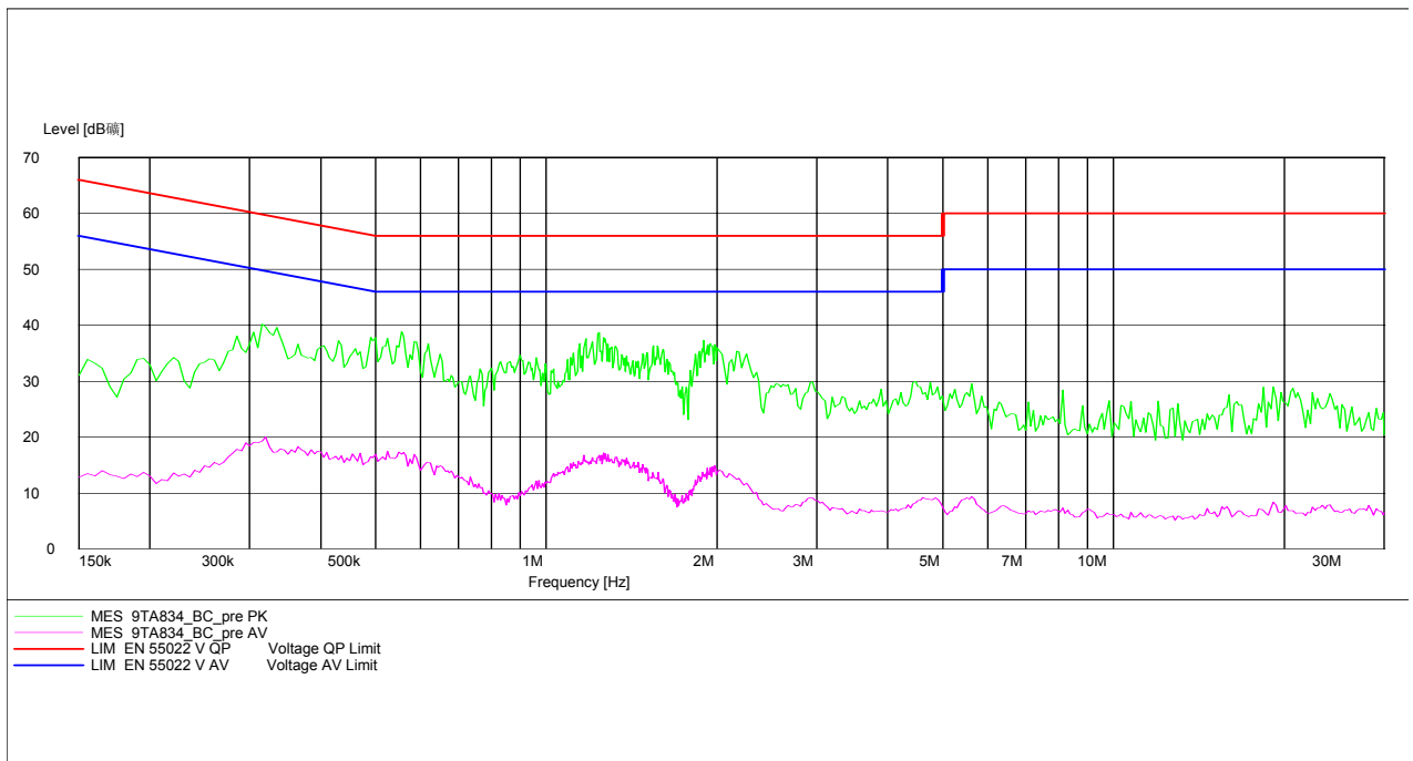
Fig. 109 AC Powerline Conducted Emission with charger
