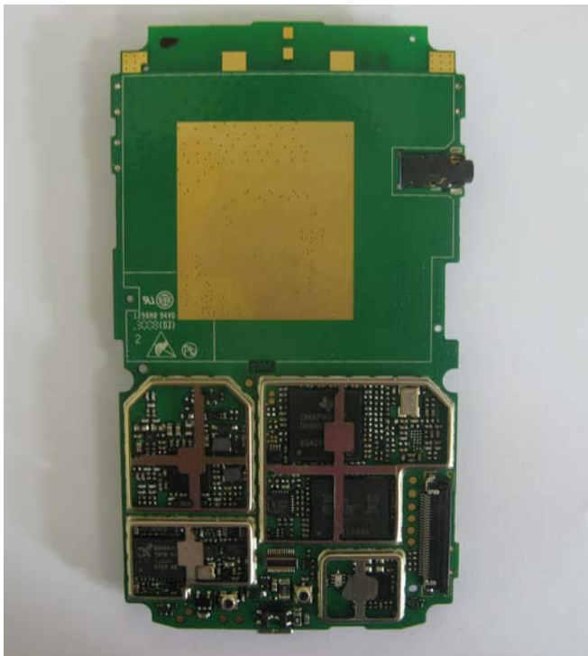
Picture 2: The top view of the PCB with the shielding cover removed
