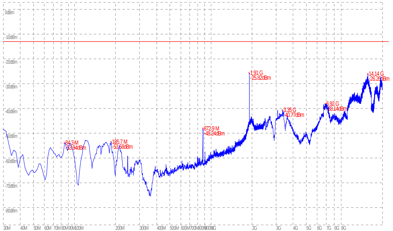
(Plot B.6: GSM 1900MHz Channel = 810, Test Antenna Vertical)
