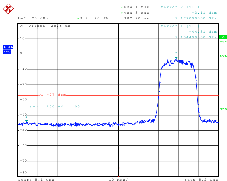
Low Band Edge Plot on Channel 36
