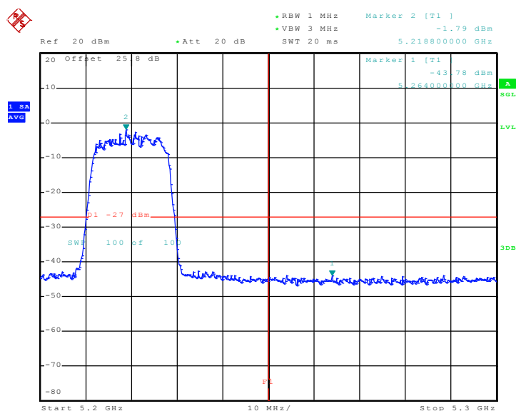
High Band Edge Plot on Channel 44
