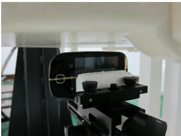
Left Side of DUT with Phantom 1 cm Gap
