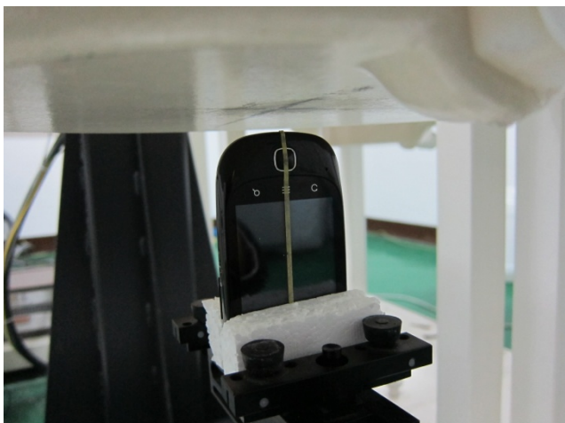
Bottom Side of DUT with Phantom 1 cm Gap
