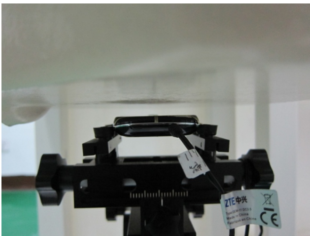
Front of DUT with Earphone to Phantom 1 cm Gap
