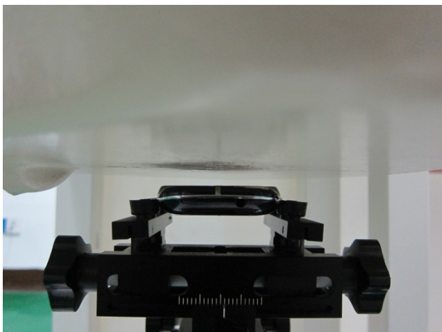
Front of DUT with Phantom 1 cm Gap
