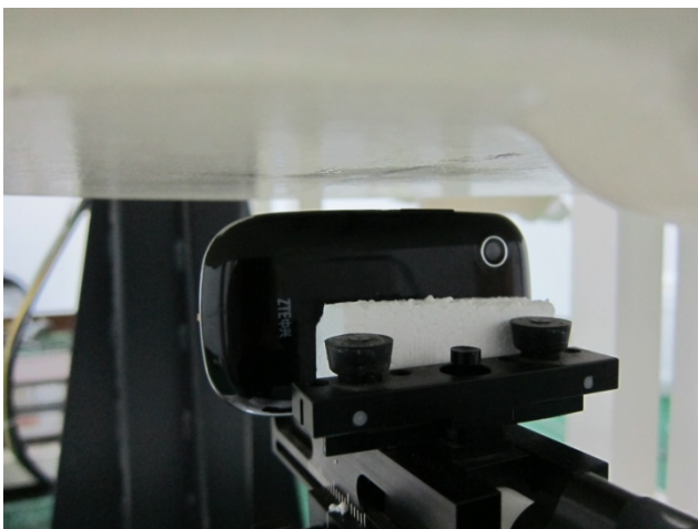
Right Side of DUT with Phantom 1 cm Gap
