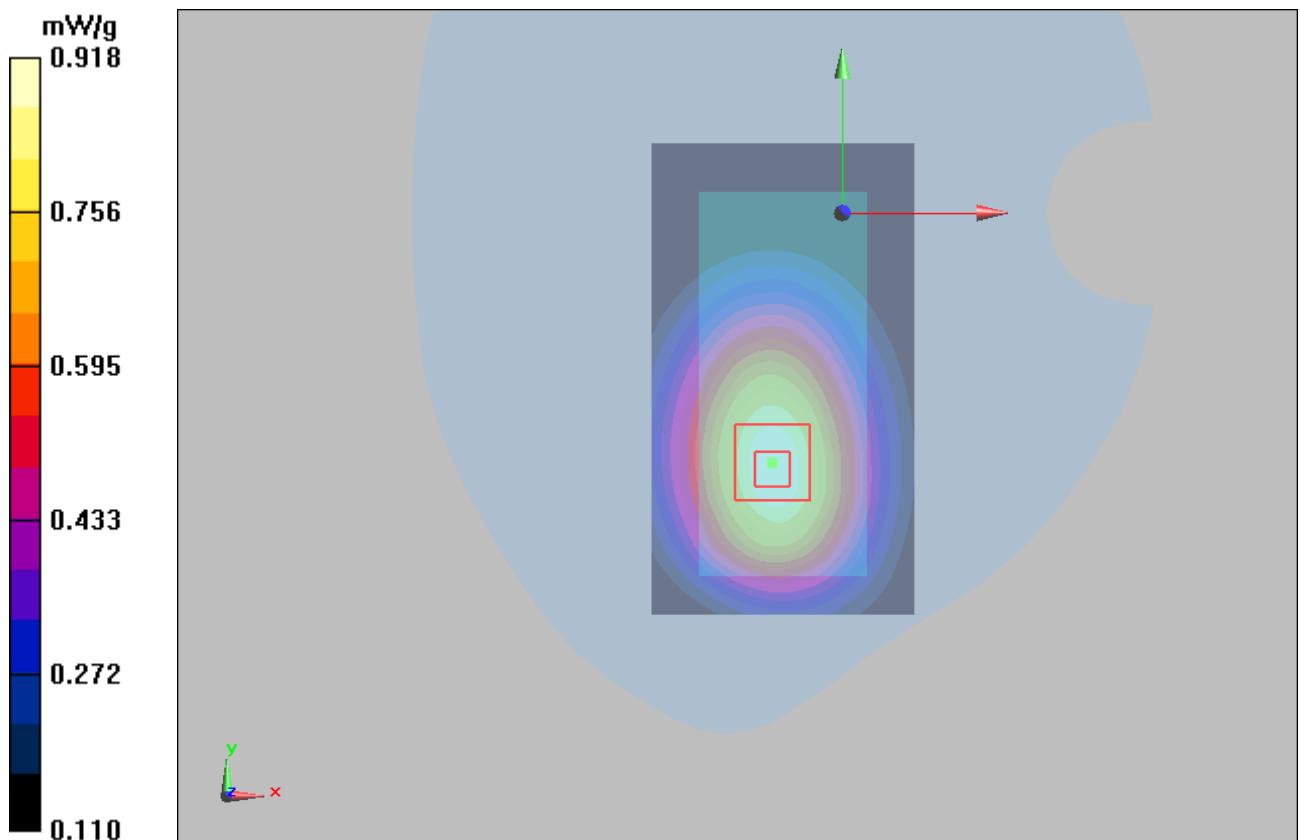
Figure 22 Body, Towards Phantom, GSM 850 GPRS (3Up) Channel 190
