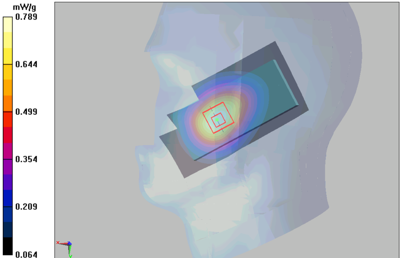
Figure 64 Right Hand Touch Cheek WCDMA Band V Channel 4183
