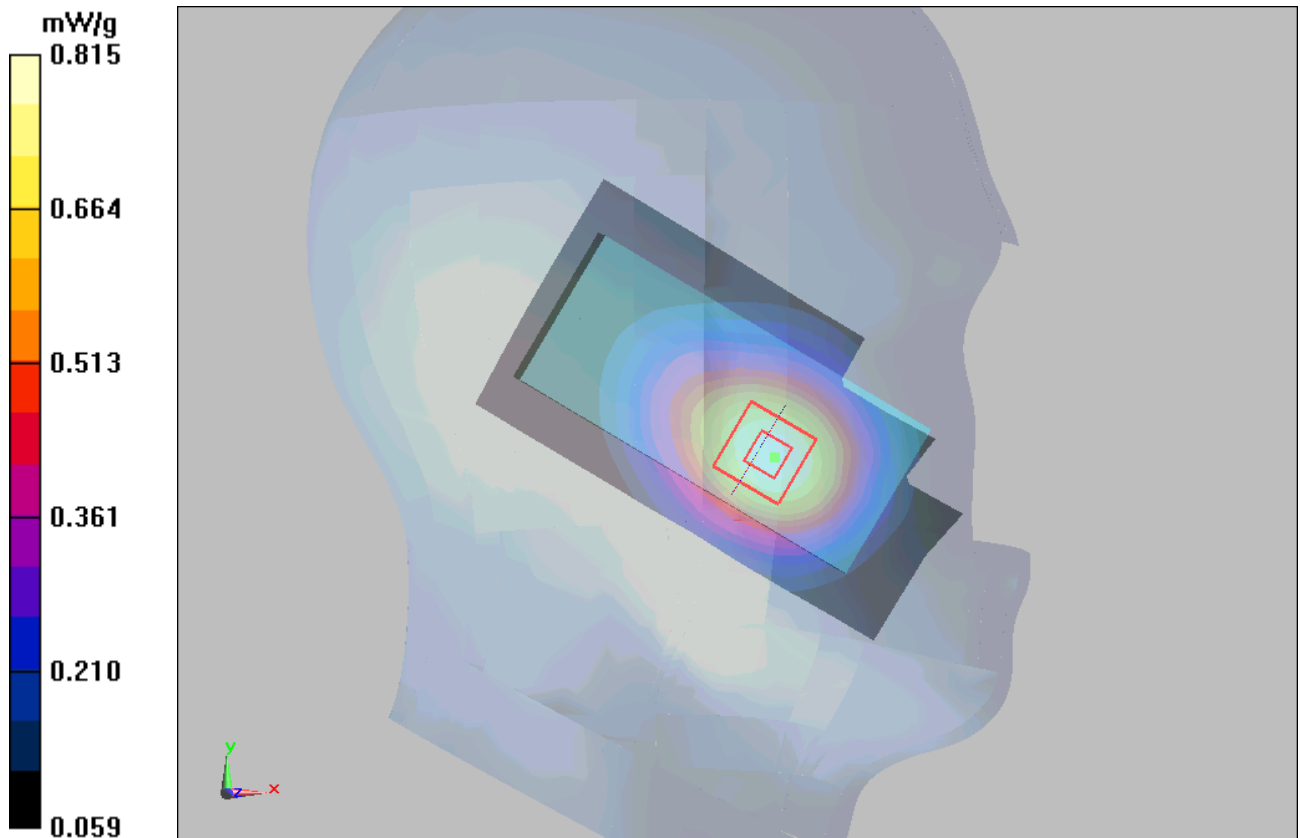
Figure 61 Left Hand Touch Cheek WCDMA Band V Channel 4183
