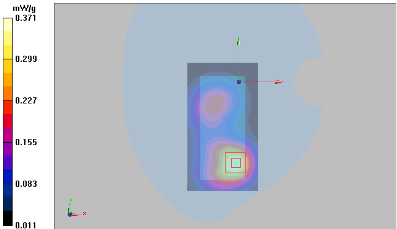
Figure 55 Body, Towards Phantom, WCDMA Band II Channel 9400
