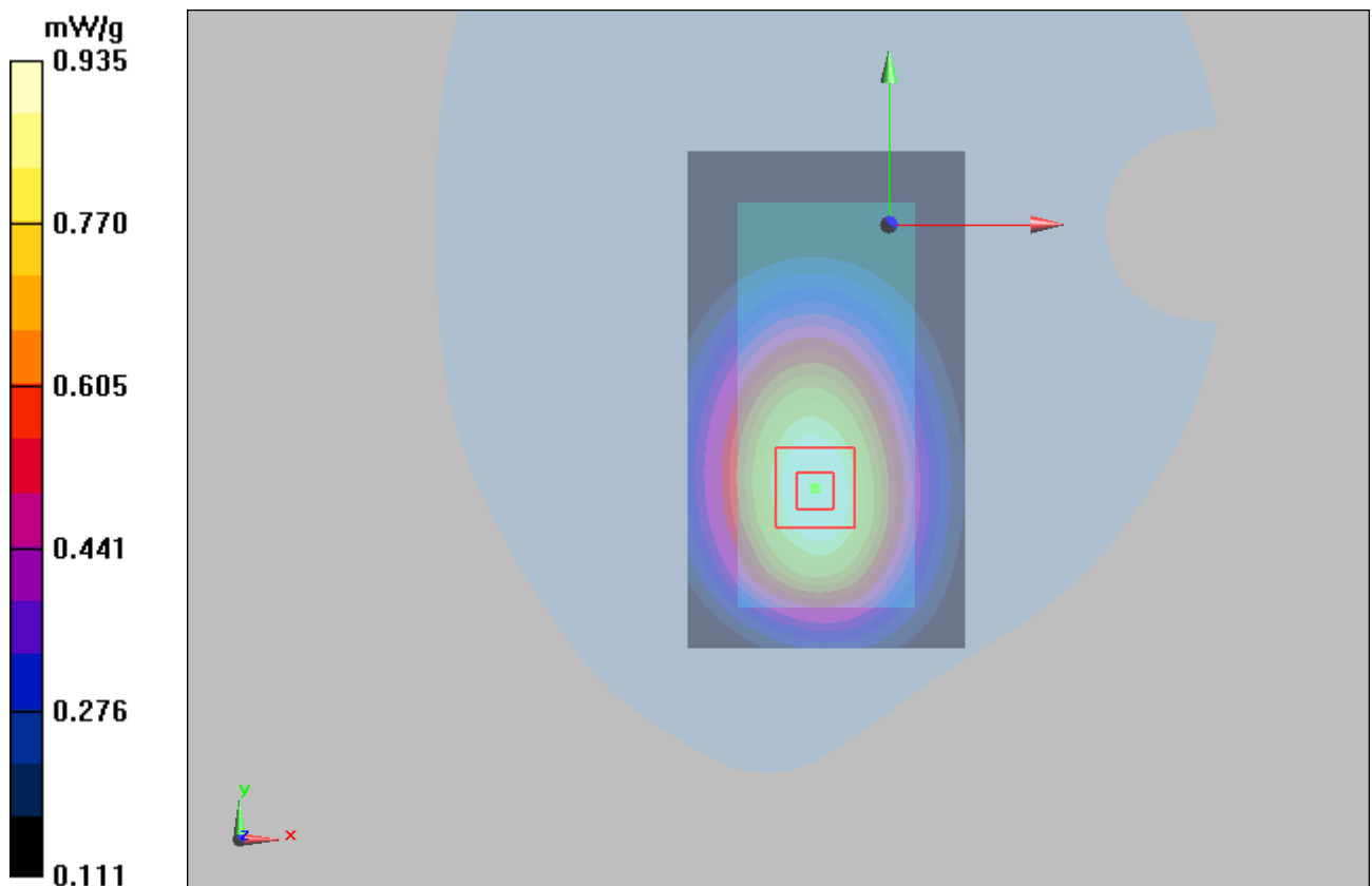
Figure 23 Body, Towards Phantom, GSM 850 GPRS (3Up) Channel 128
