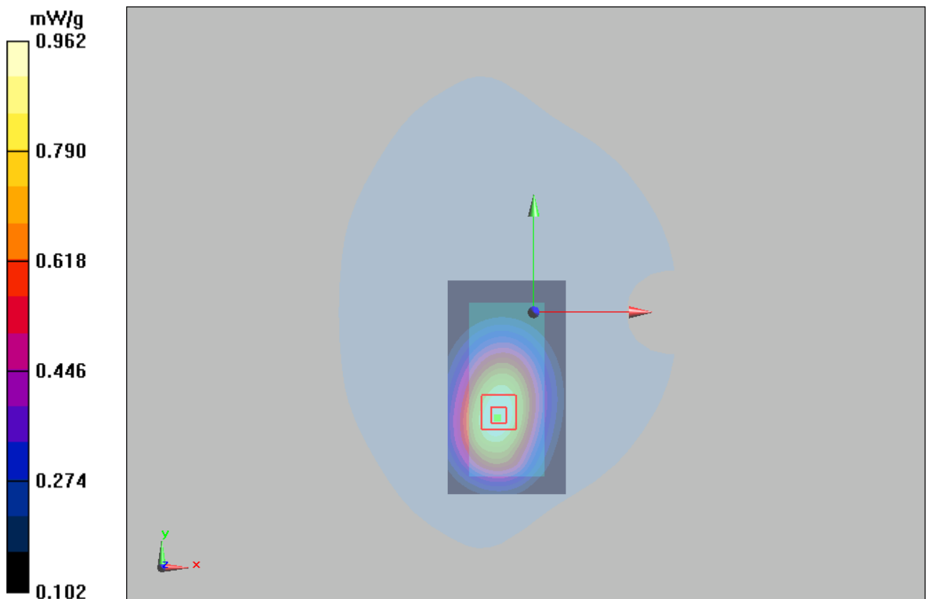
Figure 28 Body, Towards Ground, GSM 850 GPRS (4Up) Channel 190
