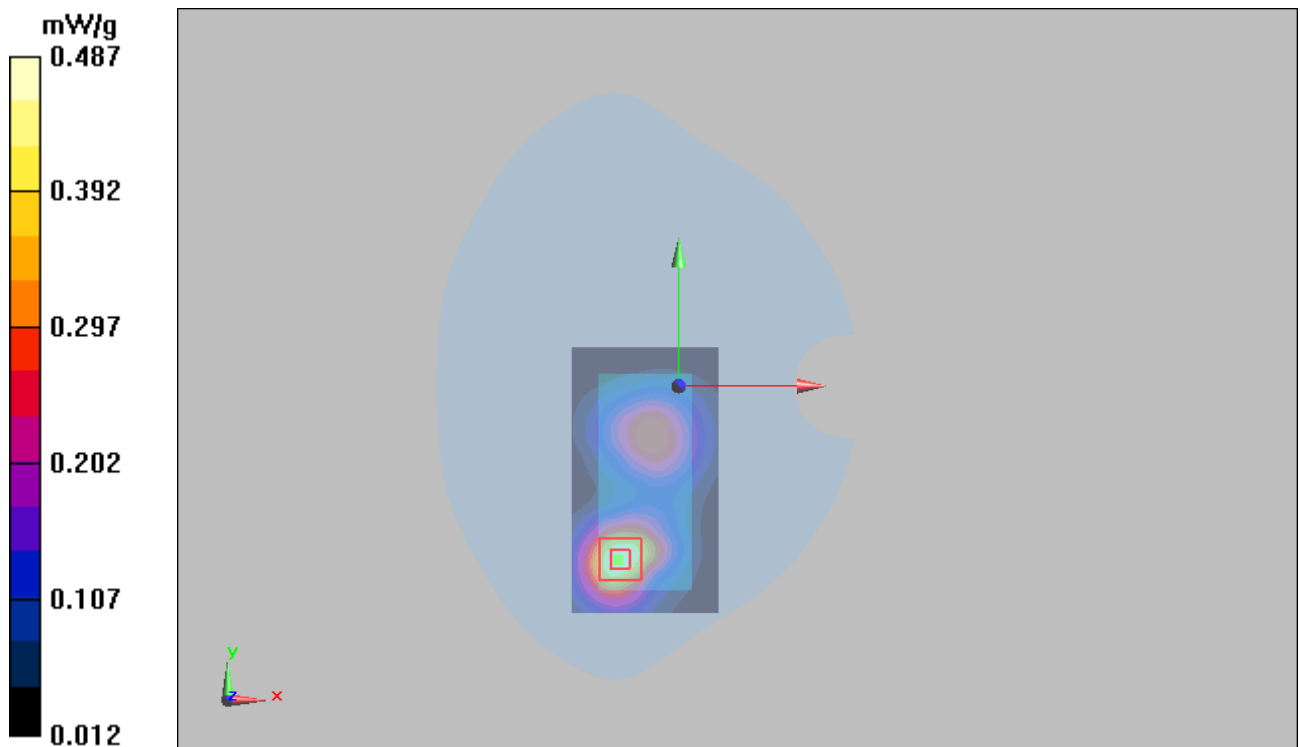
Figure 59 Body with Earphone, Towards Ground, WCDMA Band II Channel 9262
