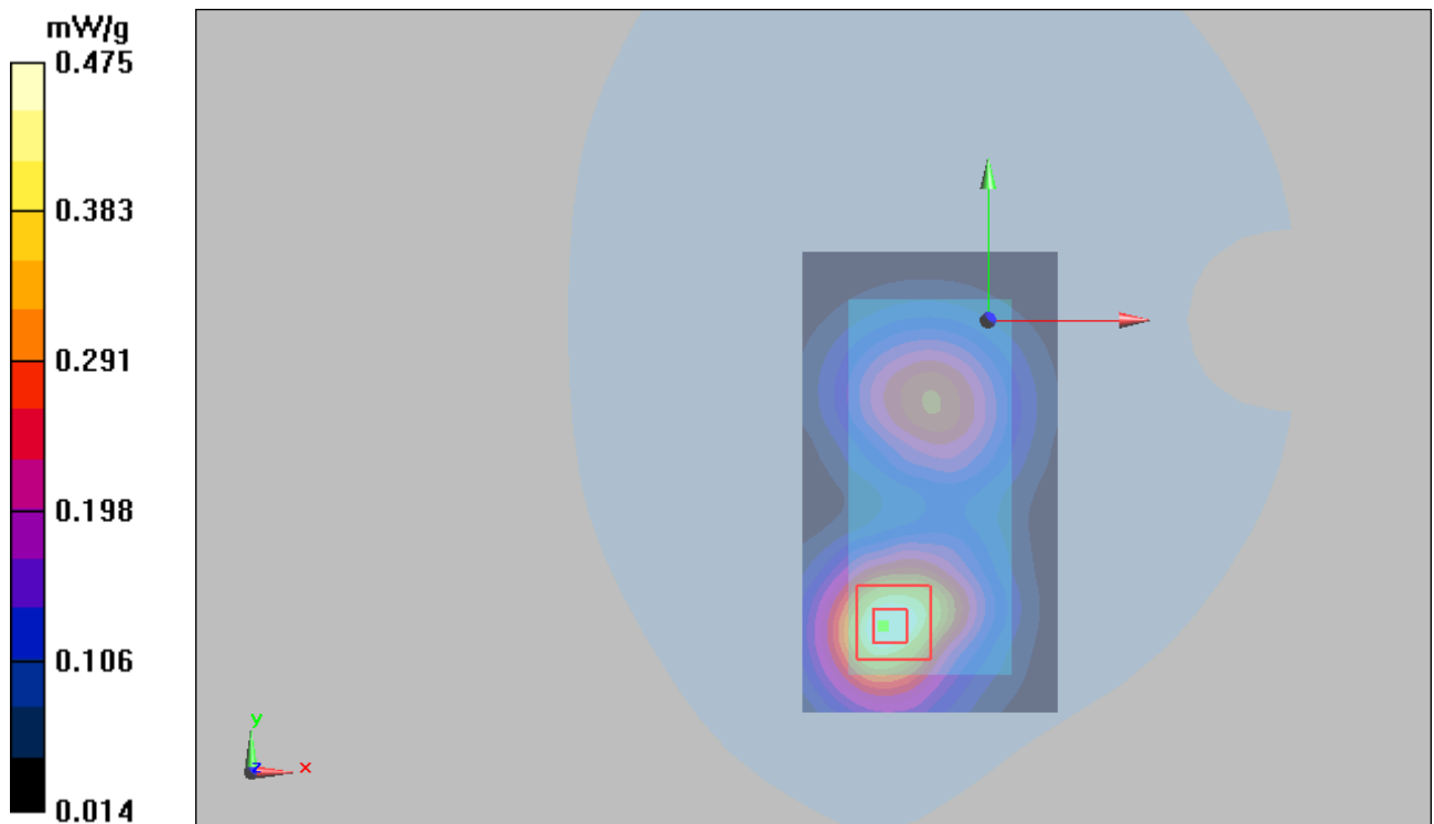
Figure 57 Body, Towards Ground, WCDMA Band II Channel 9400
