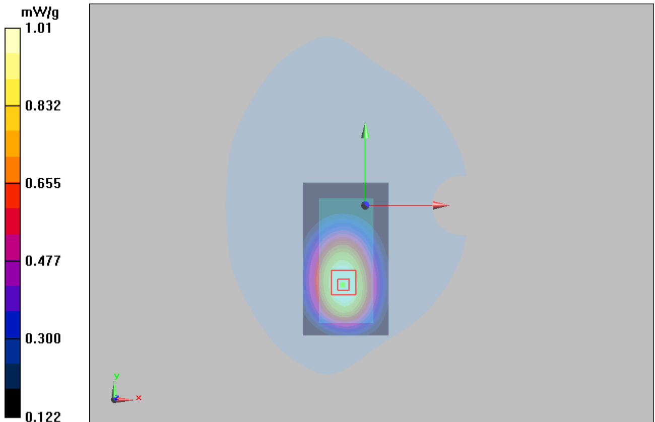
Figure 25 Body, Towards Phantom, GSM 850 GPRS (4Up) Channel 190
