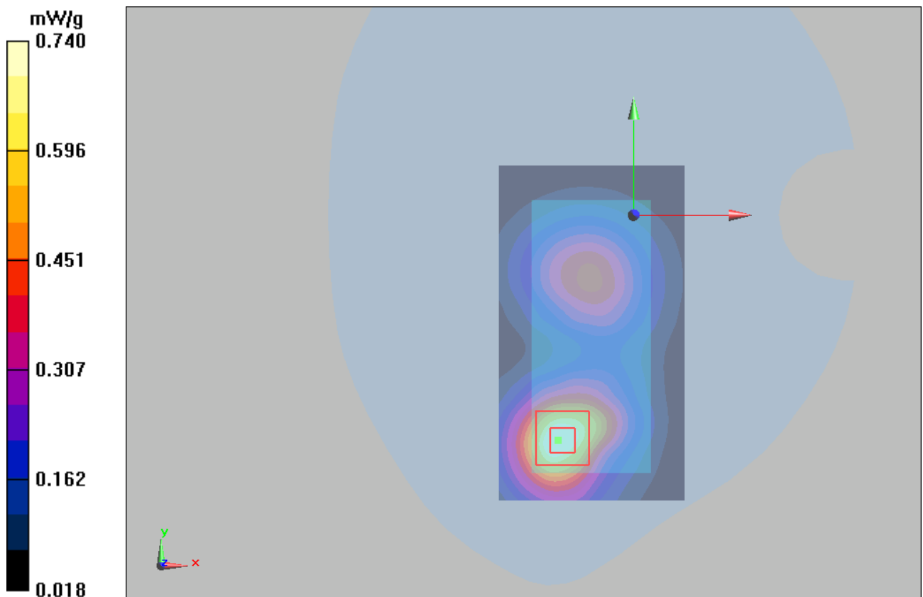
Figure 45 Body, Towards Ground, GSM 1900 GPRS (4Up) Channel 512
