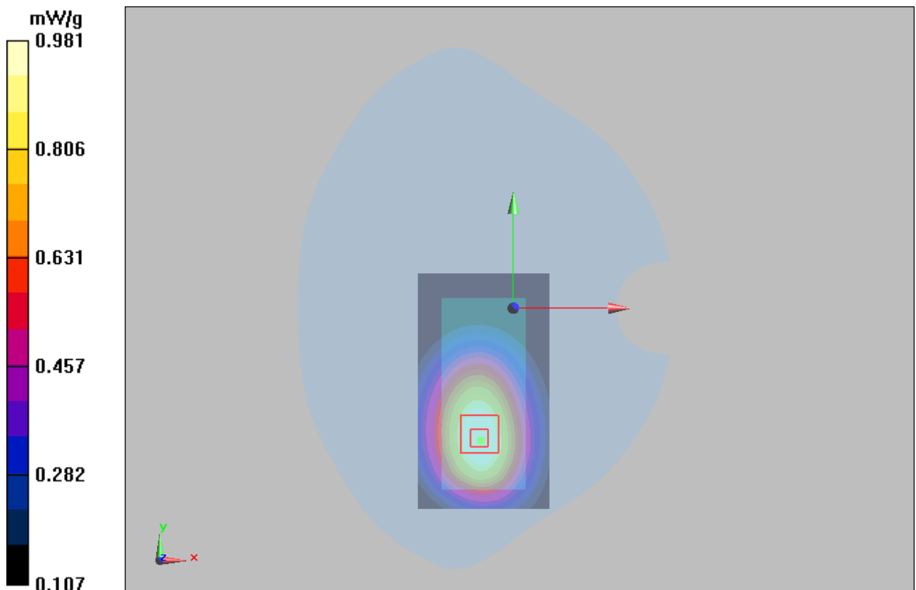
Figure 26 Body, Towards Phantom, GSM 850 GPRS (4Up) Channel 128
