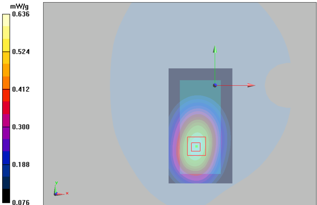
Figure 70 Body with Earphone, Towards Ground, WCDMA Band V Channel 4233
