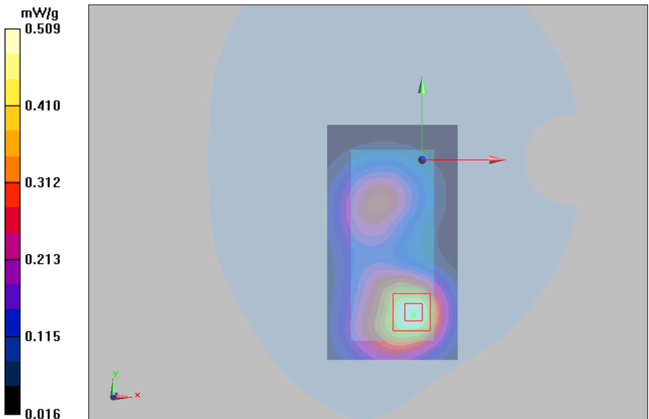
Figure 40 Body, Towards Phantom, GSM 1900 GPRS (2Up) Channel 661
