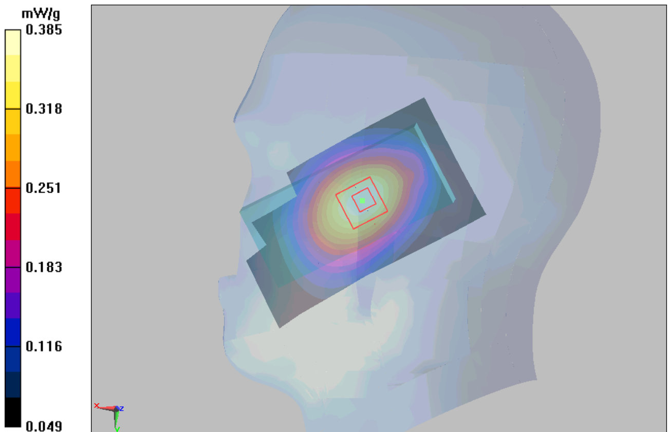
Figure 65 Right Hand Tilt 15° WCDMA Band V Channel 4183
