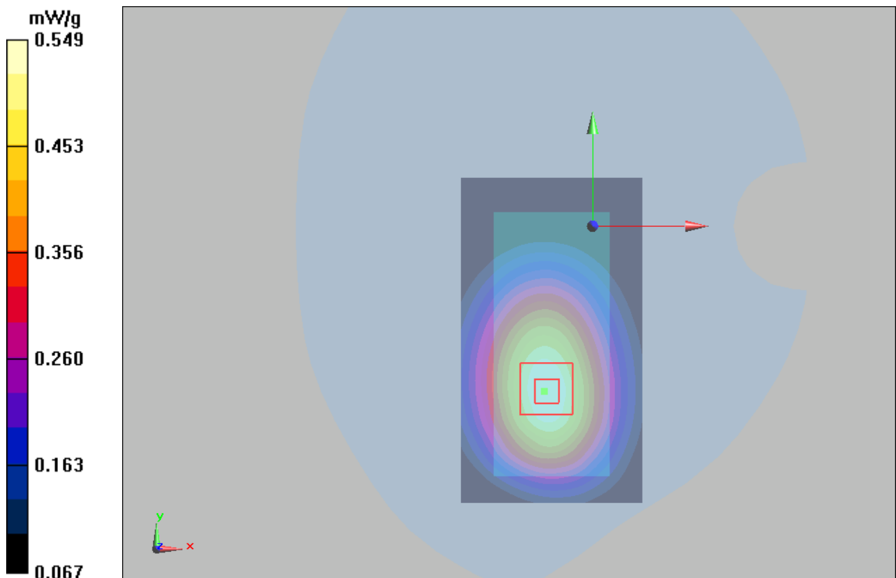
Figure 66 Body, Towards Phantom, WCDMA Band V Channel 4183
