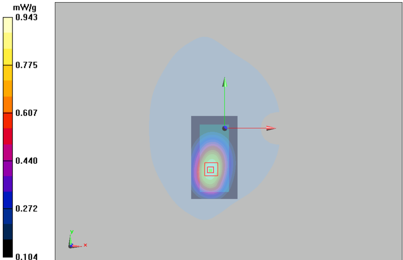
Figure 29 Body, Towards Ground, GSM 850 GPRS (4Up) Channel 128
