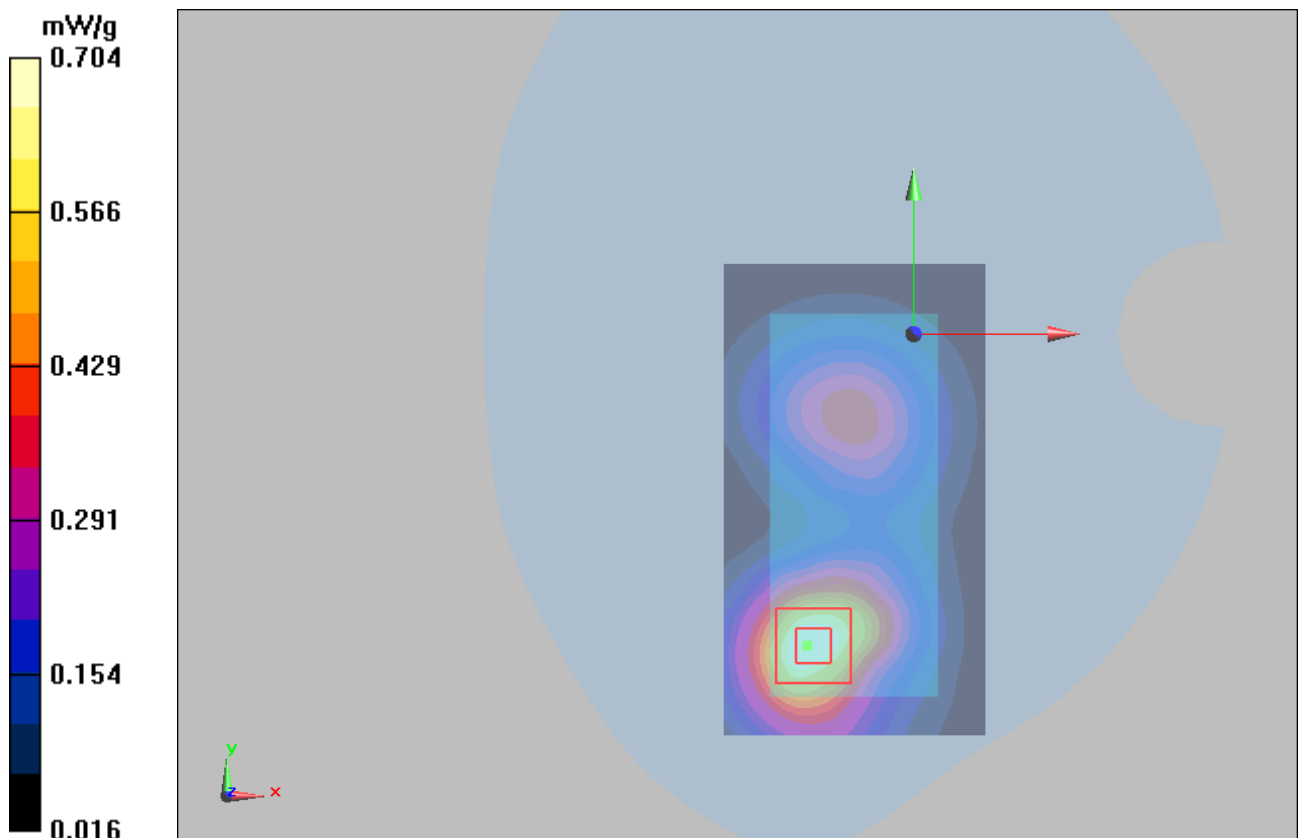
Figure 43 Body, Towards Ground, GSM 1900 GPRS (4Up) Channel 810
