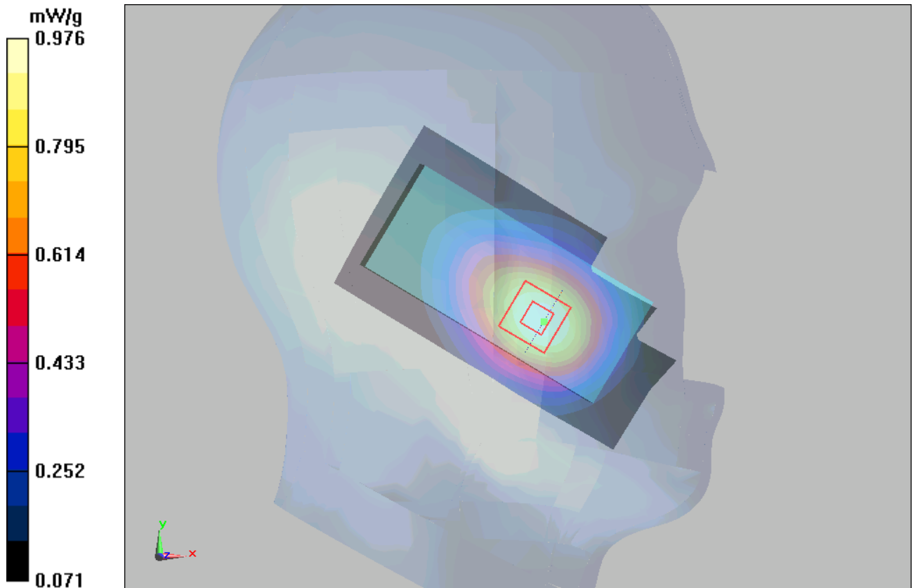
Figure 62 Left Hand Touch Cheek WCDMA Band V Channel 4132
