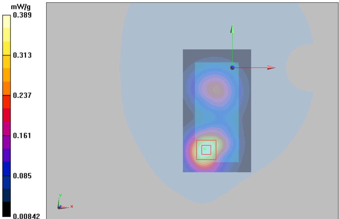
Figure 46 Body with Earphone, Towards Ground, GSM 1900 Channel 661
