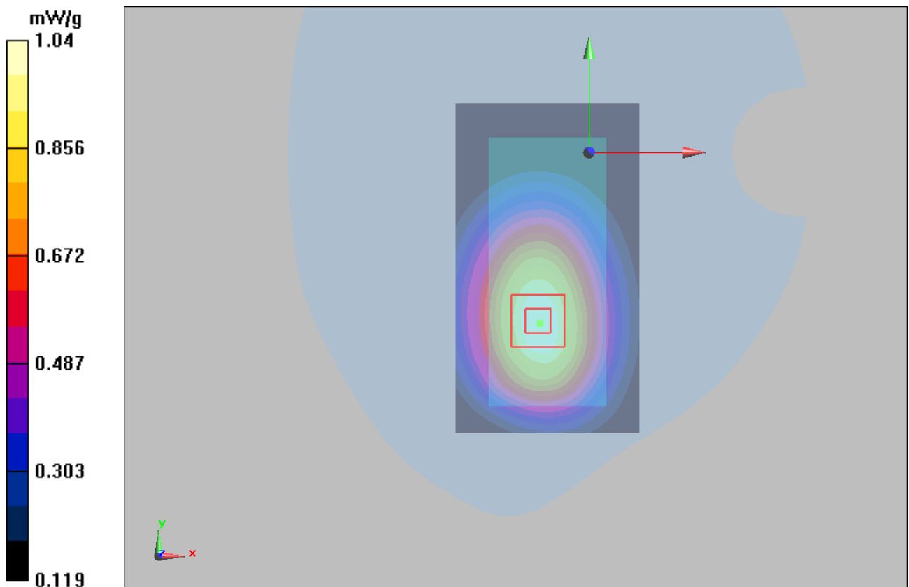
Figure 21 Body, Towards Phantom, GSM 850 GPRS (3Up) Channel 251
