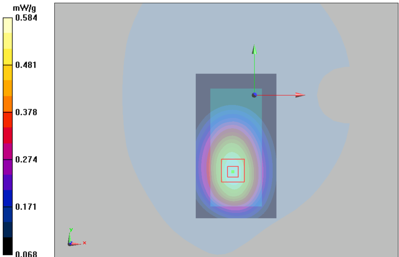
Figure 19 Body, Towards Phantom, GSM 850 Channel 190
