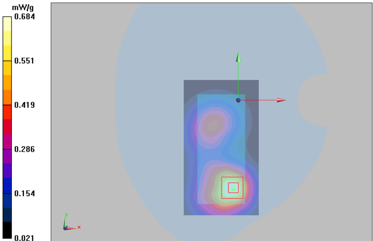
Figure 42 Body, Towards Phantom, GSM 1900 GPRS (4Up) Channel 661
