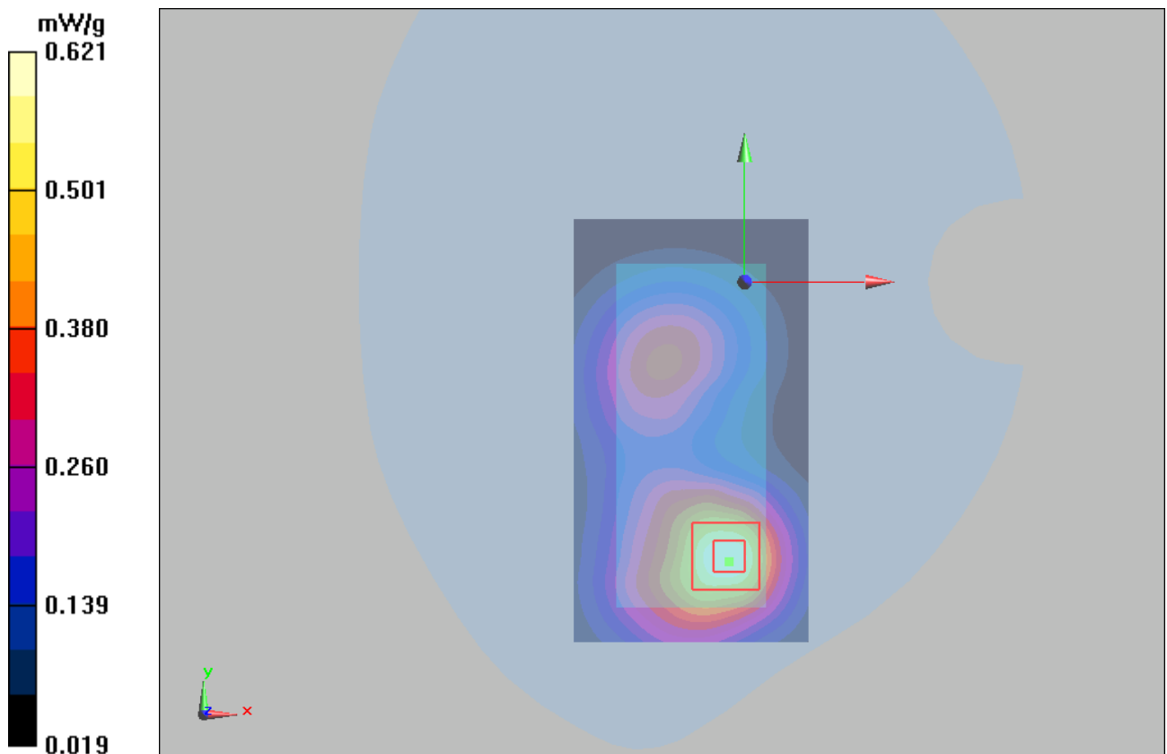
Figure 41 Body, Towards Phantom, GSM 1900 GPRS (3Up) Channel 661
