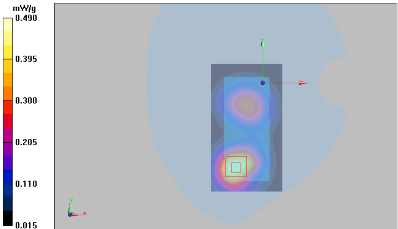
Figure 56 Body, Towards Ground, WCDMA Band II Channel 9538
