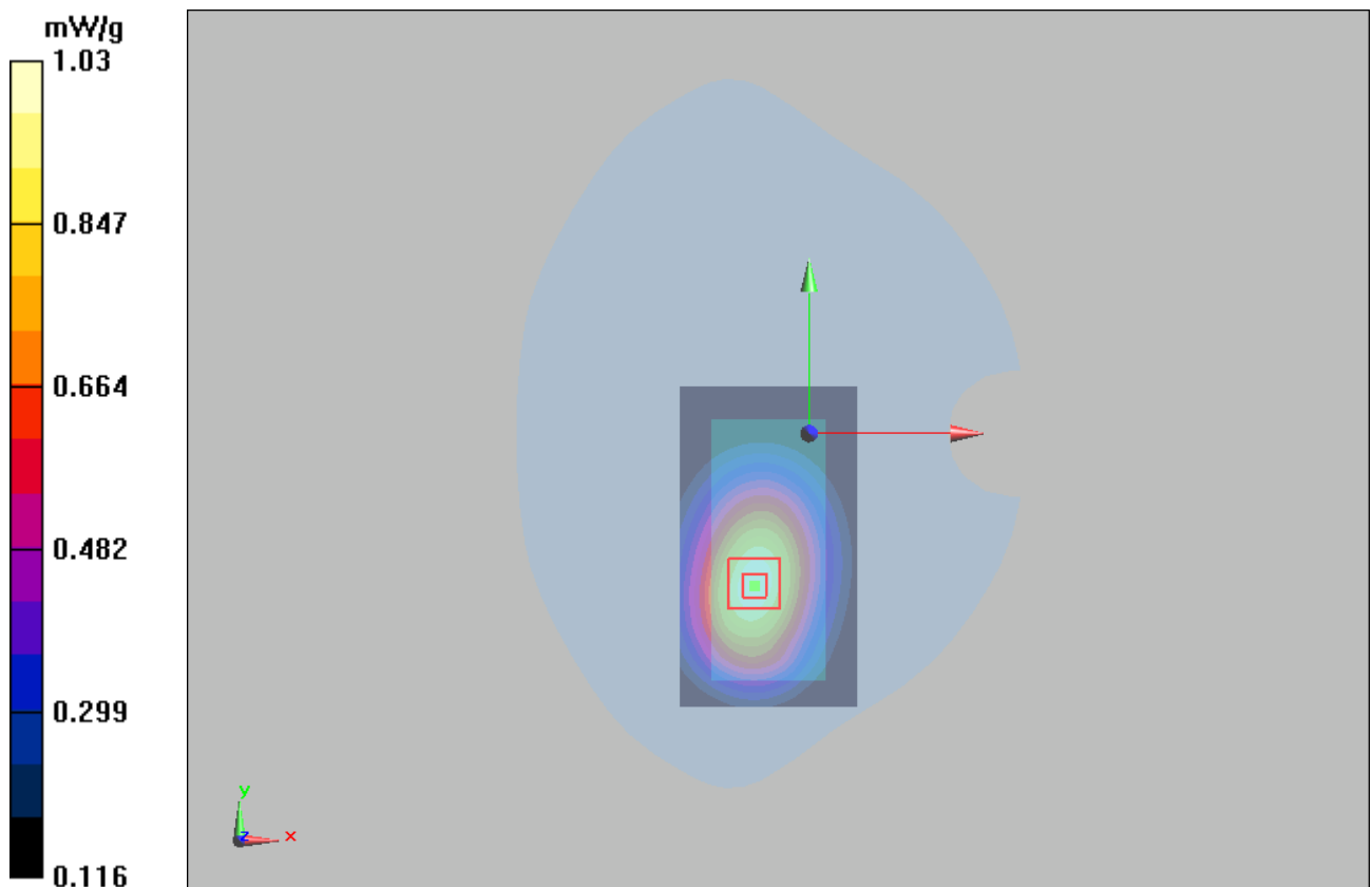
Figure 27 Body, Towards Ground, GSM 850 GPRS (4Up) Channel 251
