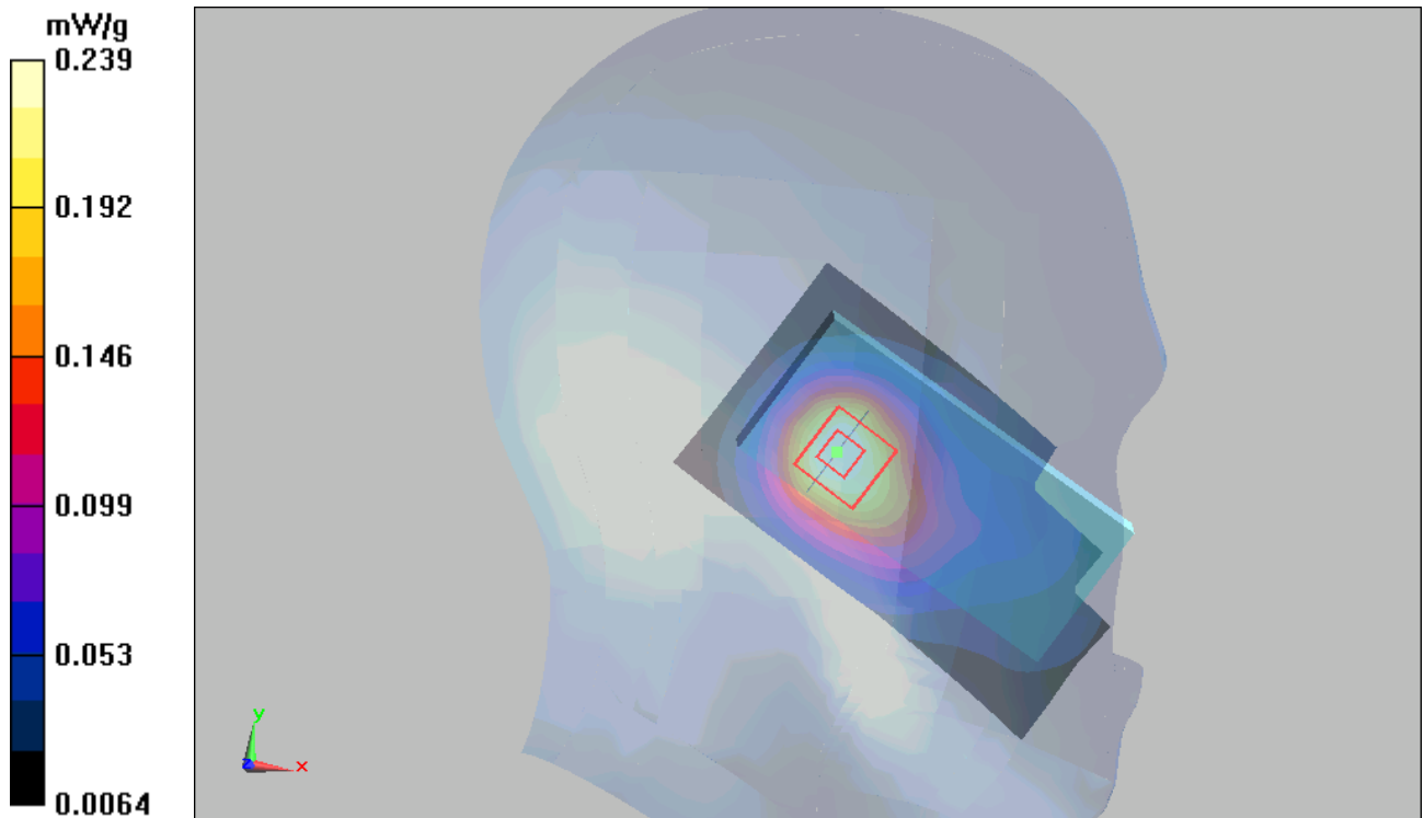
Figure 50 Left Hand Tilt 15° WCDMA Band II Channel 9400
