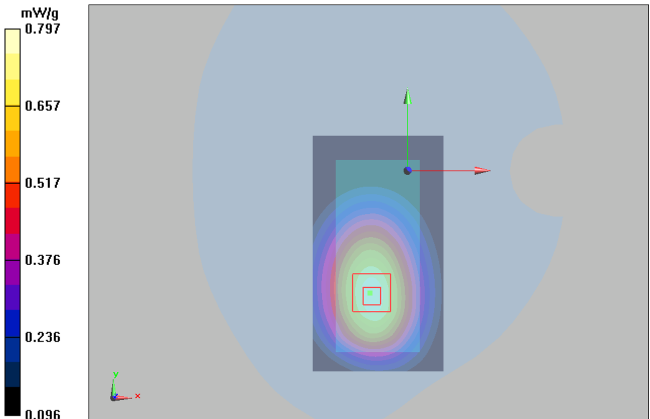
Figure 20 Body, Towards Phantom, GSM 850 GPRS (2Up) Channel 190
