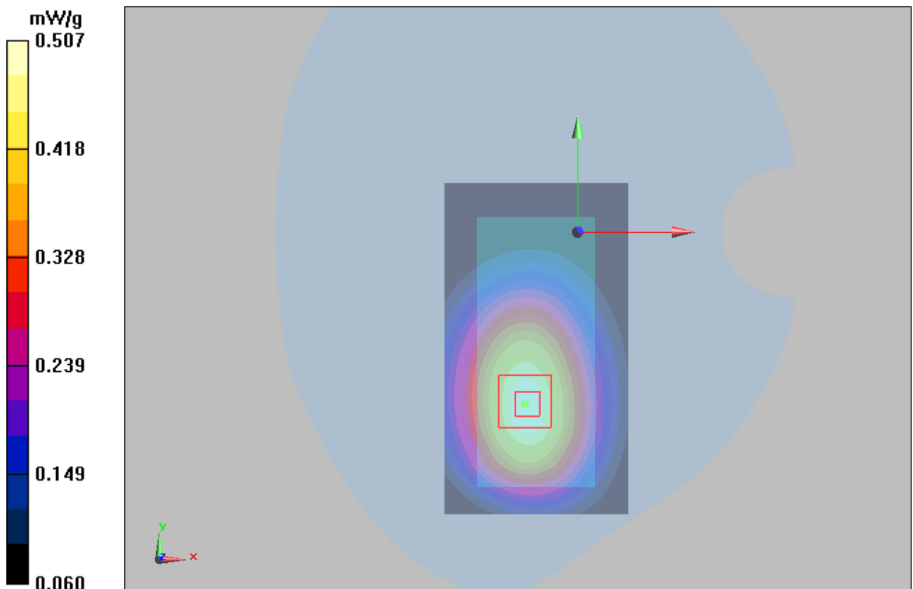
Figure 30 Body with Earphone, Towards Phantom, GSM 850 Channel 251
