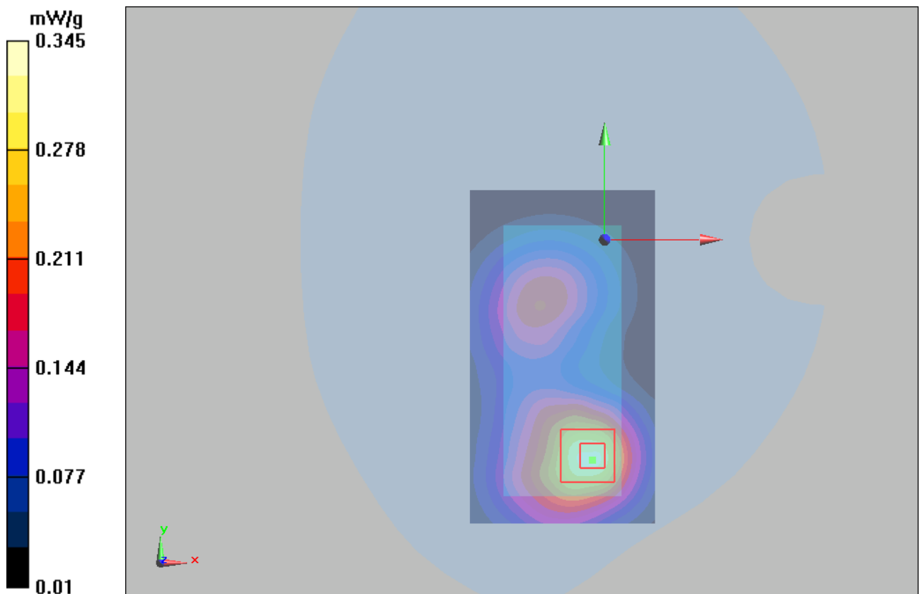
Figure 39 Body, Towards Phantom, GSM 1900 Channel 661
