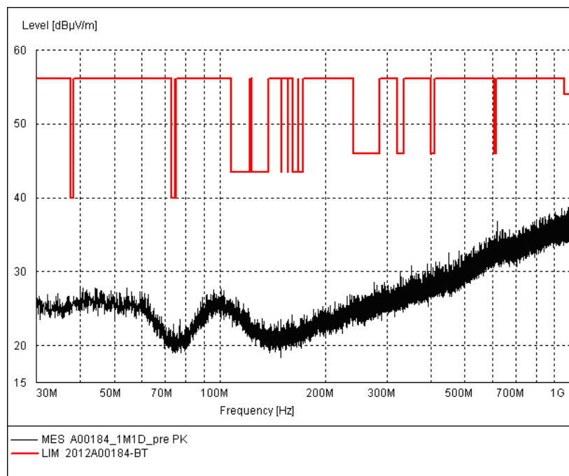
Fig.61. Radiated emission: GFSK, Channel 39, 30 MHz - 1 GHz
