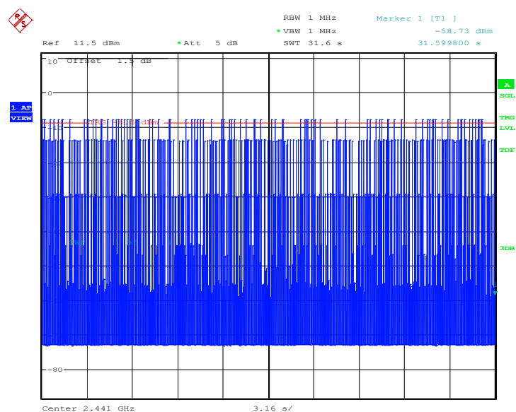
Fig.102. Time of occupancy (Dwell Time): Channel 39, Packet 2-DH3
