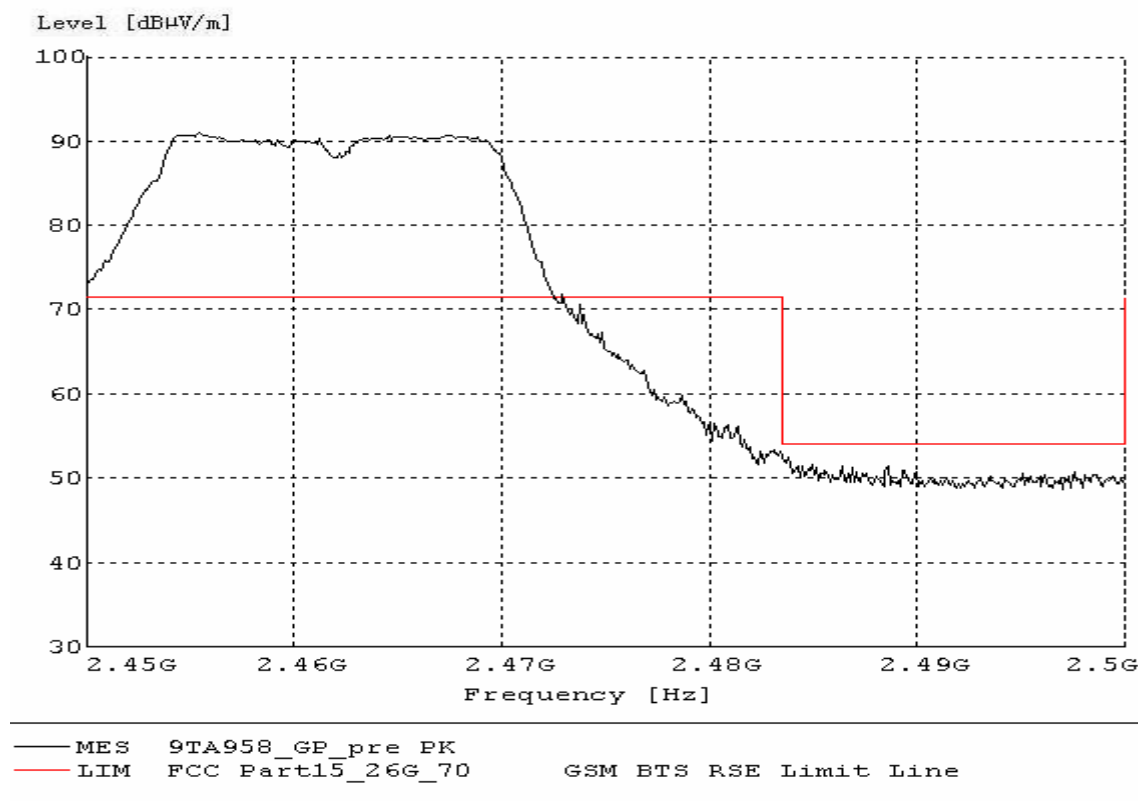
Fig. 39 Radiated Spurious Emission (Power): 802.11g, 2.45 GHz - 2.5GHz
