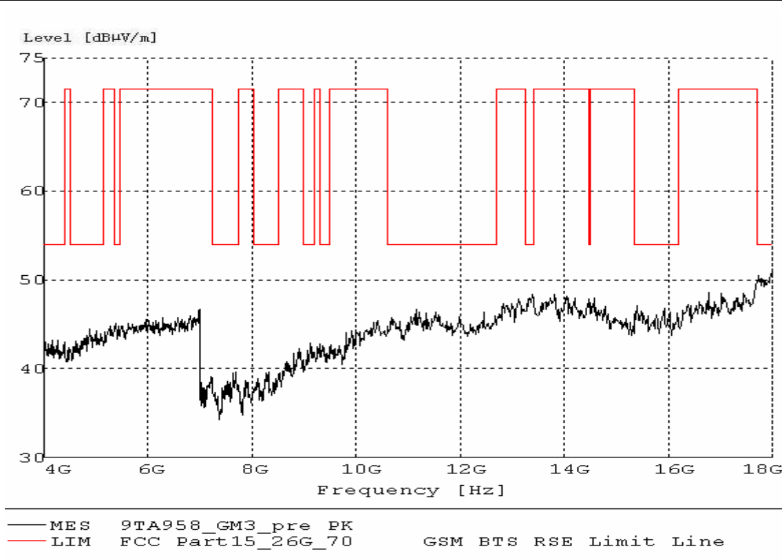
Fig. 45 Radiated Spurious Emission (802.11g, Ch6, 4 GHz-18 GHz)
