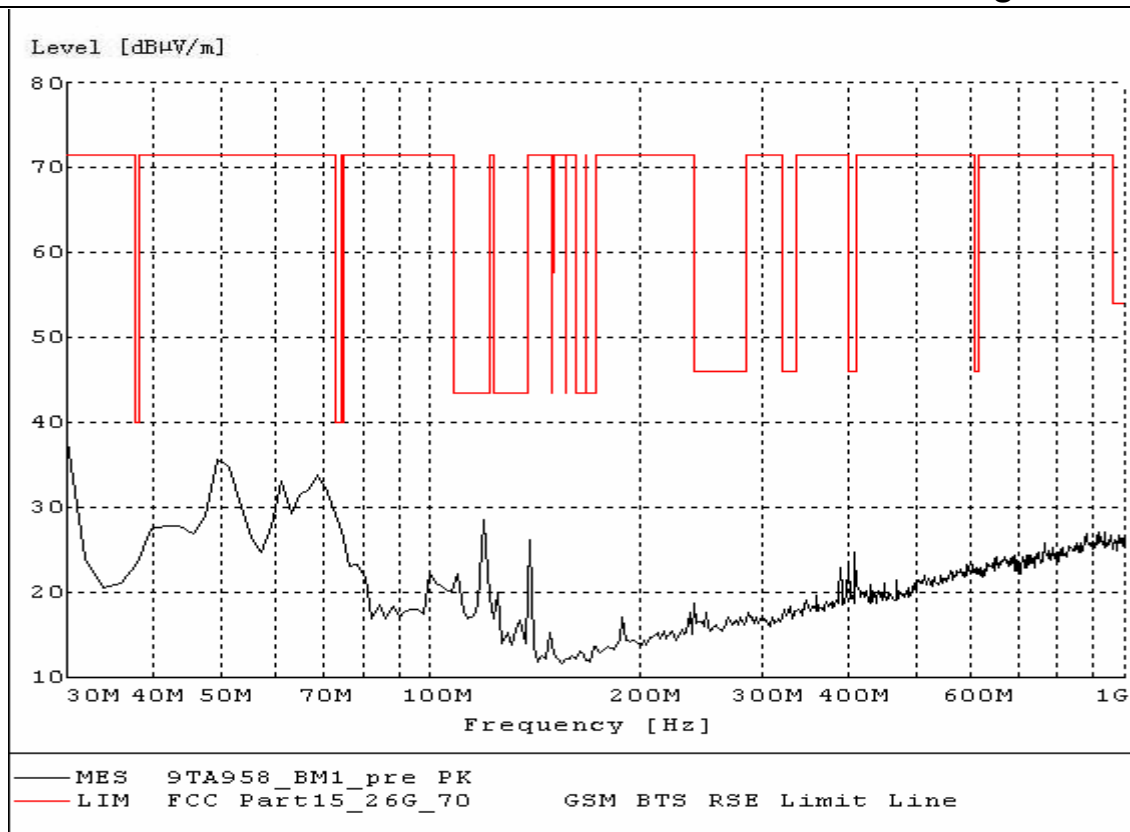
Fig. 33 Radiated Spurious Emission (802.11b, Ch6, 30 MHz-1 GHz)
