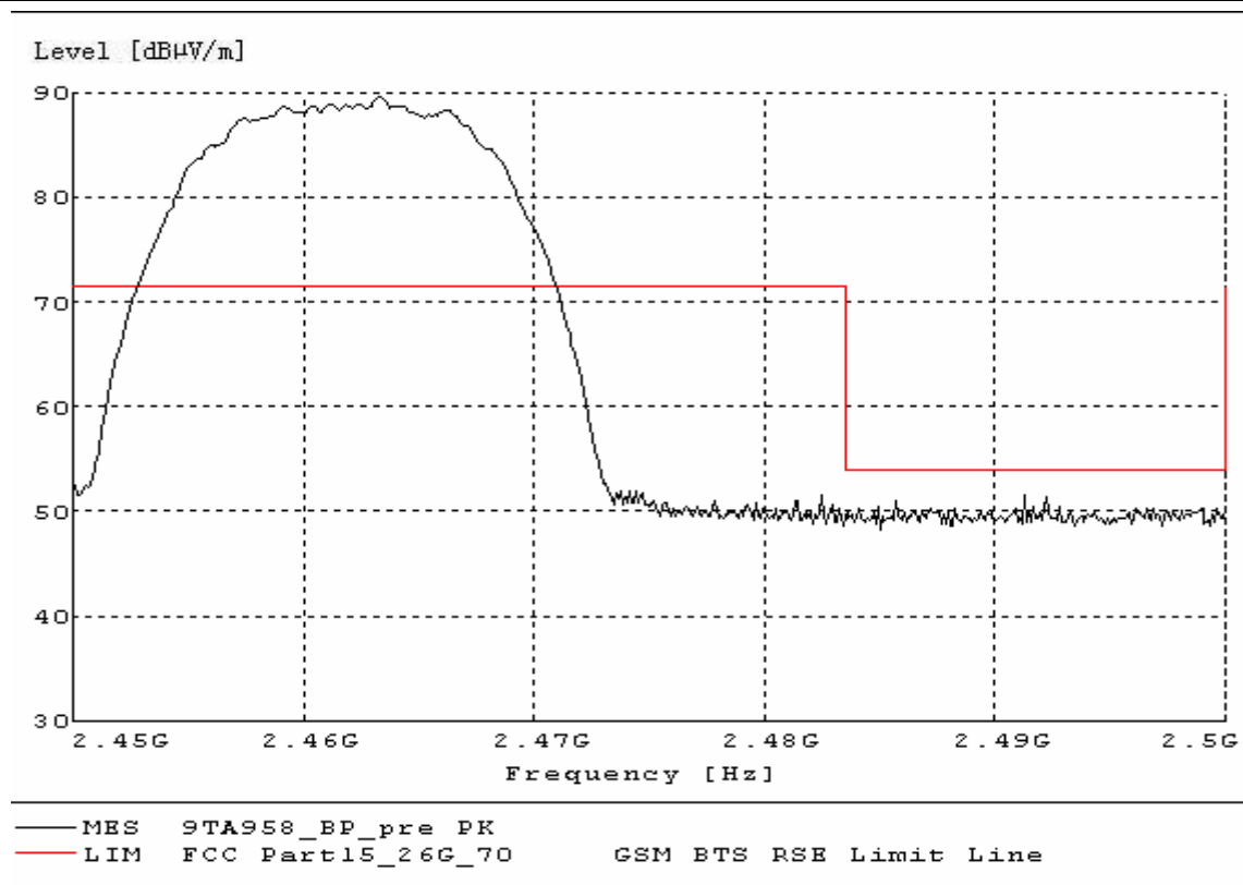
Fig. 29 Radiated Spurious Emission (Power): 802.11b, 2.45 GHz - 2.5GHz
