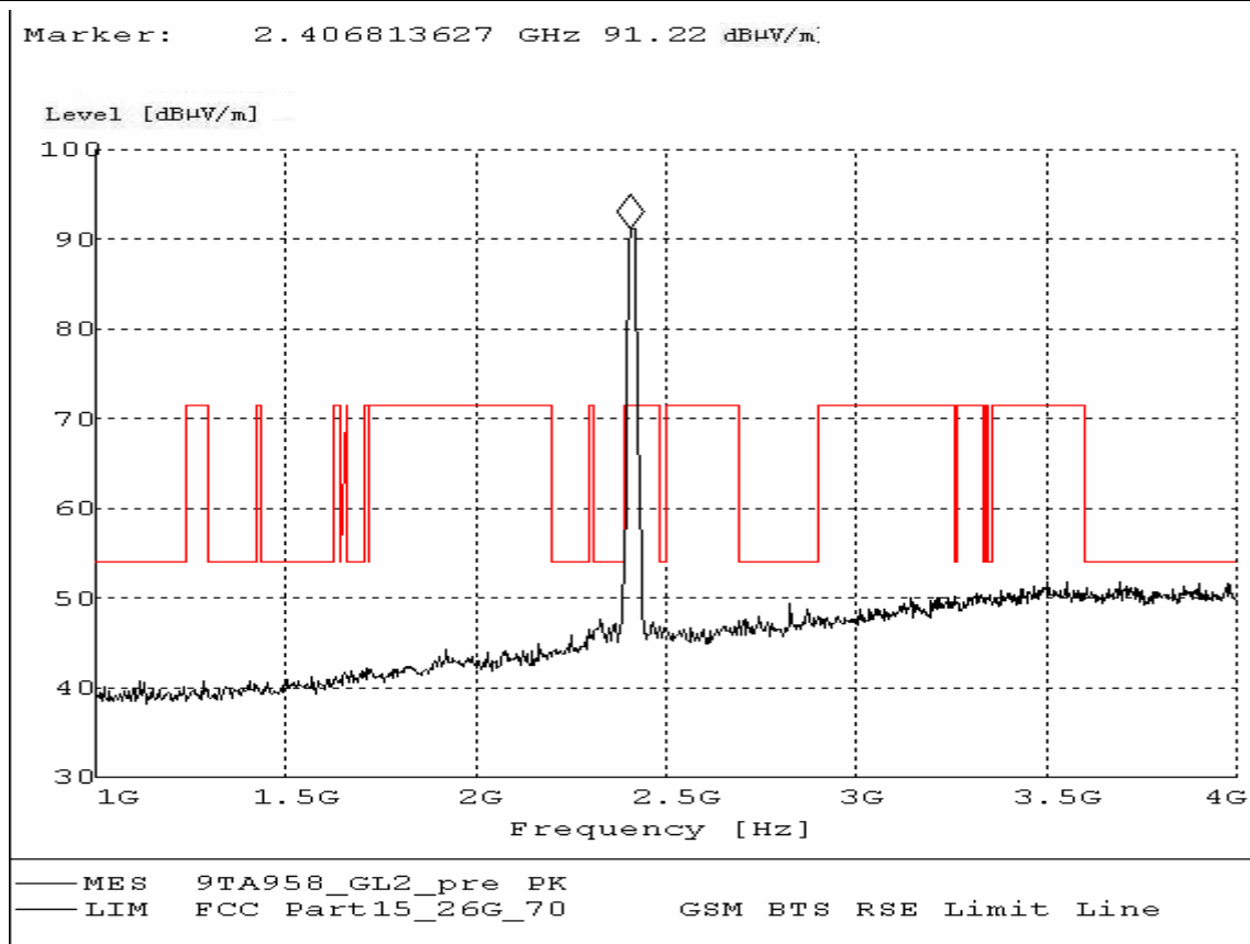
Fig. 41 Radiated Spurious Emission (802.11g, Ch1, 1 GHz-4 GHz)
