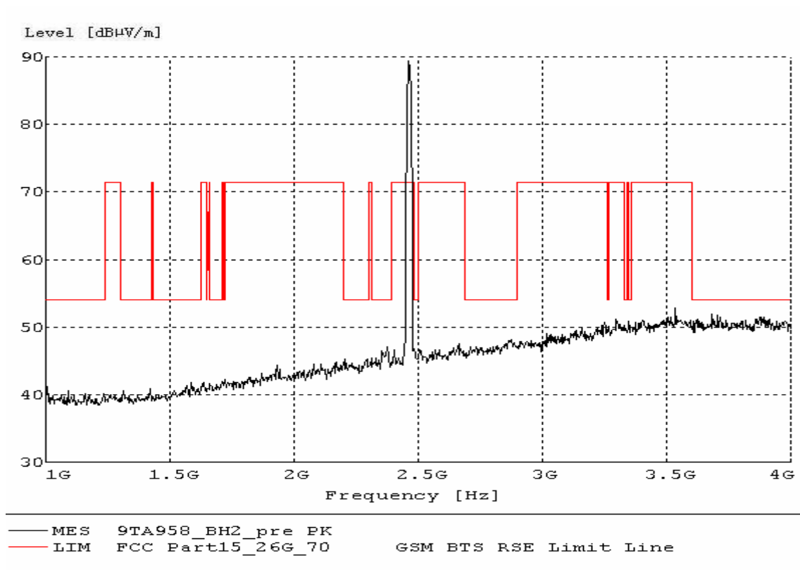
Fig. 37 Radiated Spurious Emission (802.11b, Ch11, 1 GHz-4 GHz)
