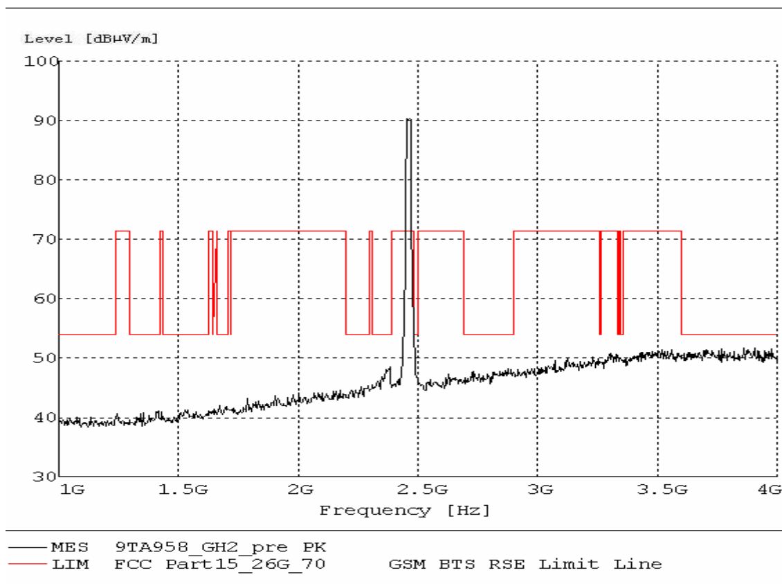
Fig. 47 Radiated Spurious Emission (802.11g, Ch11, 1 GHz-4 GHz)
