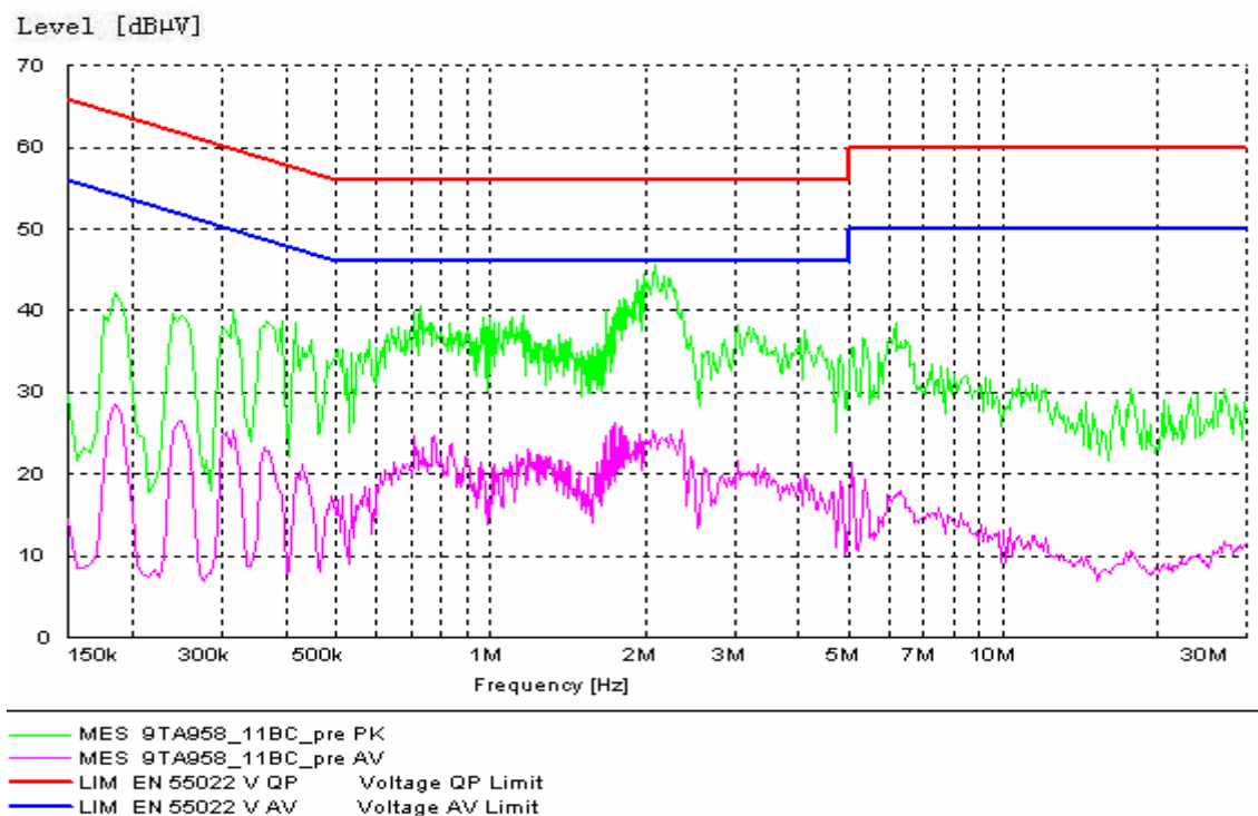
Fig. 50 AC Powerline Conducted Emission - 802.11b mode
