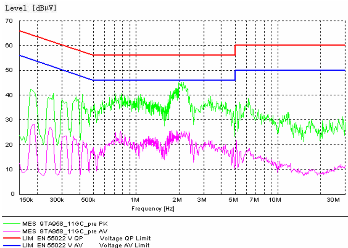
Fig. 51 AC Powerline Conducted Emission - 802.11g mode
