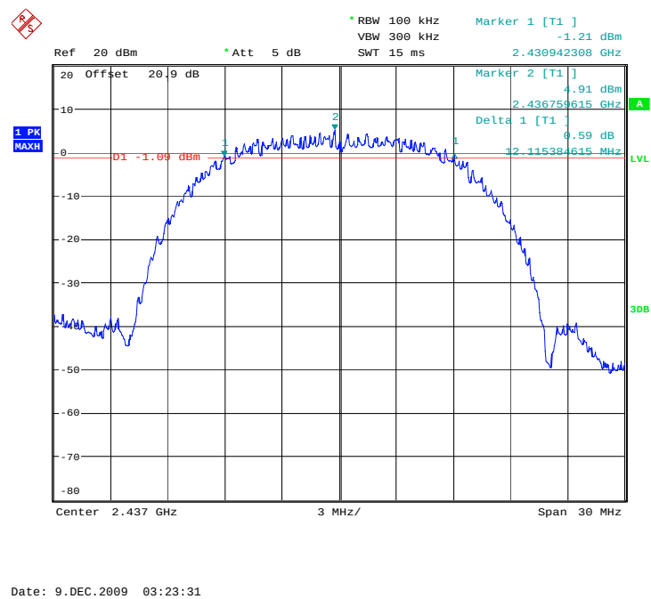
Fig. 2 Occupied 6dB Bandwidth (802.11b, Ch 6)
