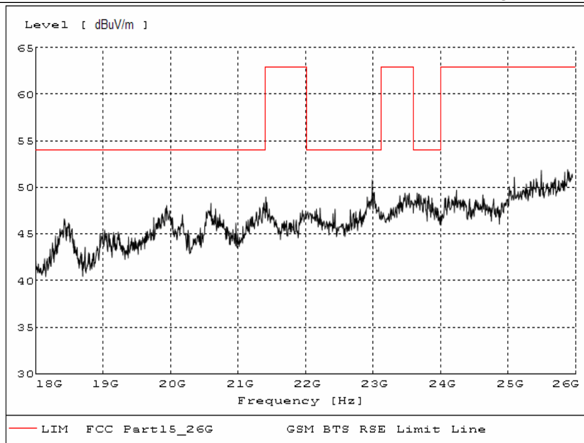
Fig. 49 Radiated emission: 18 GHz - 26 GHz
