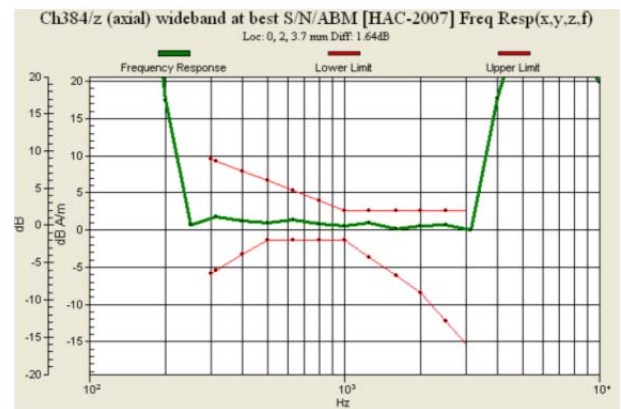
Fig. 9.2 CDMA2000 BC0 Ch384
