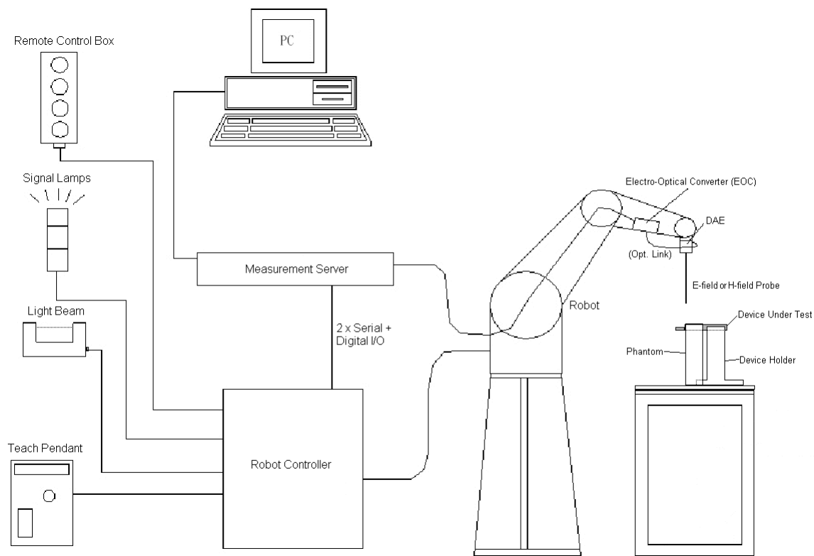
Fig 4.1 SPEAG DASY4 or DASY5 System Configurations
