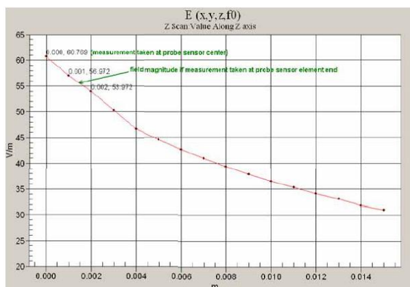
Fig 4.3 Z-Axis Scan at maximum point above a typical wireless device for E-field
