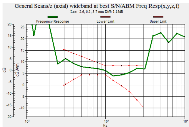
Fig 9.9 CDMA2000 BC1 Ch1175
