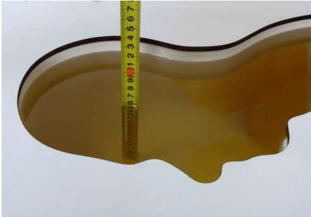
Picture 3: Liquid depth in the head Phantom (900MHz) (16cm deep)
