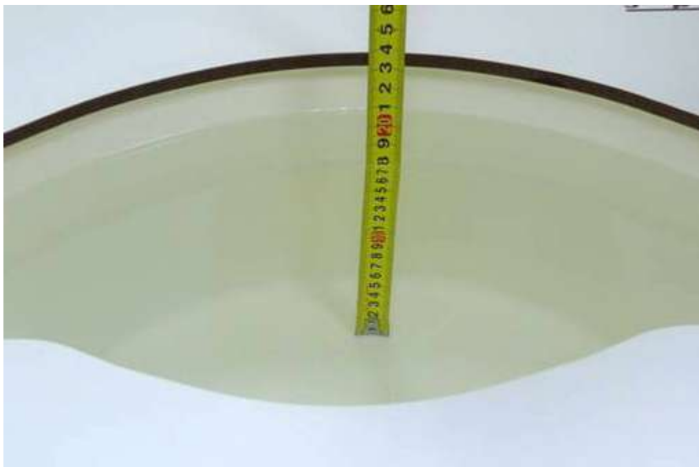
Picture 4: Liquid depth in the flat Phantom (1900 MHz) (16cm deep)
