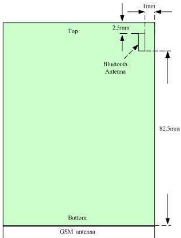
Picture: position of antenna
