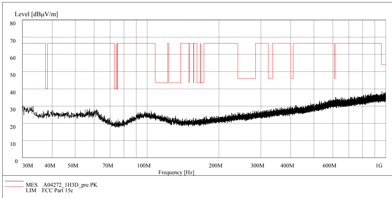
Fig.88. Radiated emission: 8DPSK, Channel 78, 30 MHz - 1 GHz
