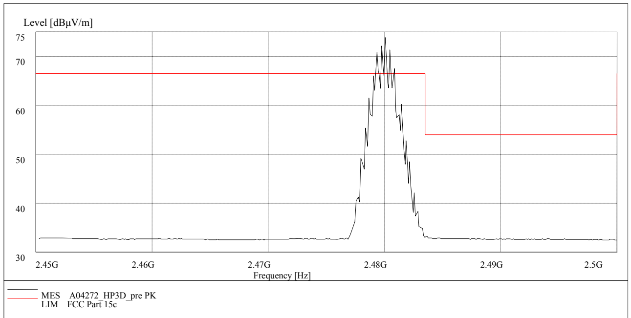
Fig.92. Radiated emission (Power): 8DPSK, high channel
