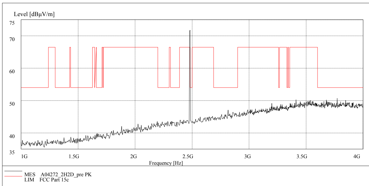
Fig.77. Radiated emission: \pi/4 DQPSK, Channel 78, 1 GHz - 4 GHz
