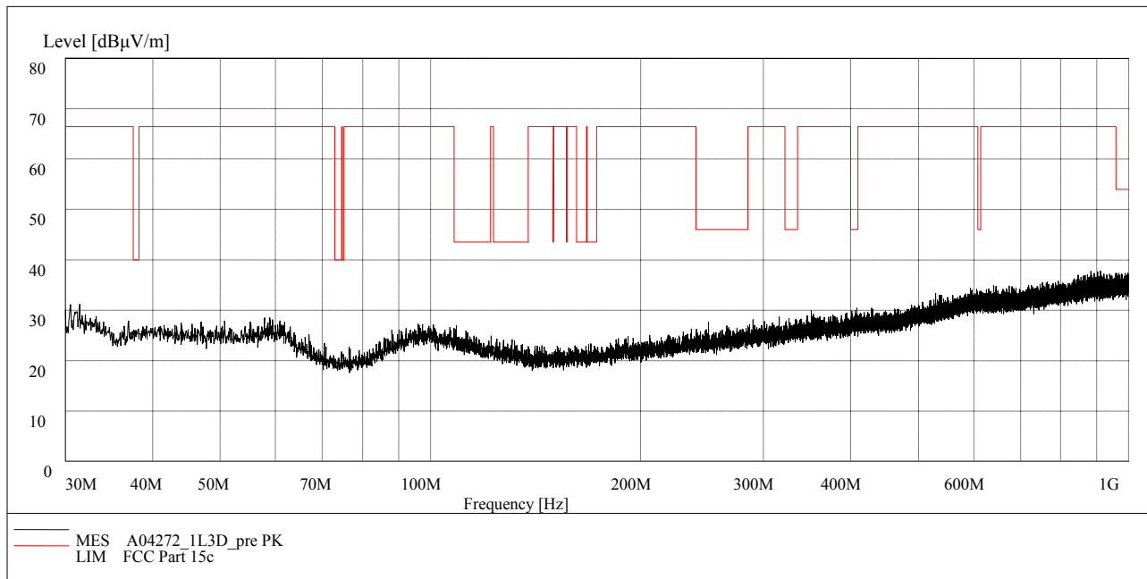
Fig.82. Radiated emission: 8DPSK, Channel 0, 30 MHz - 1 GHz
