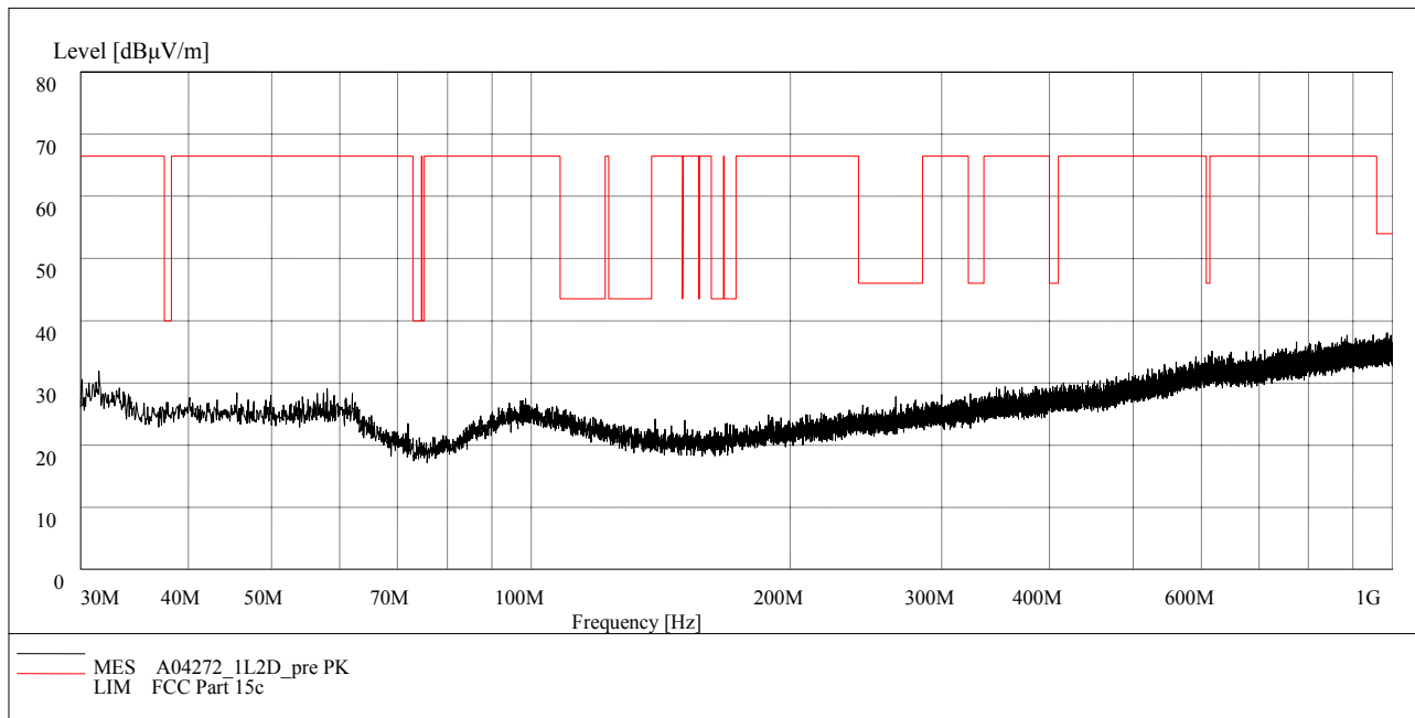
Fig.70. Radiated emission: \pi/4 DQPSK, Channel 0, 30 MHz - 1 GHz
