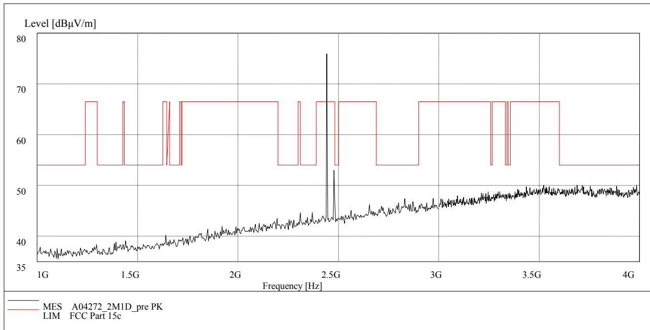
Fig.62. Radiated emission: GFSK, Channel 39, 1 GHz - 4 GHz
