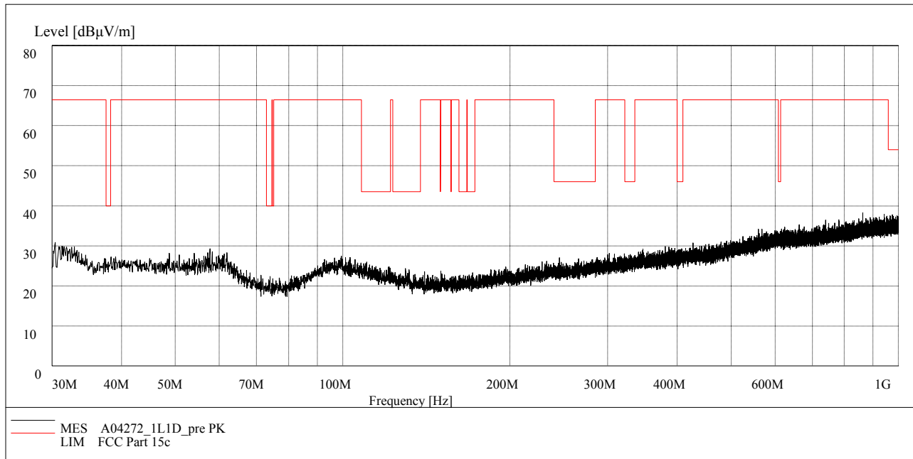
Fig.58. Radiated emission: GFSK, Channel 0, 30 MHz - 1 GHz
