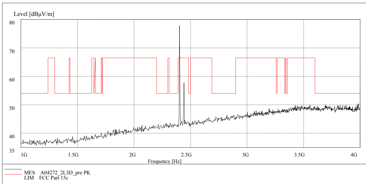
Fig.83. Radiated emission: 8DPSK, Channel 0, 1 GHz - 4 GHz
