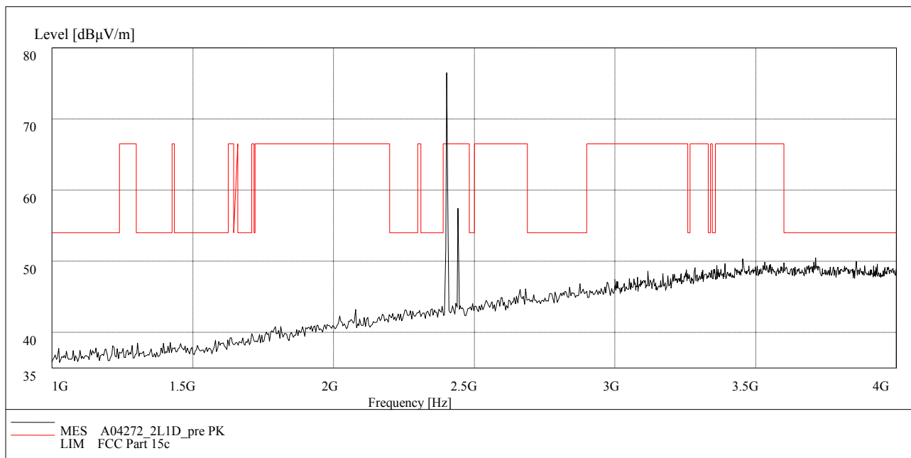
Fig.59. Radiated emission: GFSK, Channel 0, 1 GHz - 4 GHz
