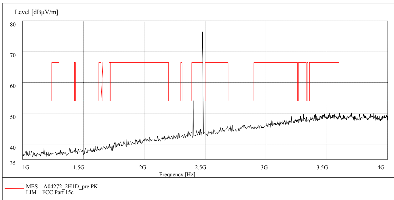
Fig.65. Fig.47 Radiated emission: GFSK, Channel 78, 1 GHz - 4 GHz
