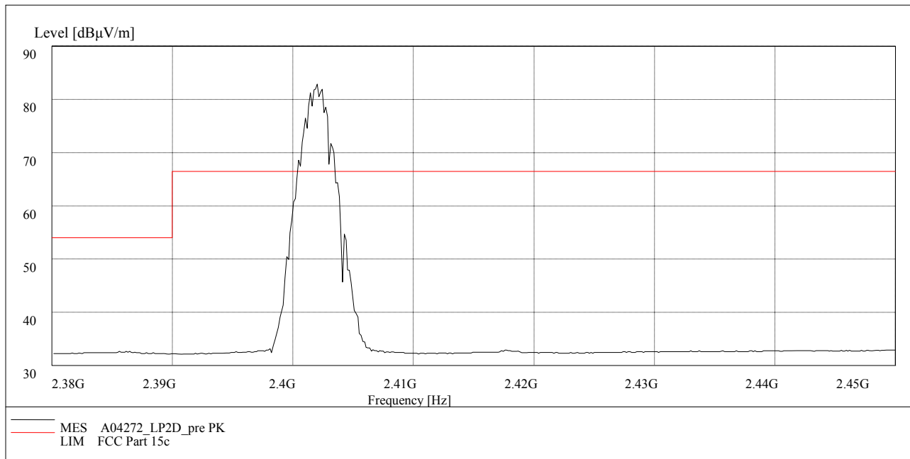
Fig.79. Radiated emission (Power): \pi/4 DQPSK, low channel
