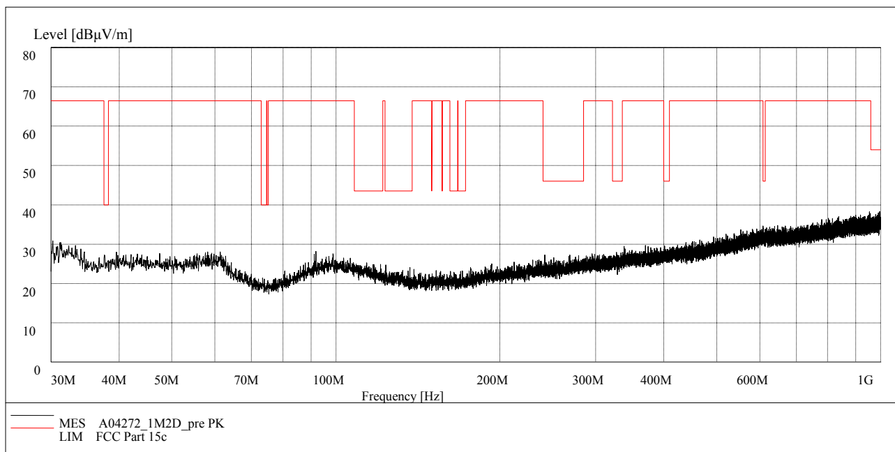
Fig.73. Radiated emission: \pi/4 DQPSK, Channel 39, 30 MHz - 1 GHz
