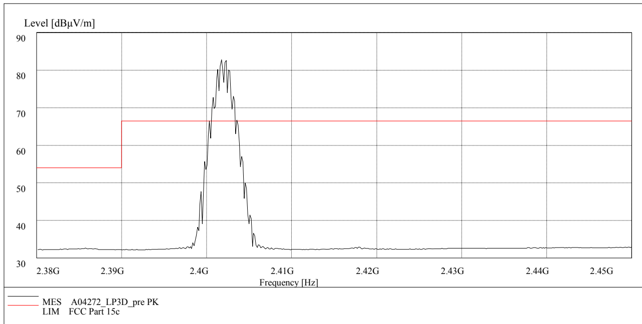
Fig.91. Radiated emission (Power): 8DPSK, low channel
