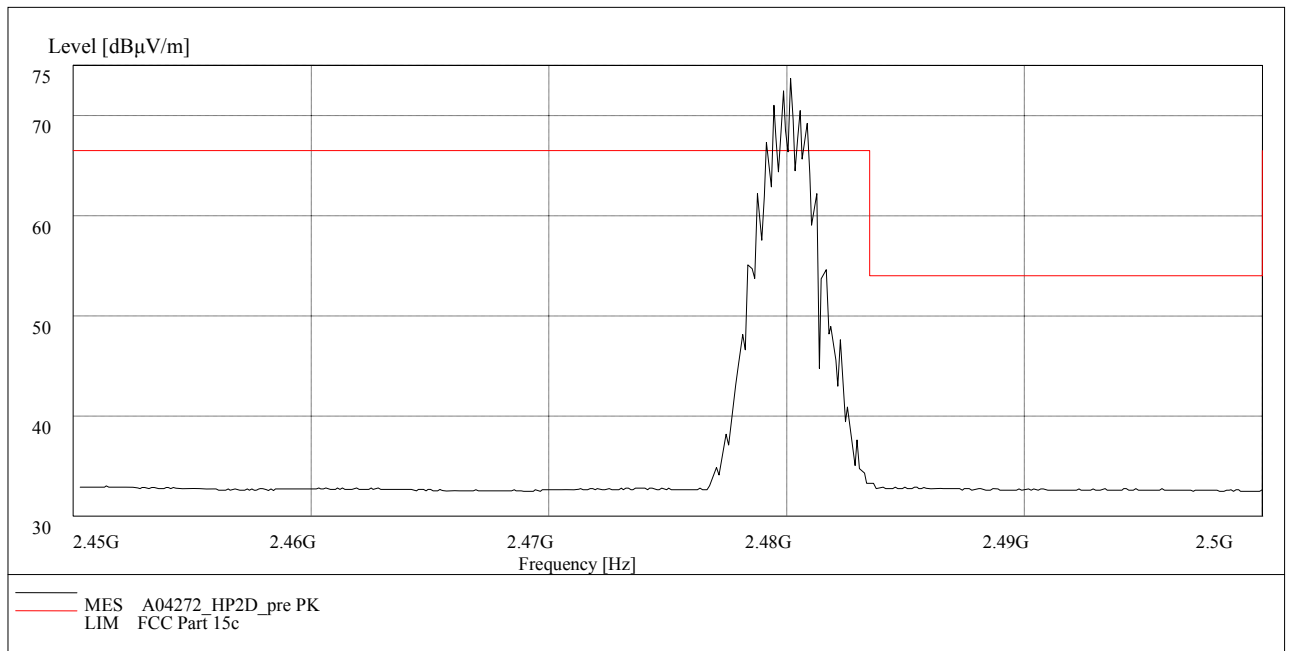
Fig.80. Radiated emission (Power): \pi/4 DQPSK, high channel
