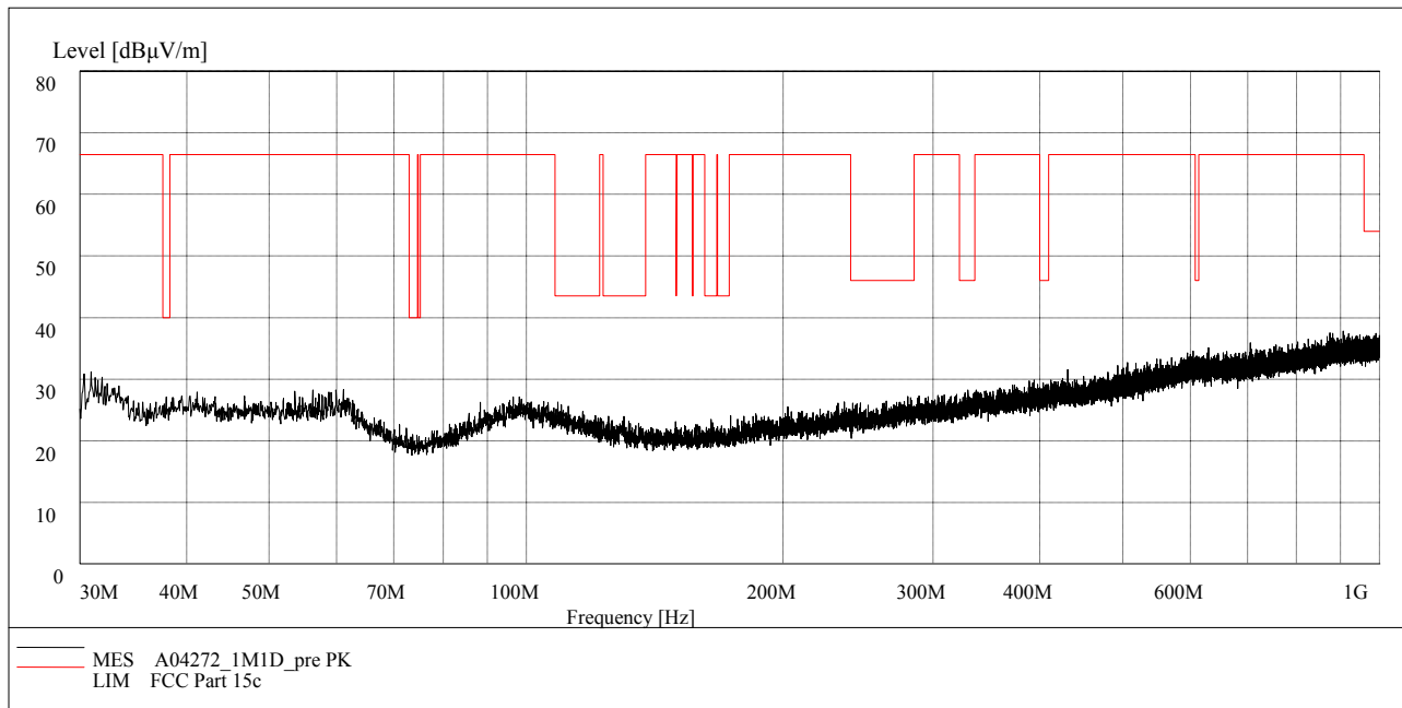
Fig.61. Radiated emission: GFSK, Channel 39, 30 MHz - 1 GHz
