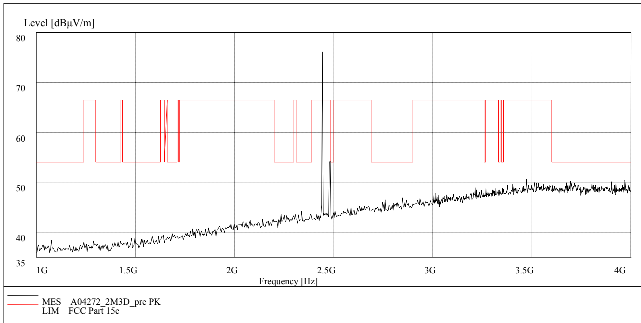
Fig.86. Radiated emission: 8DPSK, Channel 39, 1 GHz - 4 GHz
