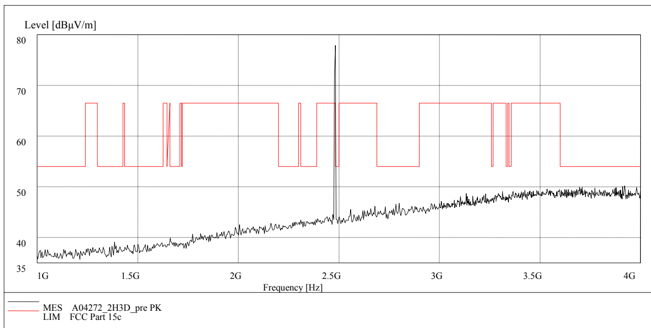
Fig.89. Radiated emission: 8DPSK, Channel 78, 1 GHz - 4 GHz
