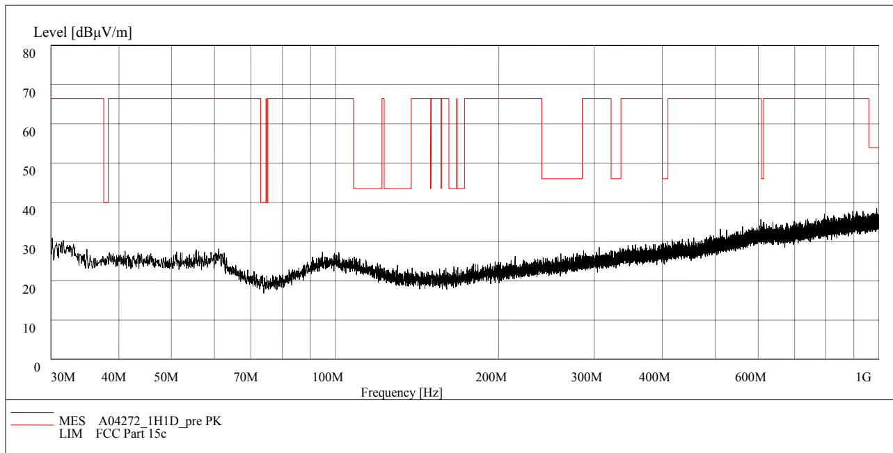
Fig.64. Radiated emission: GFSK, Channel 78, 30 MHz - 1 GHz
