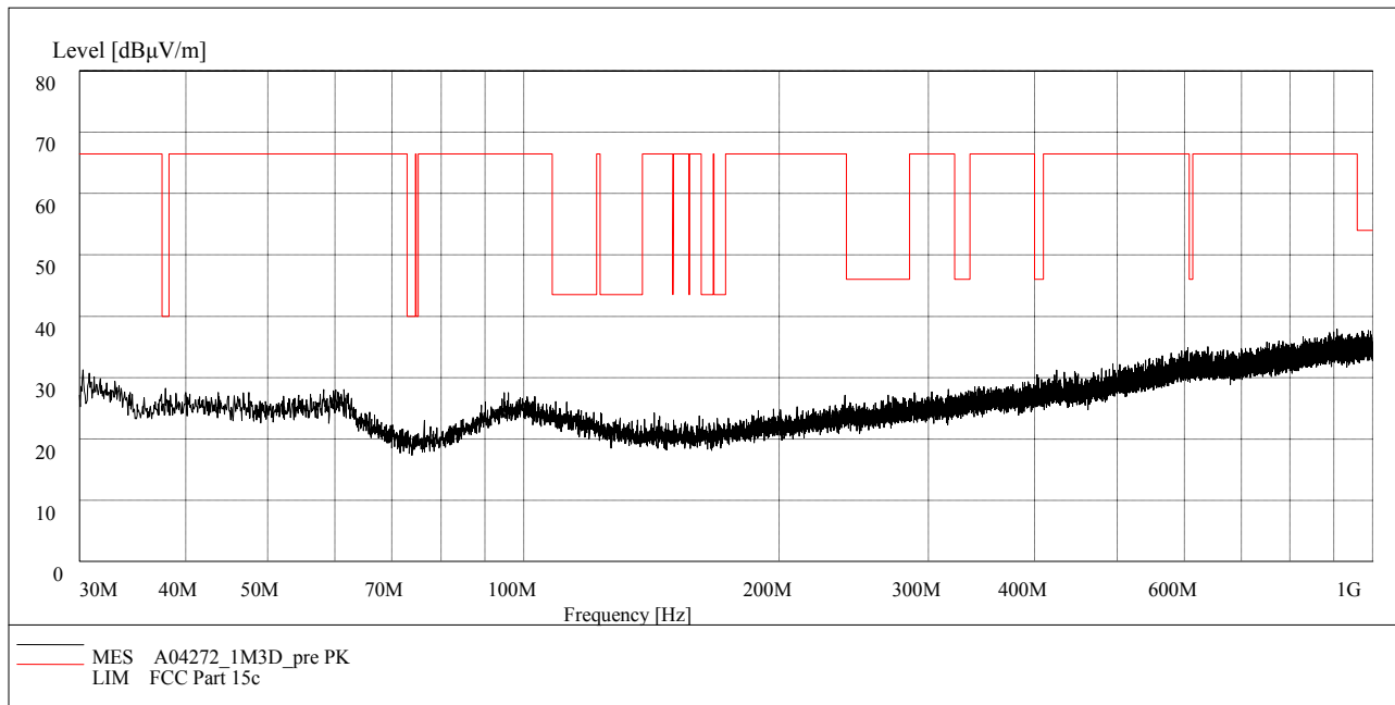
Fig.85. Radiated emission: 8DPSK, Channel 39, 30 MHz - 1 GHz
