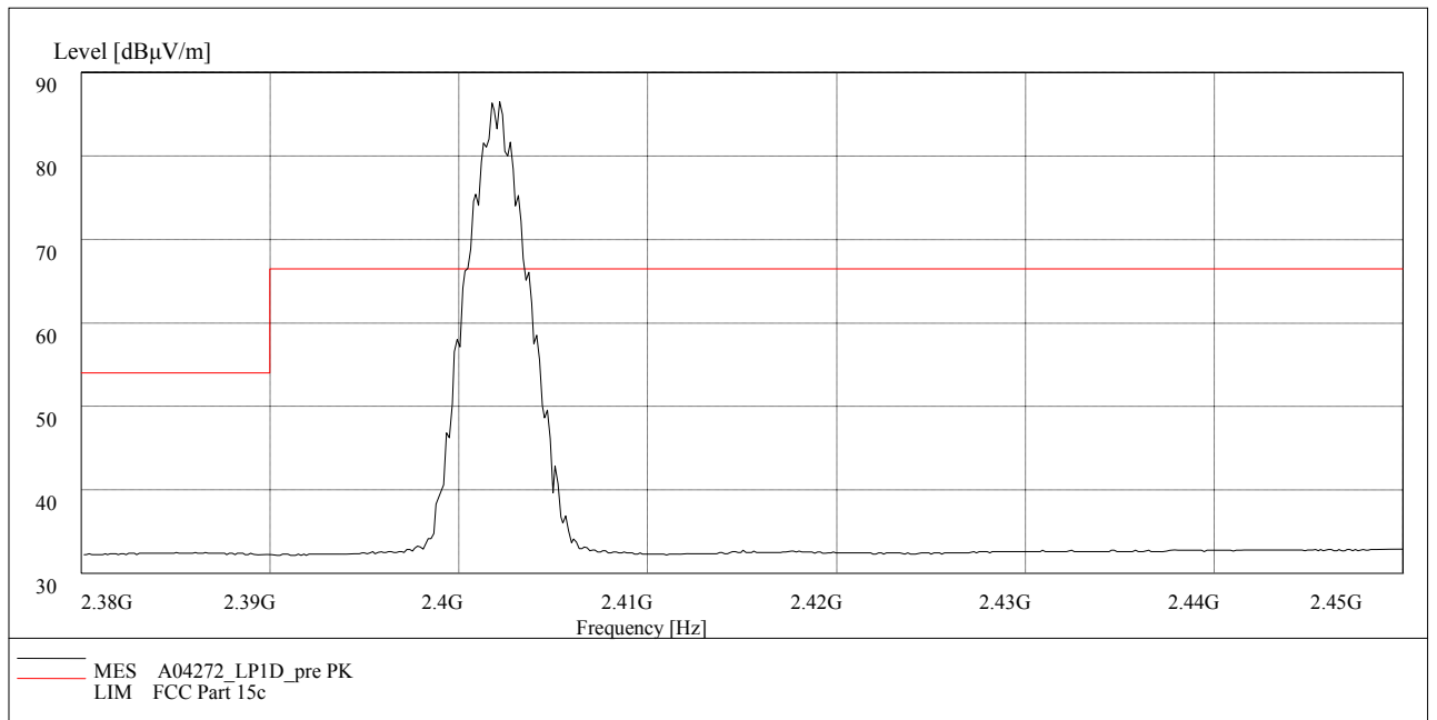
Fig.67. Radiated emission (Power) GFSK low channel
