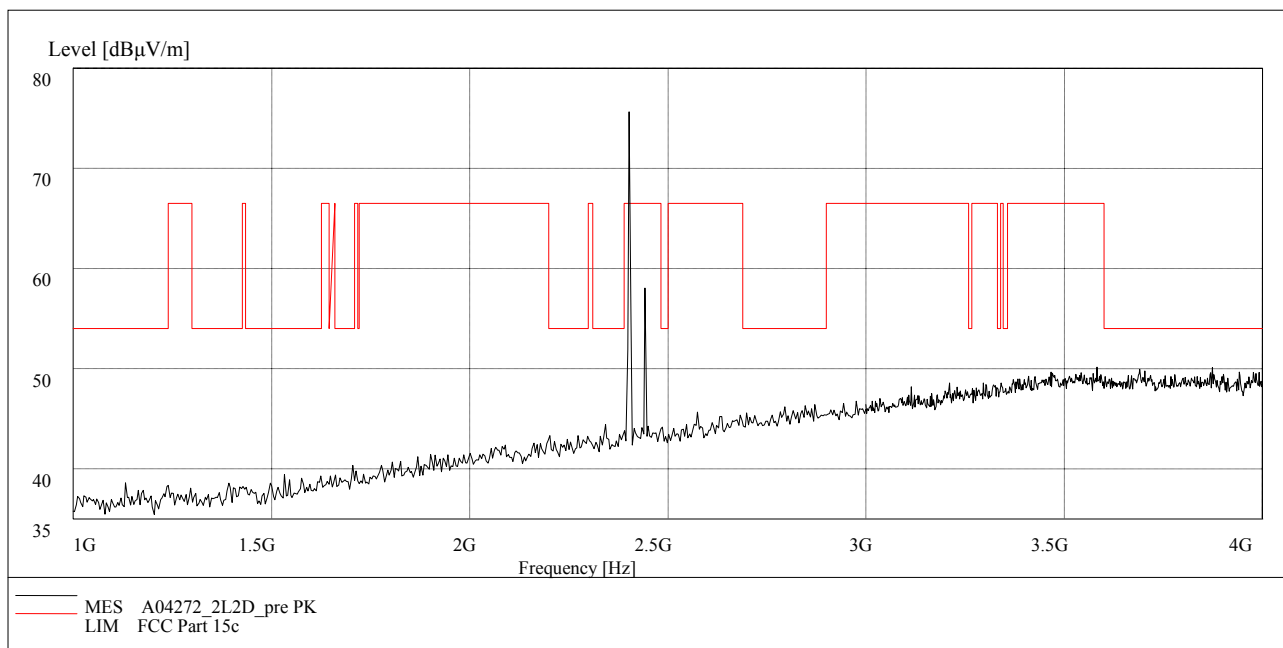
Fig.71. Radiated emission: \pi/4 DQPSK, Channel 0, 1 GHz - 4 GHz
