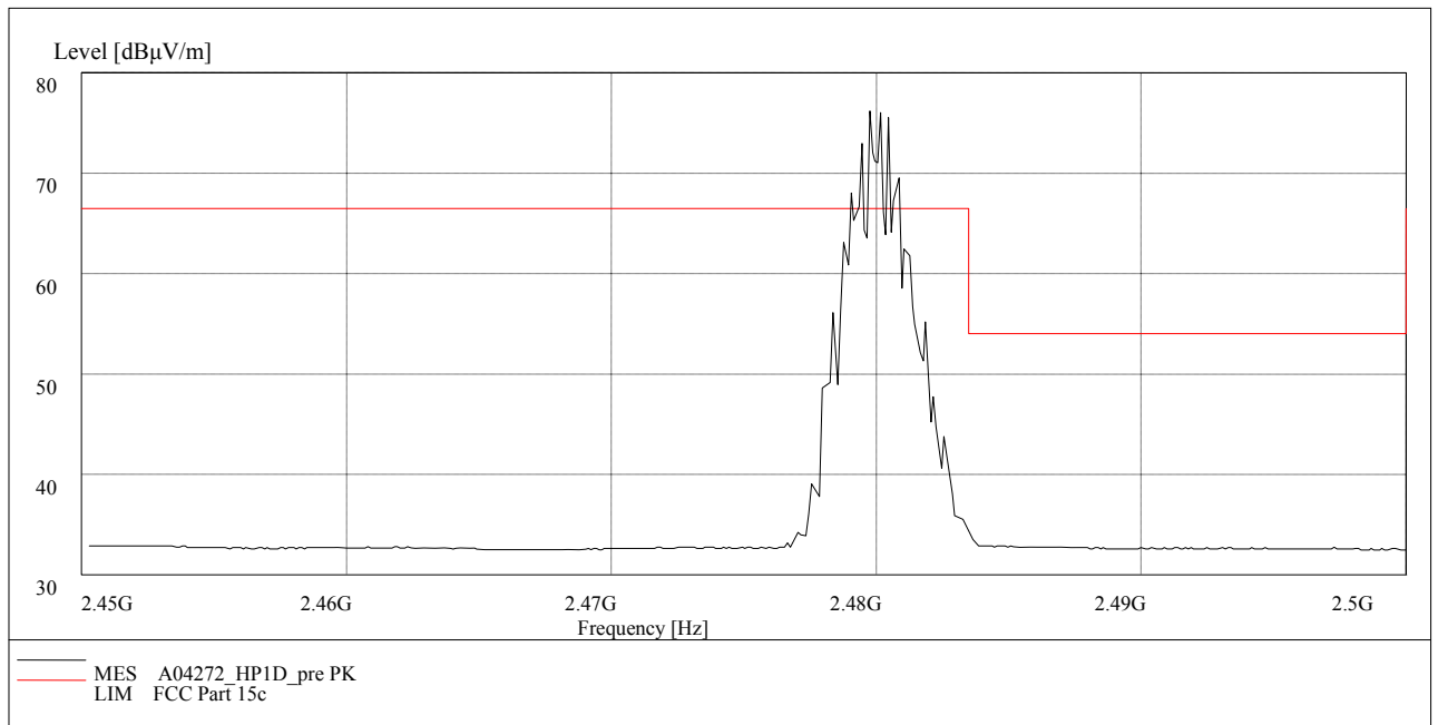
Fig.68. Radiated emission (Power) GFSK high channel
