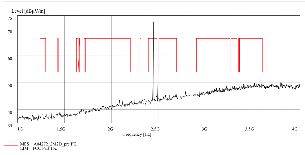
Fig.74. Radiated emission: \pi/4 DQPSK, Channel 39, 1 GHz - 4 GHz
