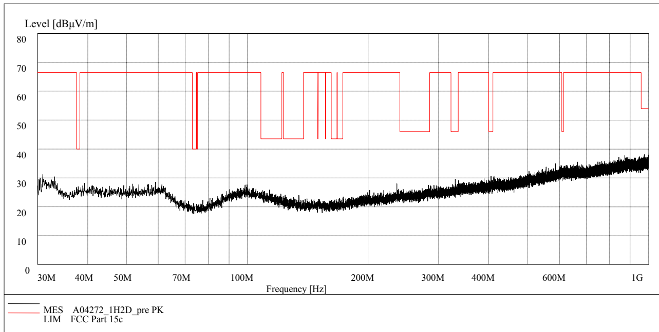
Fig.76. Radiated emission: \pi/4 DQPSK, Channel 78, 30 MHz - 1 GHz
