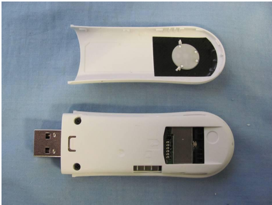
Pic A-4 USB Modem Disassembly
