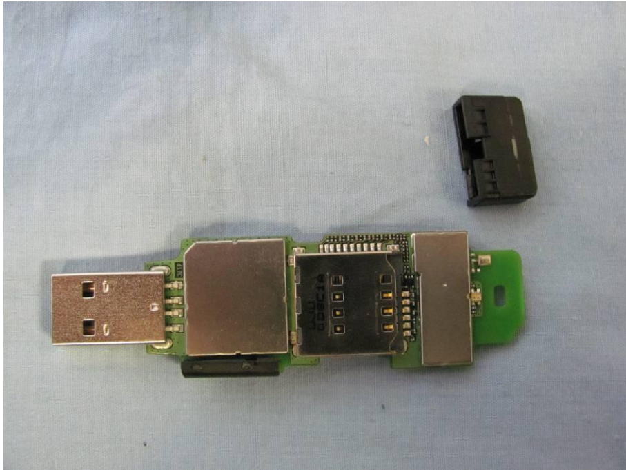
Pic A-7 USB Modem Disassembly
