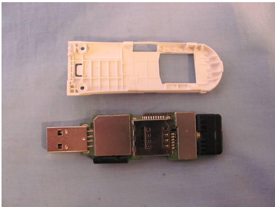
Pic A-6 USB Modem Disassembly
