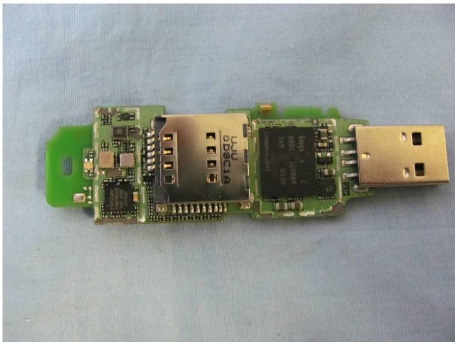
Pic A-8 USB Modem Disassembly
