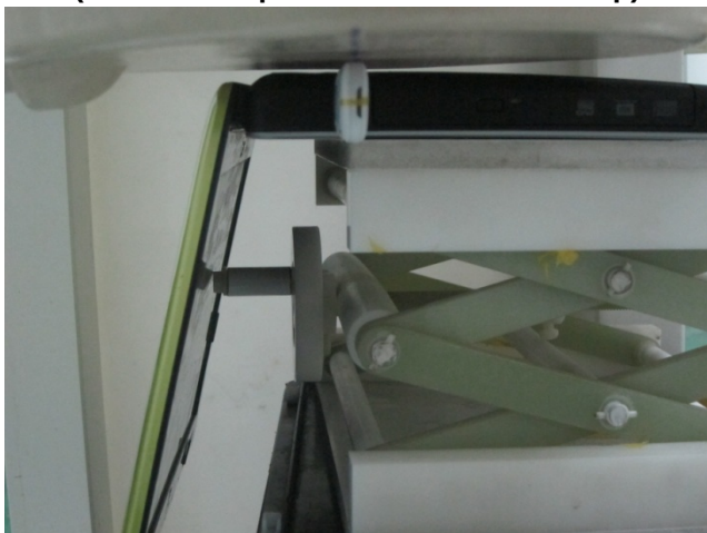
Direct Laptop Plug-in USB Configuration 3 (Vertical Front with Phantom 5 mm Gap)
