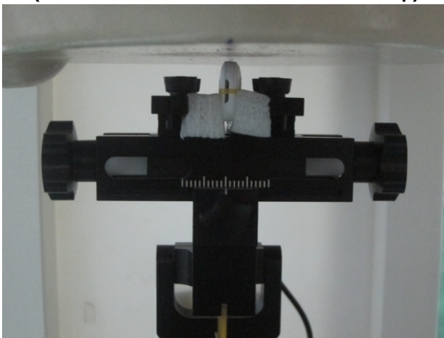
USB Cable Plug-in for USB Configuration 4 (Vertical Back with Phantom 5 mm Gap)
