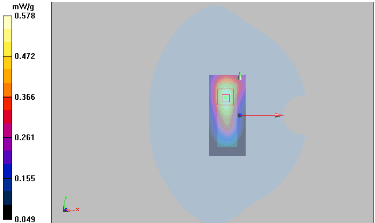
Figure 45 WCDMA Band V HSUPA with IBM T61 Test Position 1 Channel 4132
