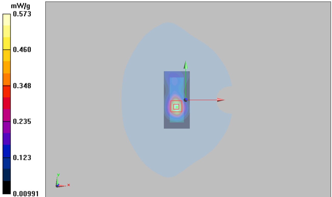
Figure 22 GSM 1900 GPRS (2TXslots) with IBM T61 Test Position 1 Channel 661
