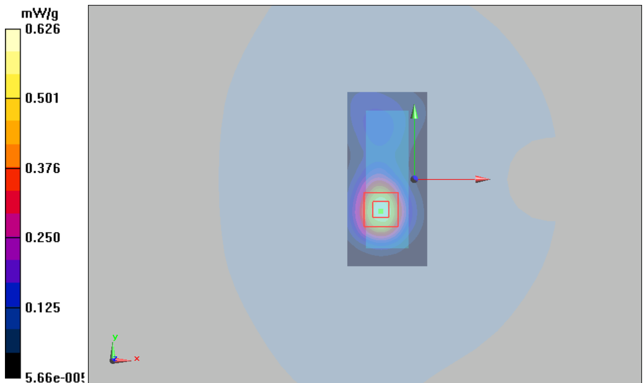
Figure 29 GSM 1900 EGPRS (4TXslots) with IBM T61 Test Position 1 Channel 512
