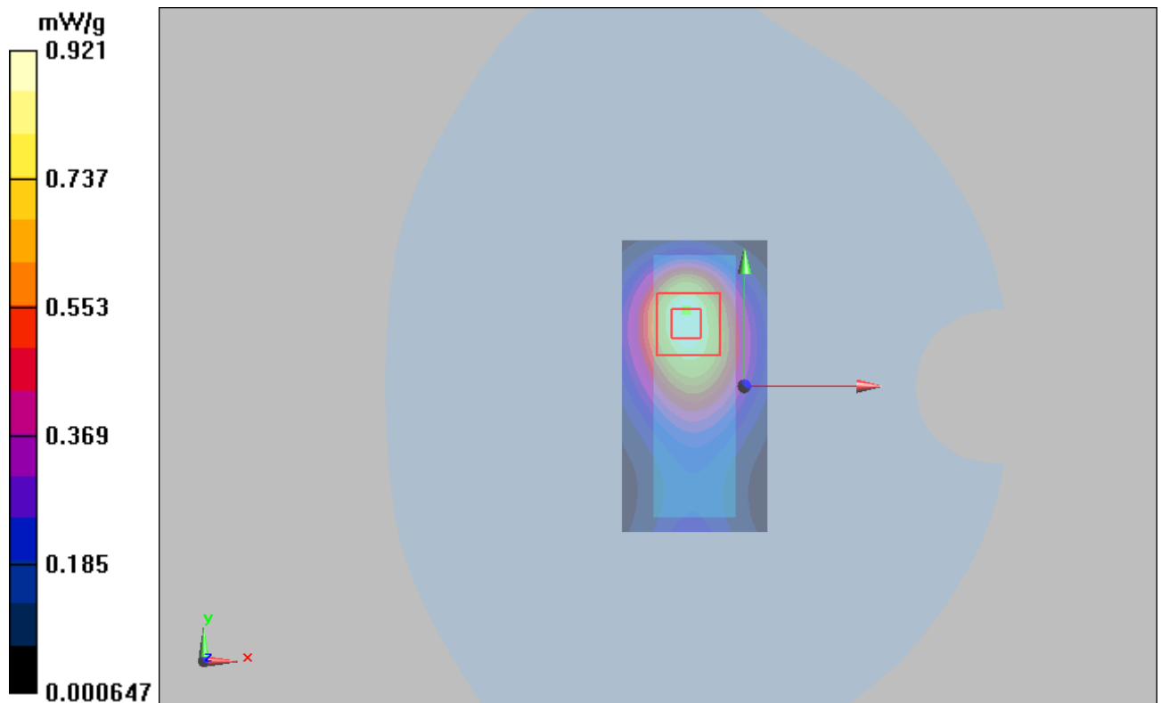
Figure 18 GSM 850 EGPRS (4Up) with IBM T61 Test Position 2 Channel 251
