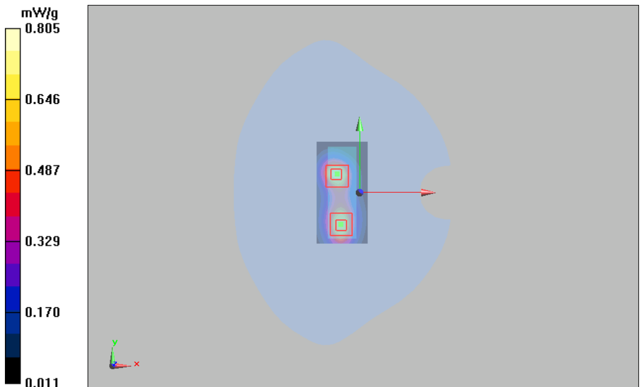
Figure 33 WCDMA Band II with IBM T61 Test Position 2 Channel 9400
