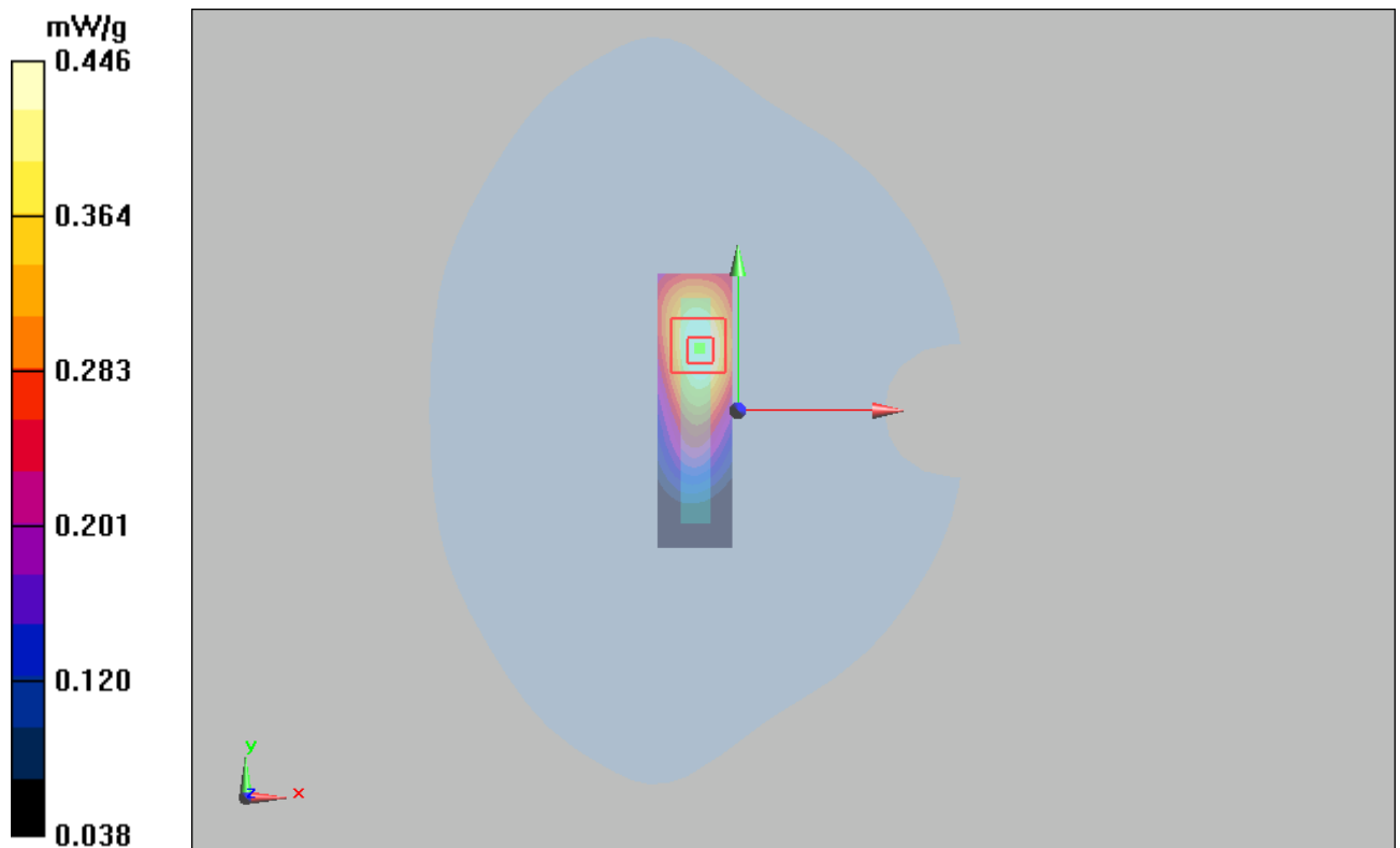
Figure 44 WCDMA Band V with Lenovo Y-450 Test Position 4 Channel 4183
