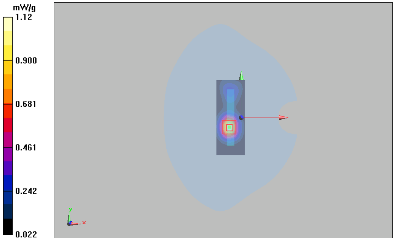
Figure 36 WCDMA Band II with Lenovo Y-450 Test Position 4 Channel 9400
