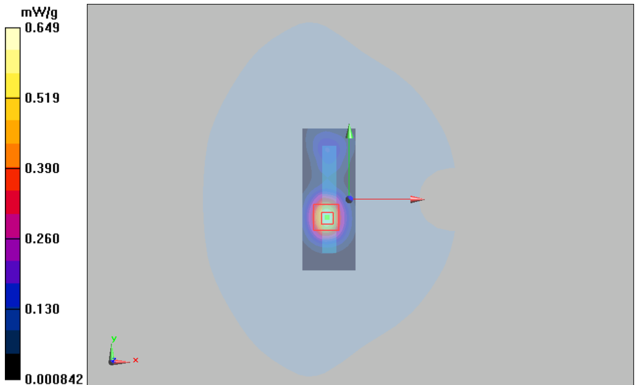
Figure 25 GSM 1900 GPRS (2Up) with Lenovo Y-450 Test Position 4 Channel 661
