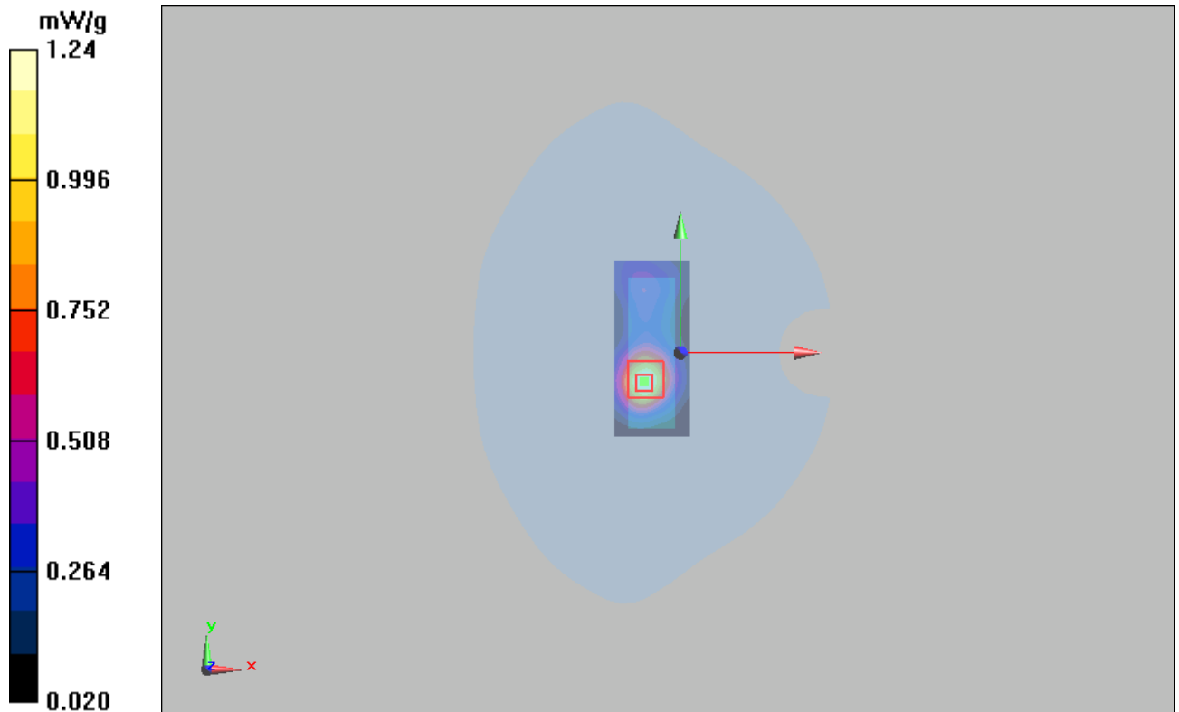
Figure 38 WCDMA Band II HSDPA with IBM T61 Test Position 1 Channel 9262
