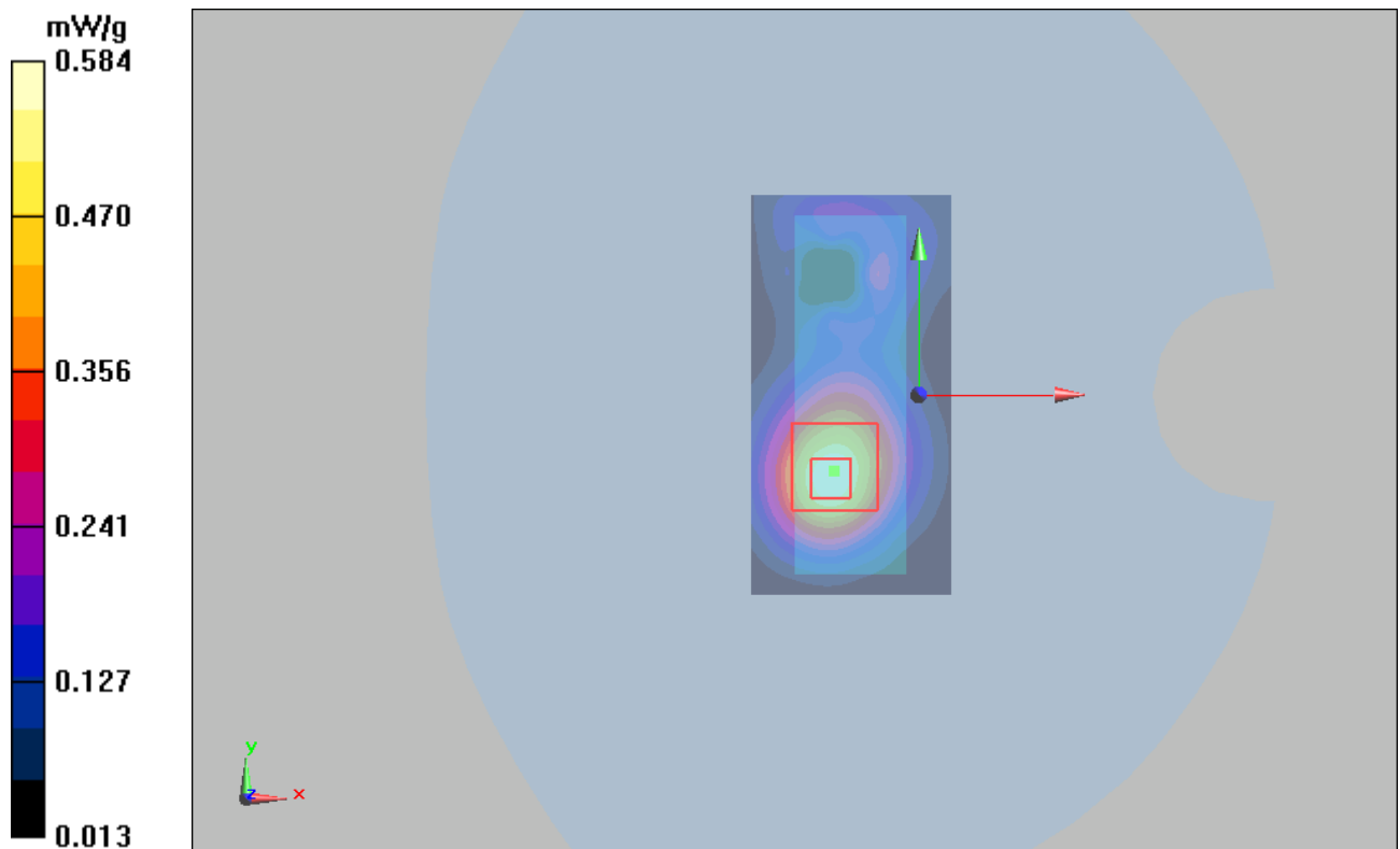
Figure 19 GSM 1900 GPRS (1Up) with IBM T61 Test Position 1 Channel 661
