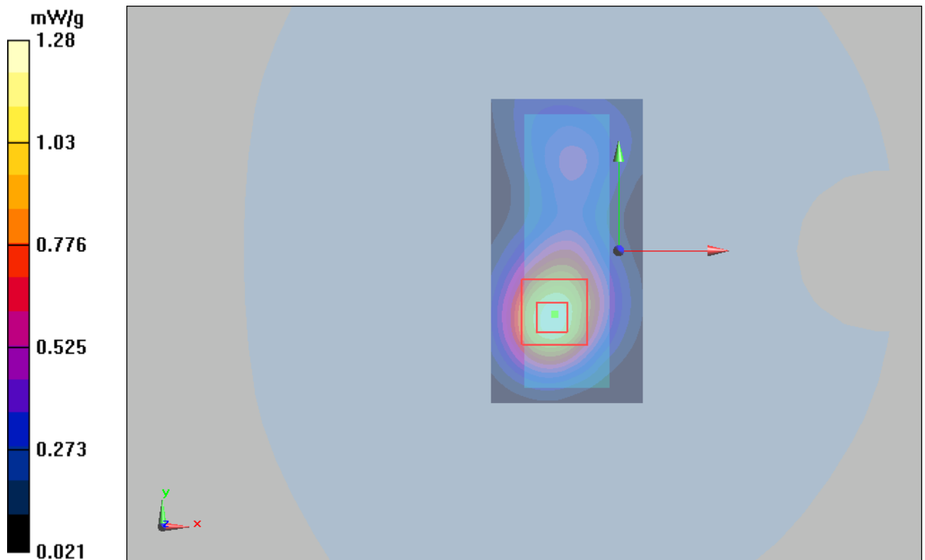
Figure 30 WCDMA Band II with IBM T61 Test Position 1 Channel 9538
