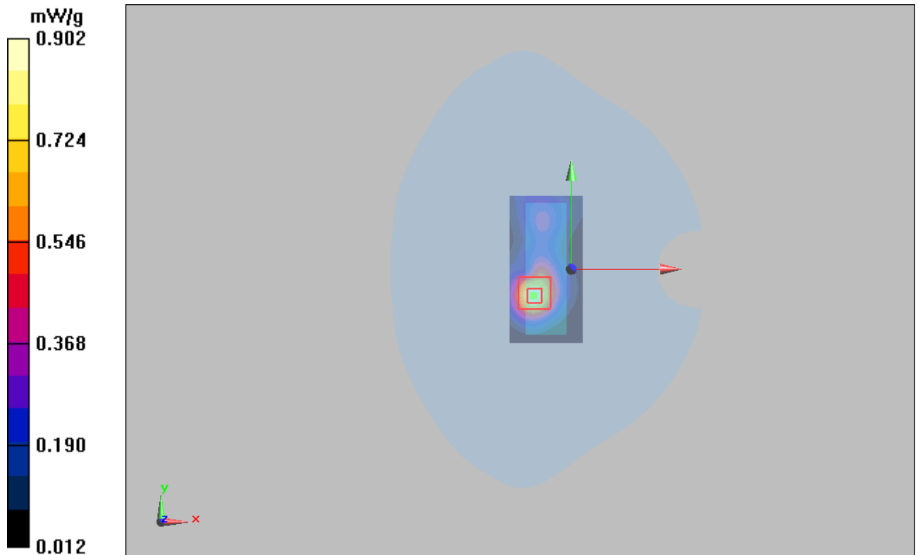
Figure 28 GSM 1900 EGPRS (3Up) with IBM T61 Test Position 1 Channel 512
