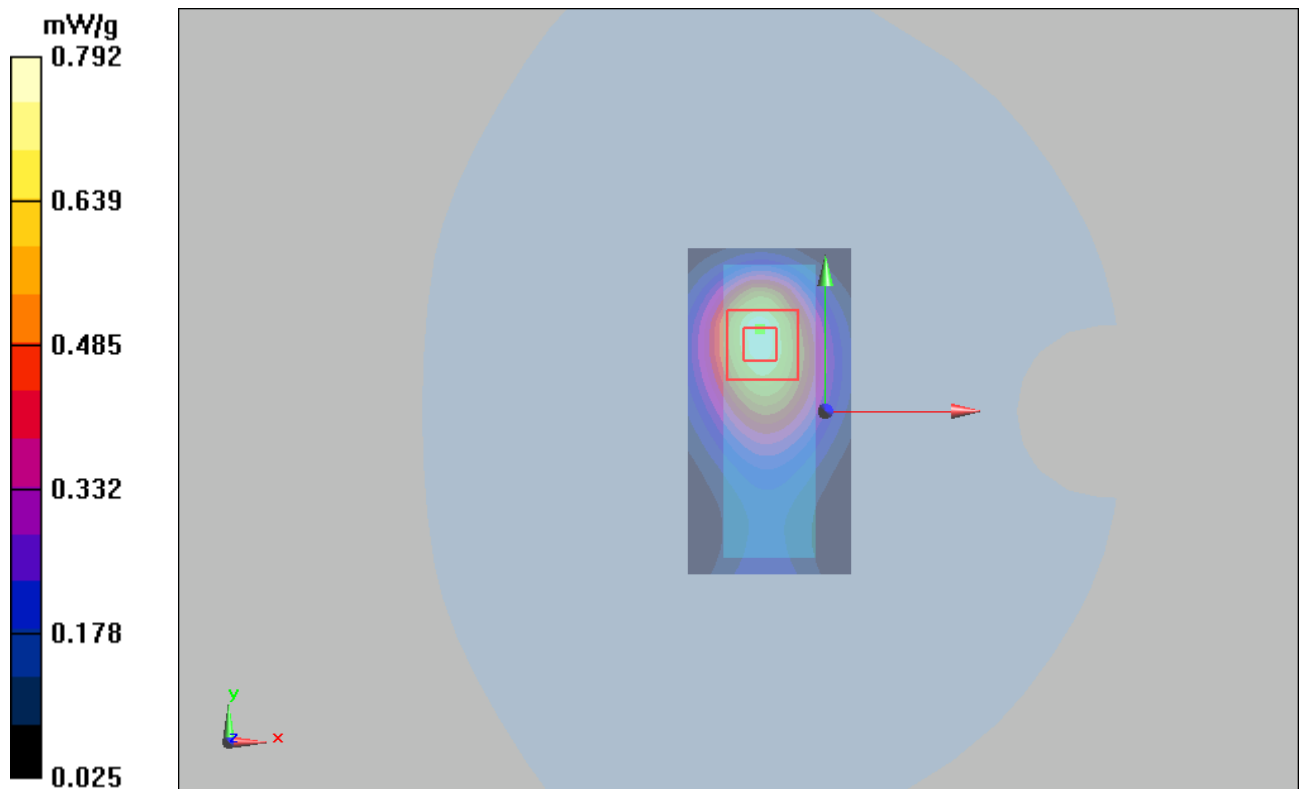
Figure 15 GSM 850 EGPRS (1Up) with IBM T61 Test Position 2 Channel 251
