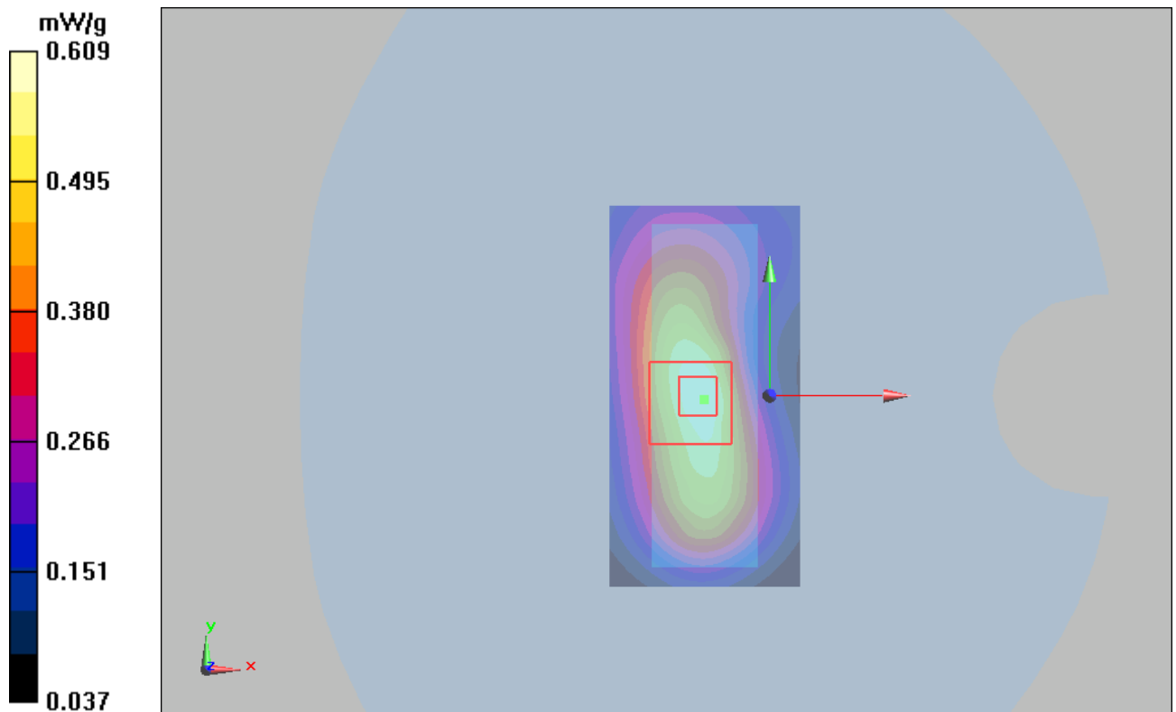
Figure 8 GSM 850 GPRS (1Up) with IBM T61 Test Position 1 Channel 190
