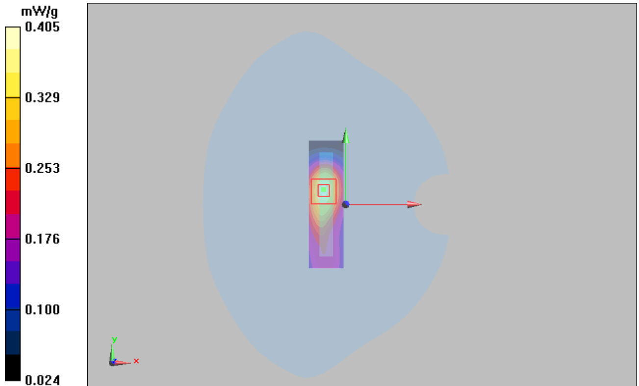
Figure 43 WCDMA Band V with Lenovo Y-450 Test Position 3 Channel 4183
