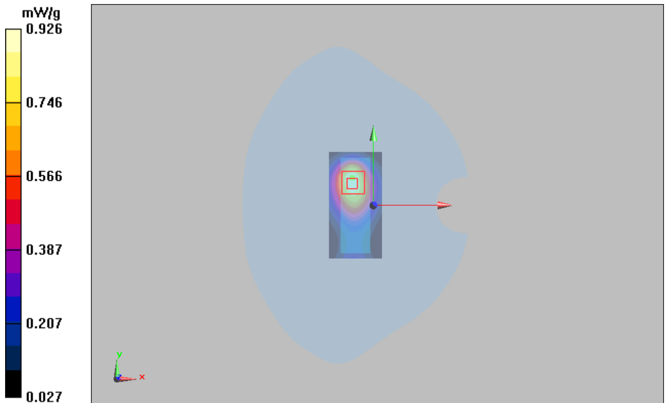
Figure 45 WCDMA Band V HSDPA with IBM T61 Test Position 2 Channel 4233
