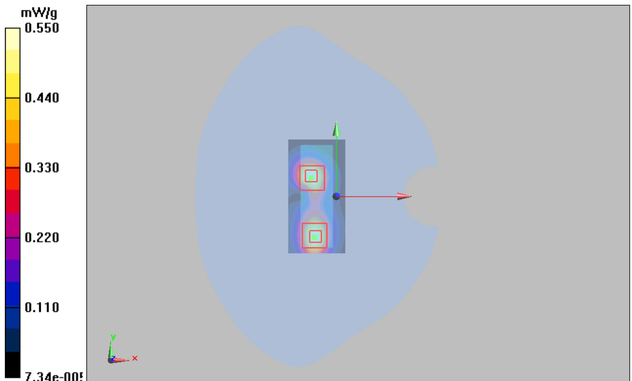
Figure 23 GSM 1900 GPRS (2Up) with IBM T61 Test Position 2 Channel 661
