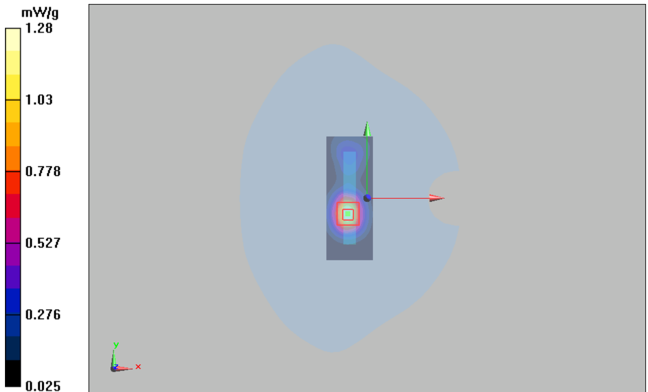
Figure 35 WCDMA Band II with Lenovo Y-450 Test Position 4 Channel 9538
