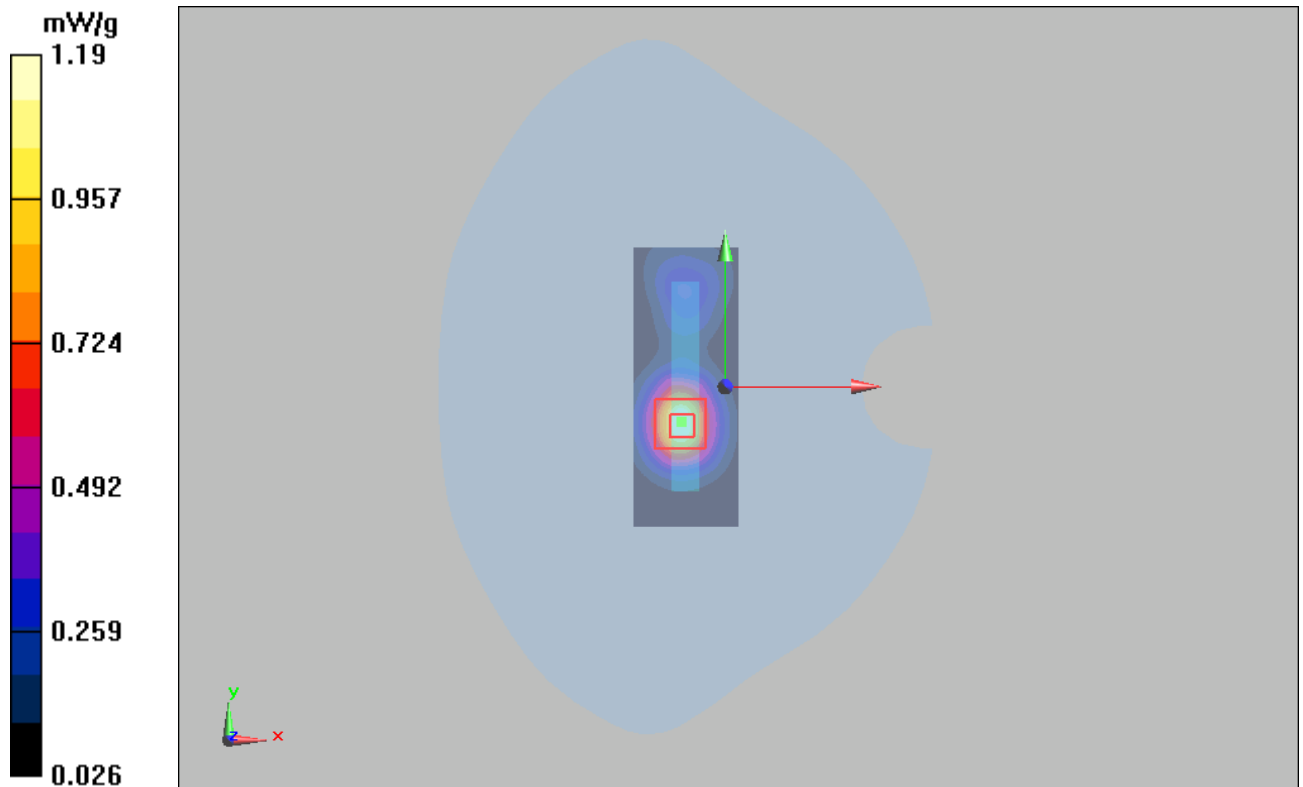
Figure 37 WCDMA Band II with Lenovo Y-450 Test Position 4 Channel 9262
