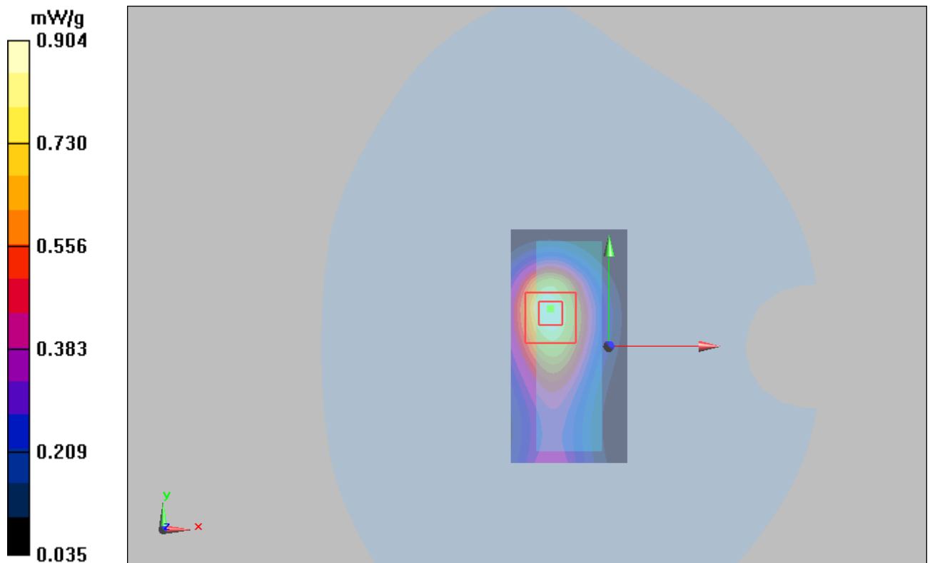
Figure 11 GSM 850 GPRS (2Up) with IBM T61 Test Position 2 Channel 190
