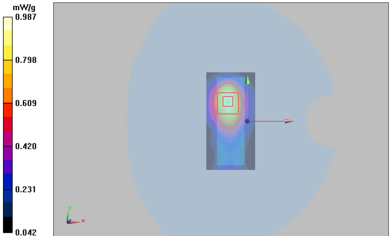
Figure 12 GSM 850 GPRS (2Up) with IBM T61 Test Position 2 Channel 128
