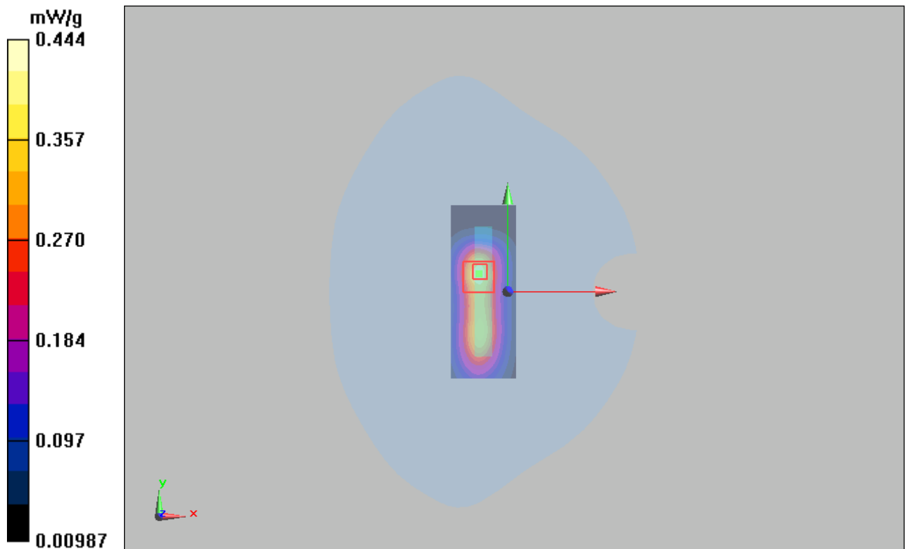
Figure 34 WCDMA Band II with Lenovo Y-450 Test Position 3 Channel 9400
