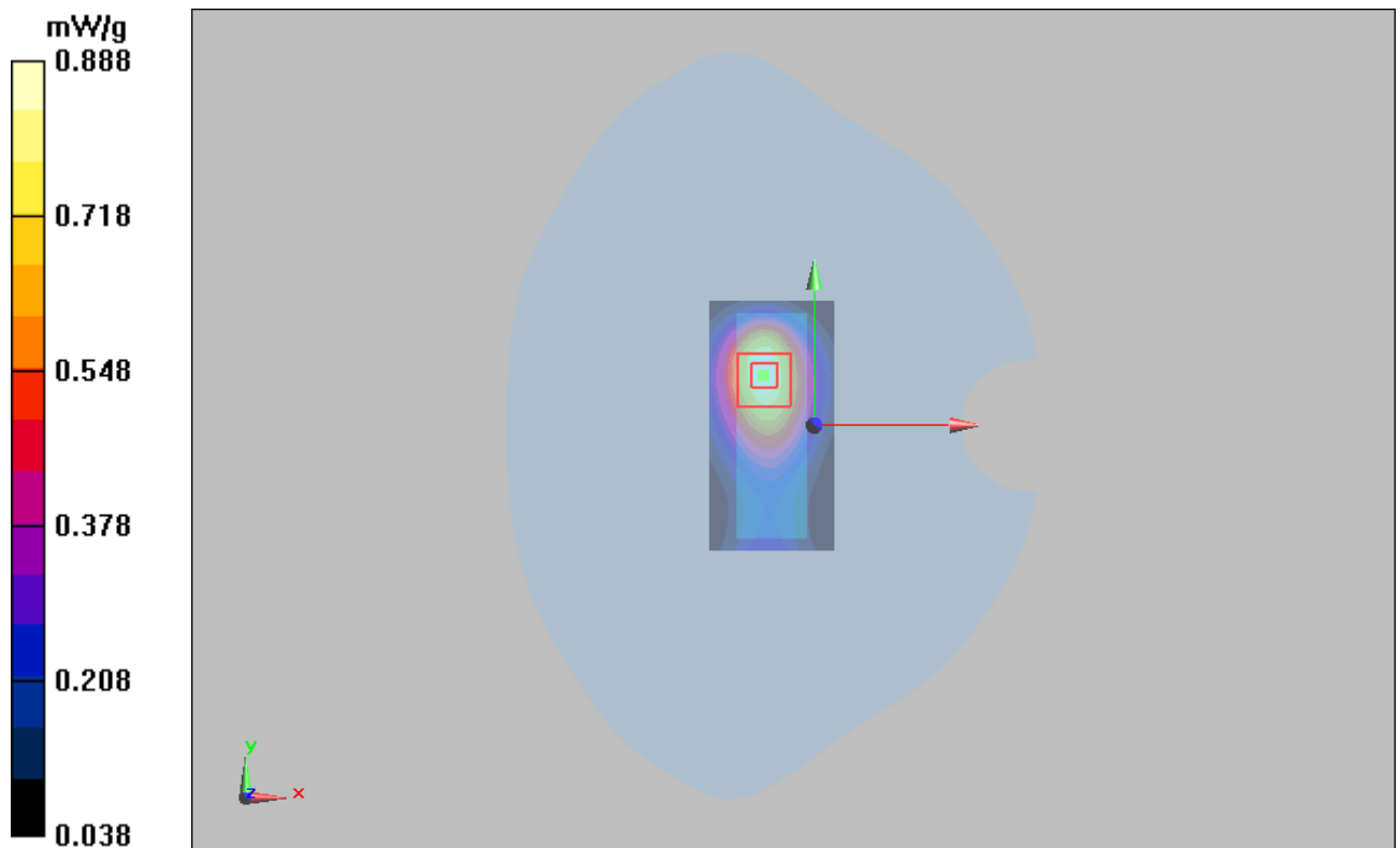
Figure 42 WCDMA Band V with IBM T61 Test Position 2 Channel 4132
