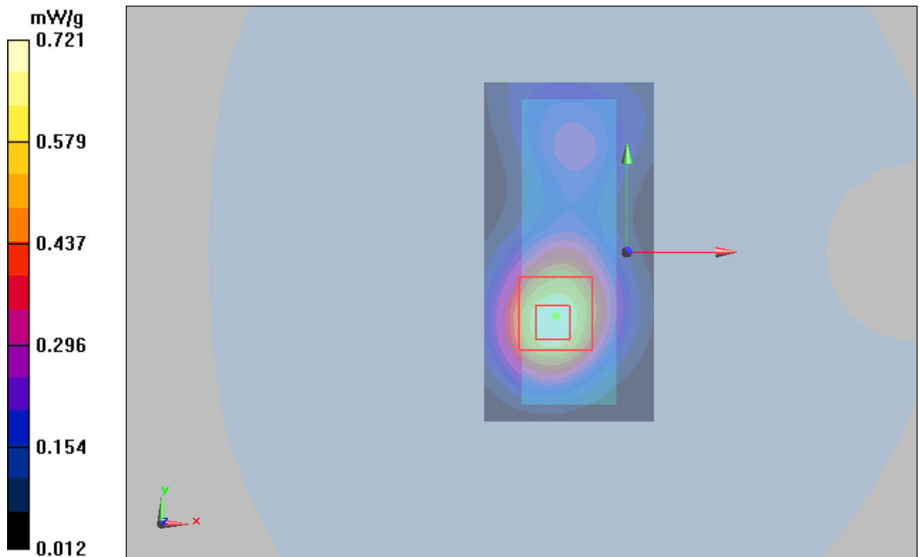
Figure 21 GSM 1900 GPRS (2Up) with IBM T61 Test Position 1 Channel 661
