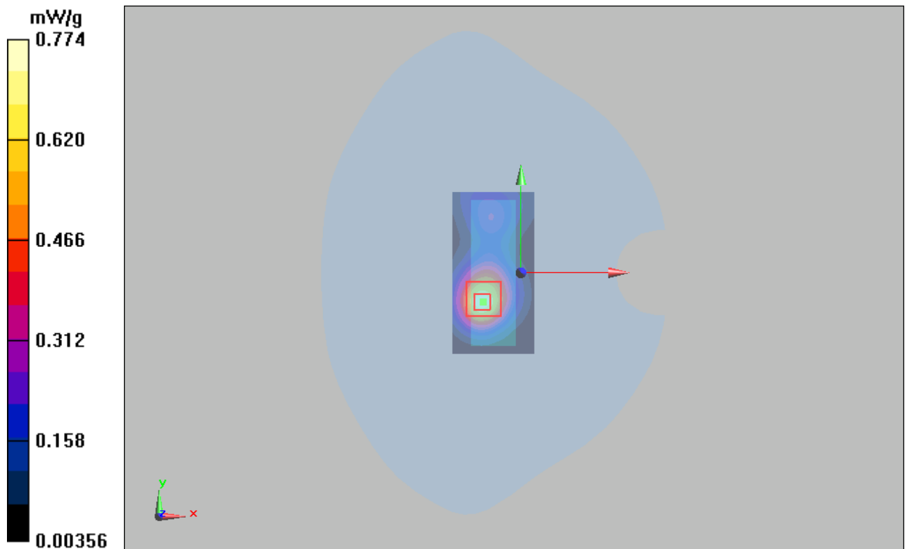
Figure 26 GSM 1900 EGPRS (1Up) with IBM T61 Test Position 1 Channel 512
