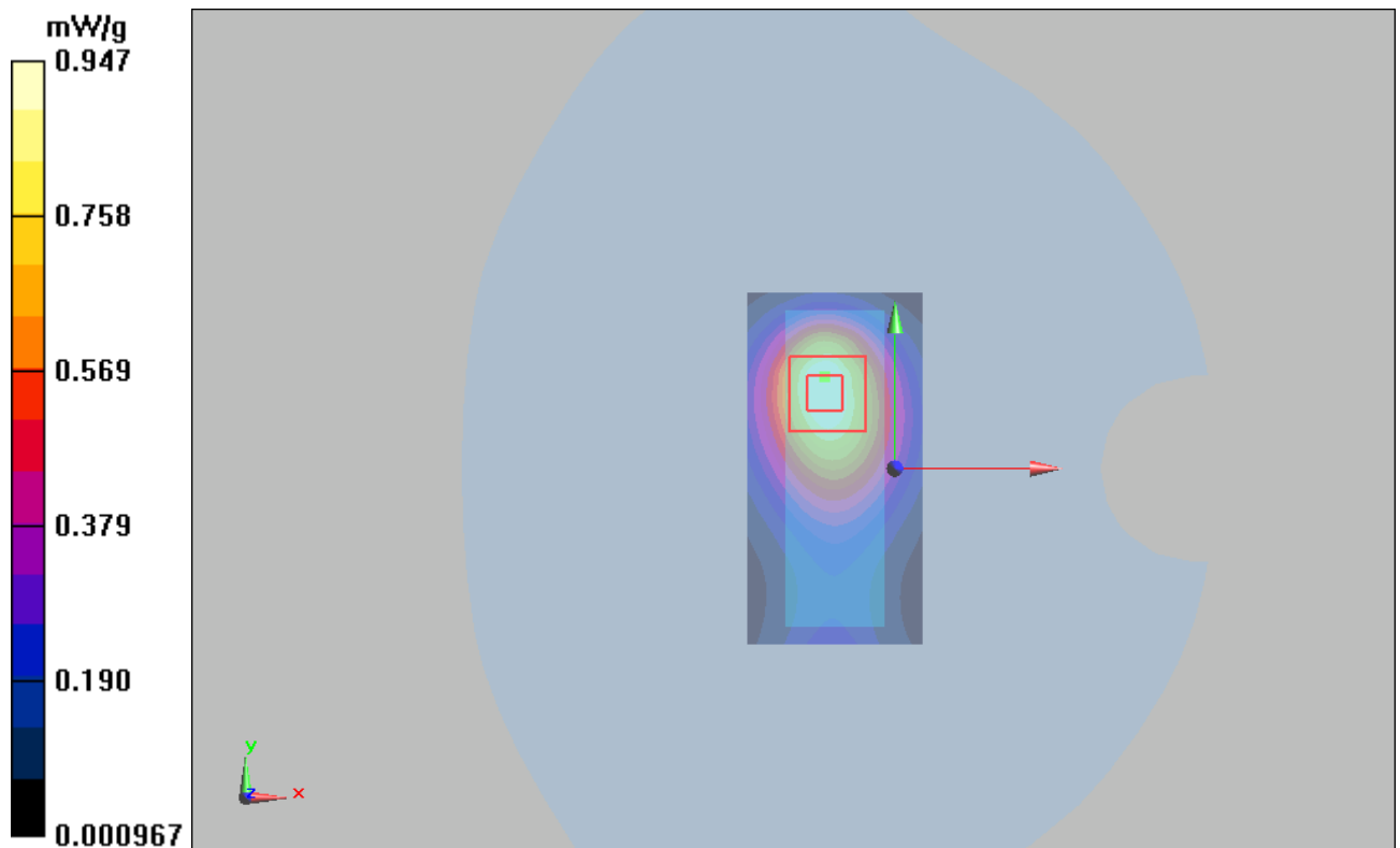
Figure 17 GSM 850 EGPRS (3Up) with IBM T61 Test Position 2 Channel 251
