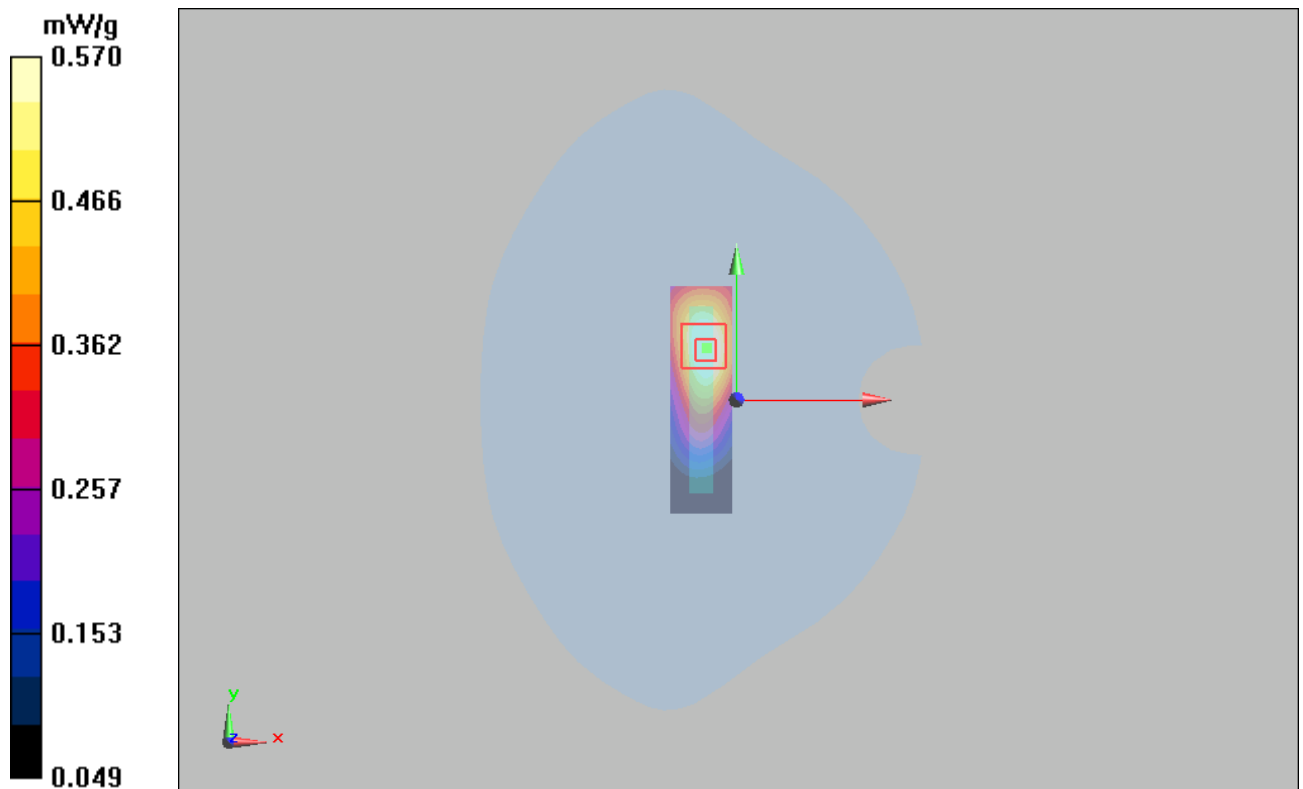
Figure 14 GSM 850 GPRS (2Up) with Lenovo Y-450 Test Position 4 Channel 190
