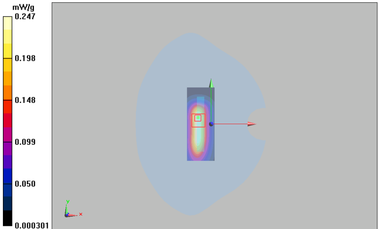
Figure 24 GSM 1900 GPRS (2Up) with Lenovo Y-450 Test Position 3 Channel 661
