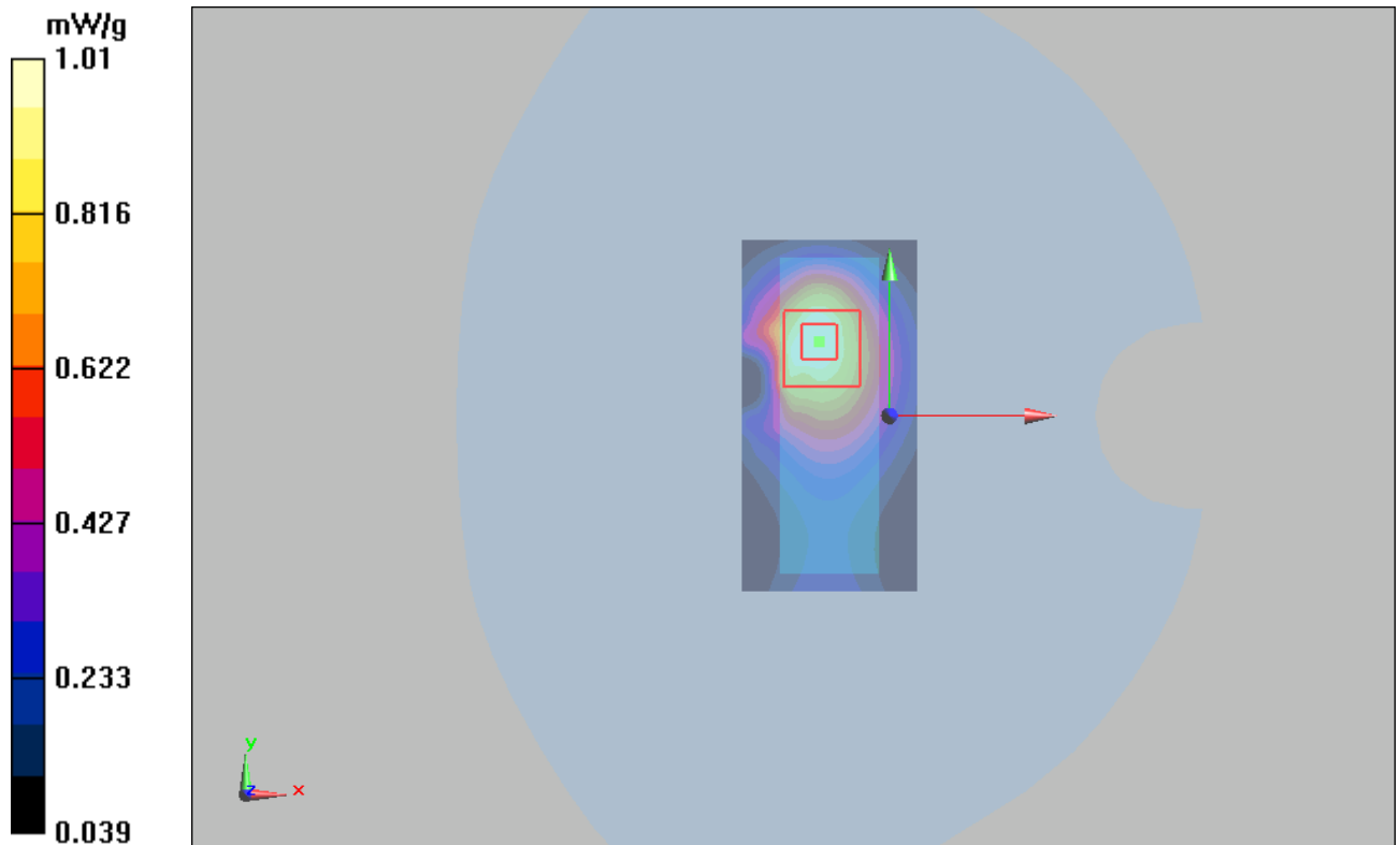
Figure 16 GSM 850 EGPRS (2Up) with IBM T61 Test Position 2 Channel 251
