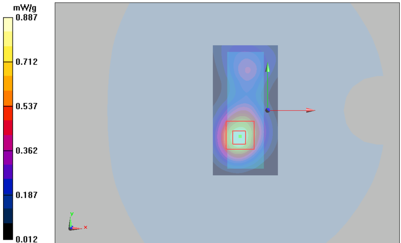
Figure 22 GSM 1900 GPRS (2Up) with IBM T61 Test Position 1 Channel 512
