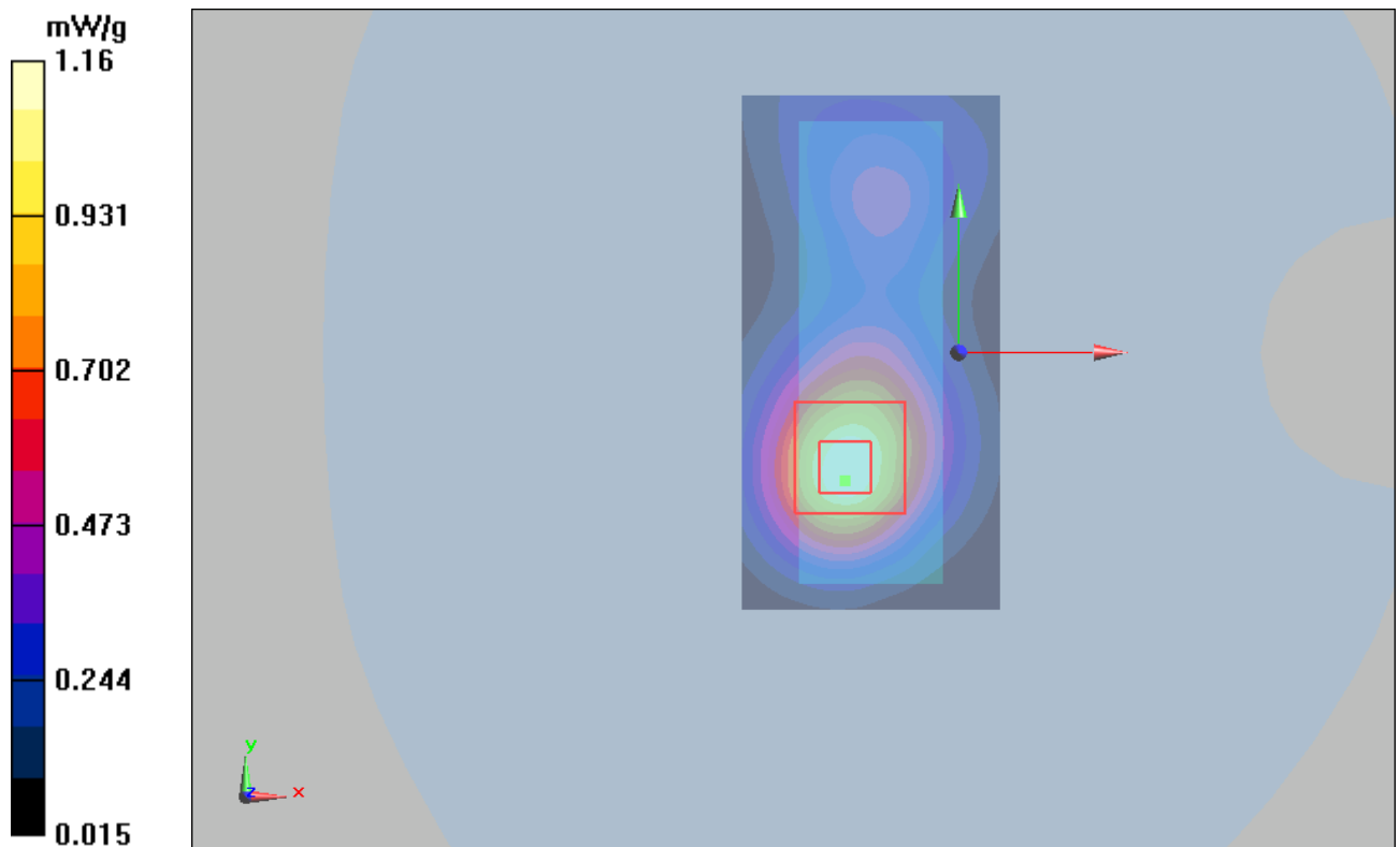
Figure 31 WCDMA Band II with IBM T61 Test Position 1 Channel 9400
