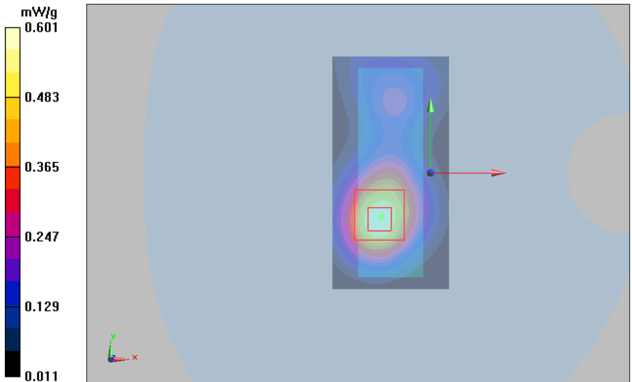
Figure 20 GSM 1900 GPRS (2Up) with IBM T61 Test Position 1 Channel 810
