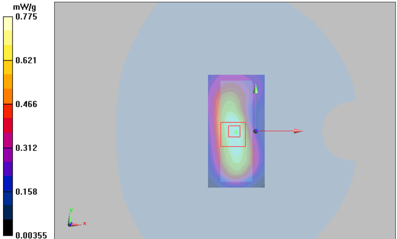
Figure 9 GSM 850 GPRS (2Up) with IBM T61 Test Position 1 Channel 190
