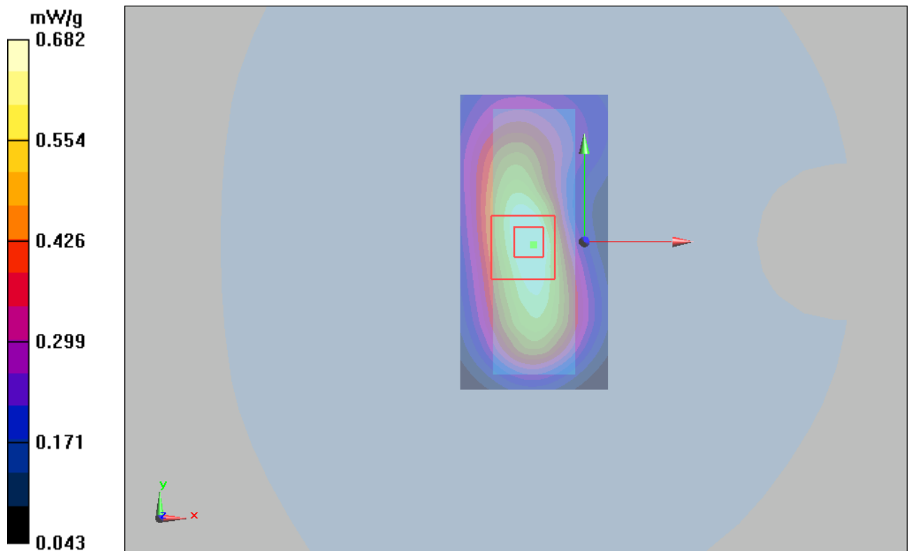
Figure 39 WCDMA Band V with IBM T61 Test Position 1 Channel 4183
