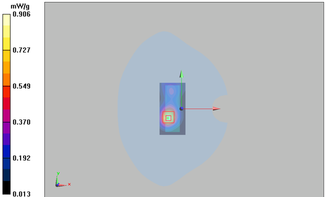
Figure 27 GSM 1900 EGPRS (2Up) with IBM T61 Test Position 1 Channel 512
