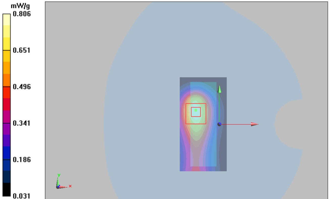
Figure 41 WCDMA Band V with IBM T61 Test Position 2 Channel 4183
