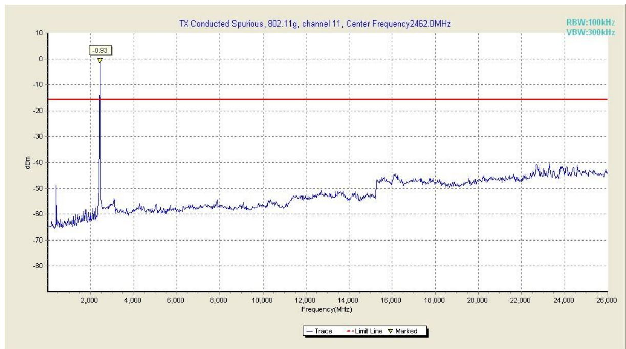
Fig. 28 Conducted Spurious Emission (802.11g, Ch11, 30 MHz-26 GHz)
