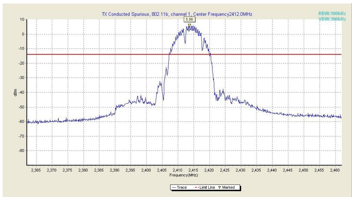
Fig. 17 Conducted Spurious Emission (802.11b, Ch1, Center Frequency)
