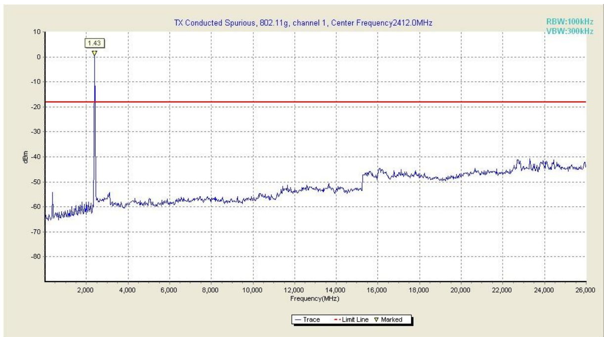
Fig. 24 Conducted Spurious Emission (802.11g, Ch1, 30 MHz-26 GHz)
