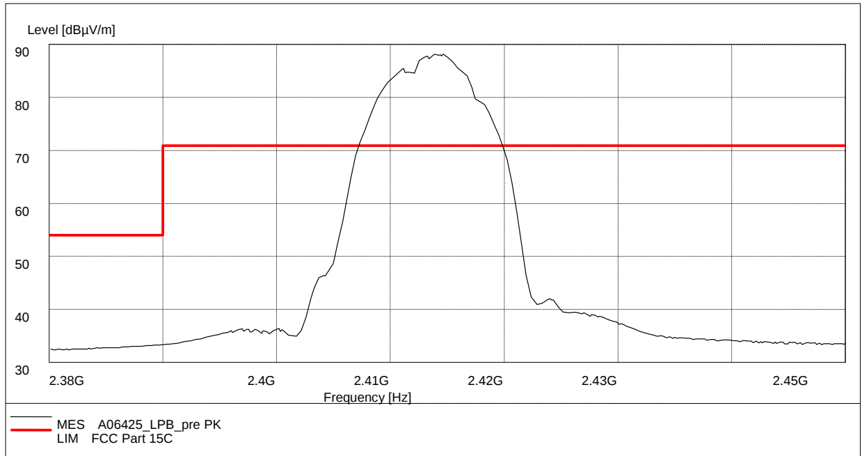
Fig. 29 Radiated Spurious Emission (Power): 802.11b, ch1, 2.38 GHz - 245GHz
