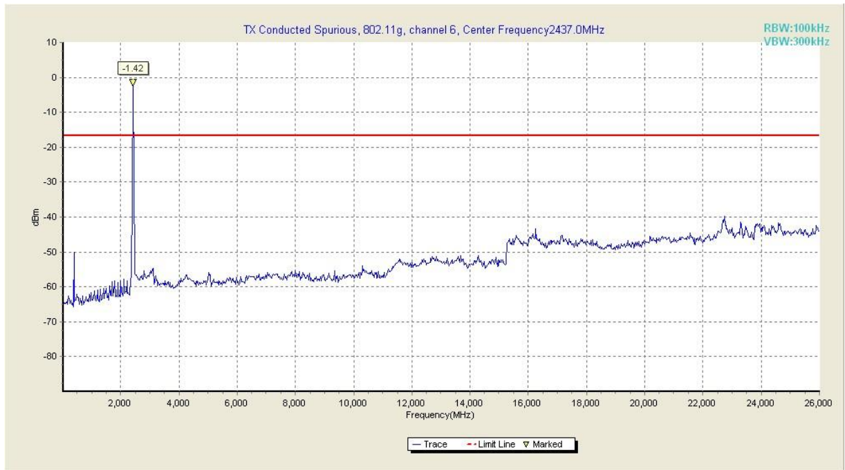
Fig. 26 Conducted Spurious Emission (802.11g, Ch6, 30 MHz-26 GHz)
