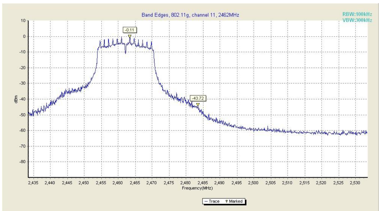
Fig. 16 Band Edges (802.11g, Ch 11)
