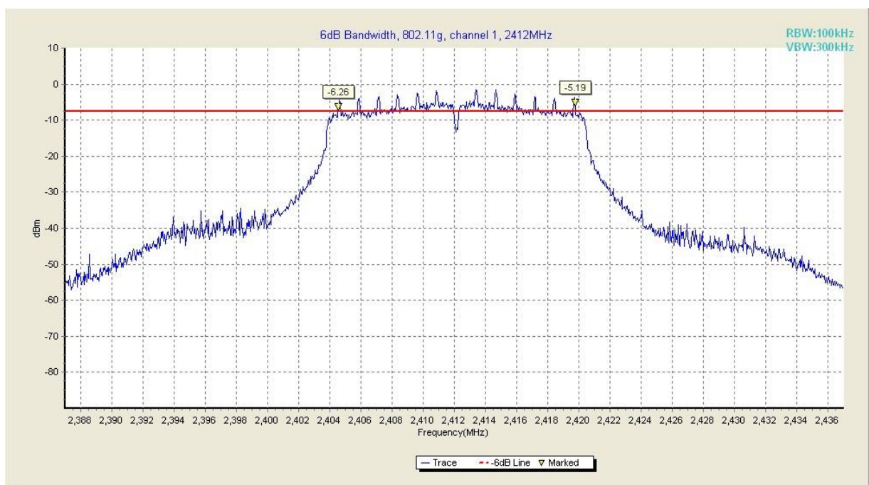
Fig. 10 Occupied 6dB Bandwidth (802.11g, Ch 1)
