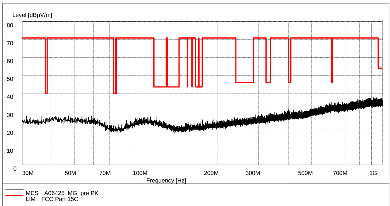
Fig. 44 Radiated Spurious Emission (802.11g, Ch6, 30 MHz-1 GHz)
