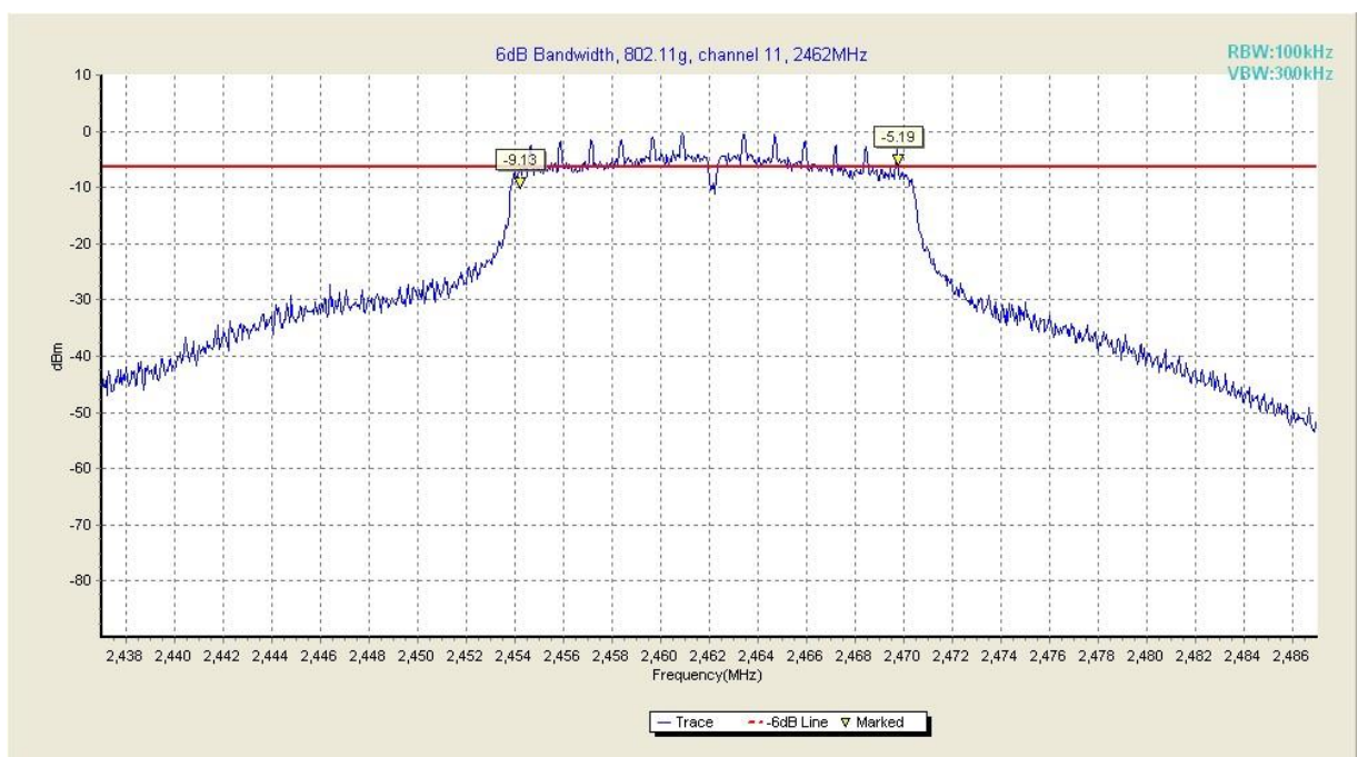
Fig. 12 Occupied 6dB Bandwidth (802.11g, Ch 11)
