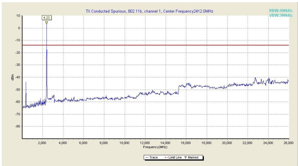
Fig. 18 Conducted Spurious Emission (802.11b, Ch1, 30 MHz-26 GHz)
