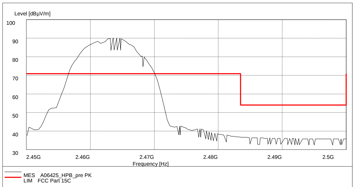
Fig. 36 Radiated Spurious Emission (Power): 802.11b, ch11, 2.45 GHz - 2.50GHz
