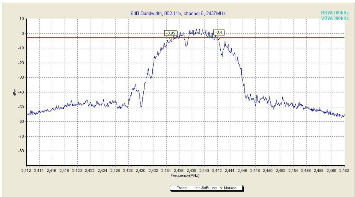
Fig. 8 Occupied 6dB Bandwidth (802.11b, Ch 6)
