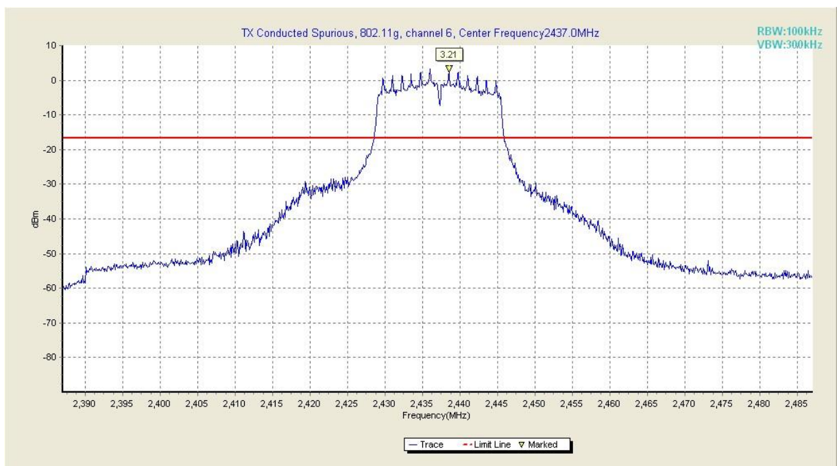
Fig. 25 Conducted Spurious Emission (802.11g, Ch6, Center Frequency)
