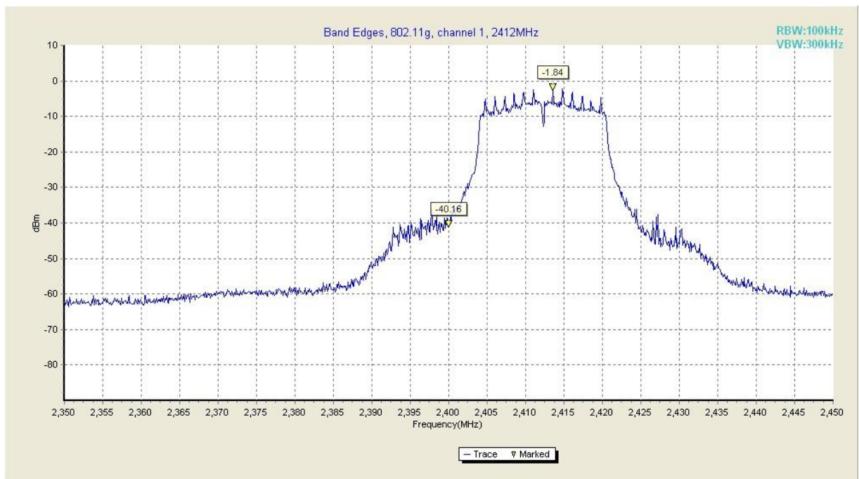
Fig. 15 Band Edges (802.11g, Ch 1)
