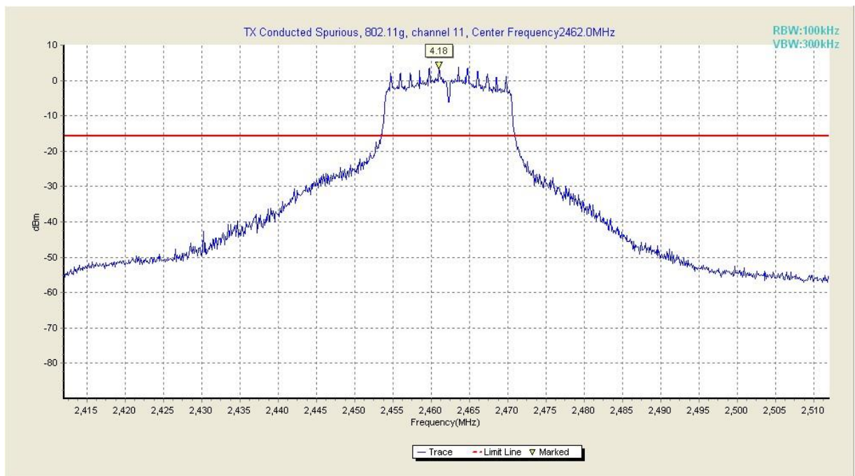
Fig. 27 Conducted Spurious Emission (802.11g, Ch11, Center Frequency)
