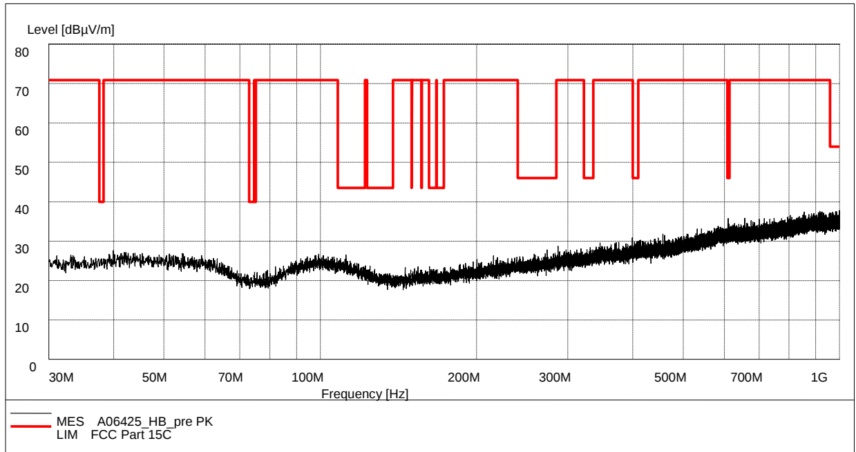
Fig. 37 Radiated Spurious Emission (802.11b, Ch11, 30 MHz-1 GHz)
