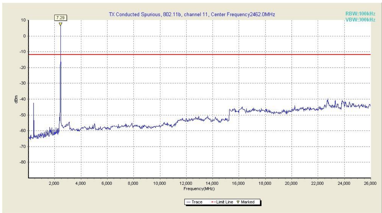
Fig. 22 Conducted Spurious Emission (802.11b, Ch11, 30 MHz-26 GHz)
