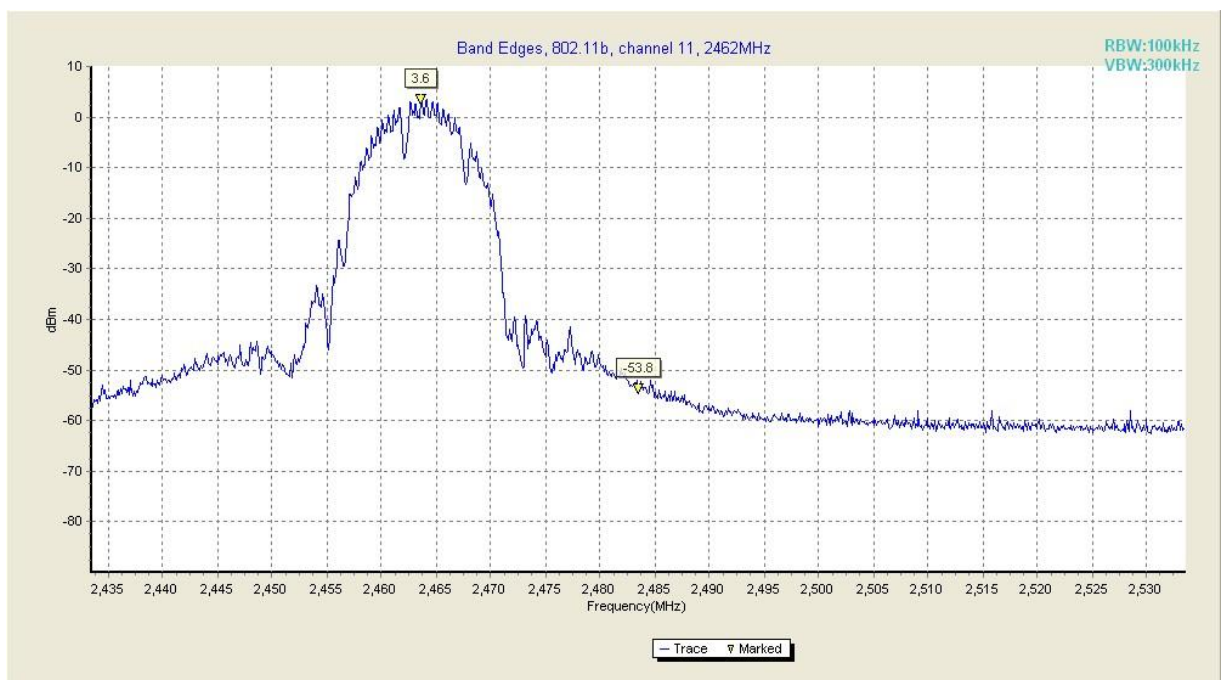
Fig. 14 Band Edges (802.11b, Ch 11)
