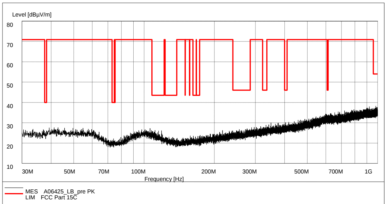
Fig. 30 Radiated Spurious Emission (802.11b, Ch1, 30 MHz-1 GHz)
