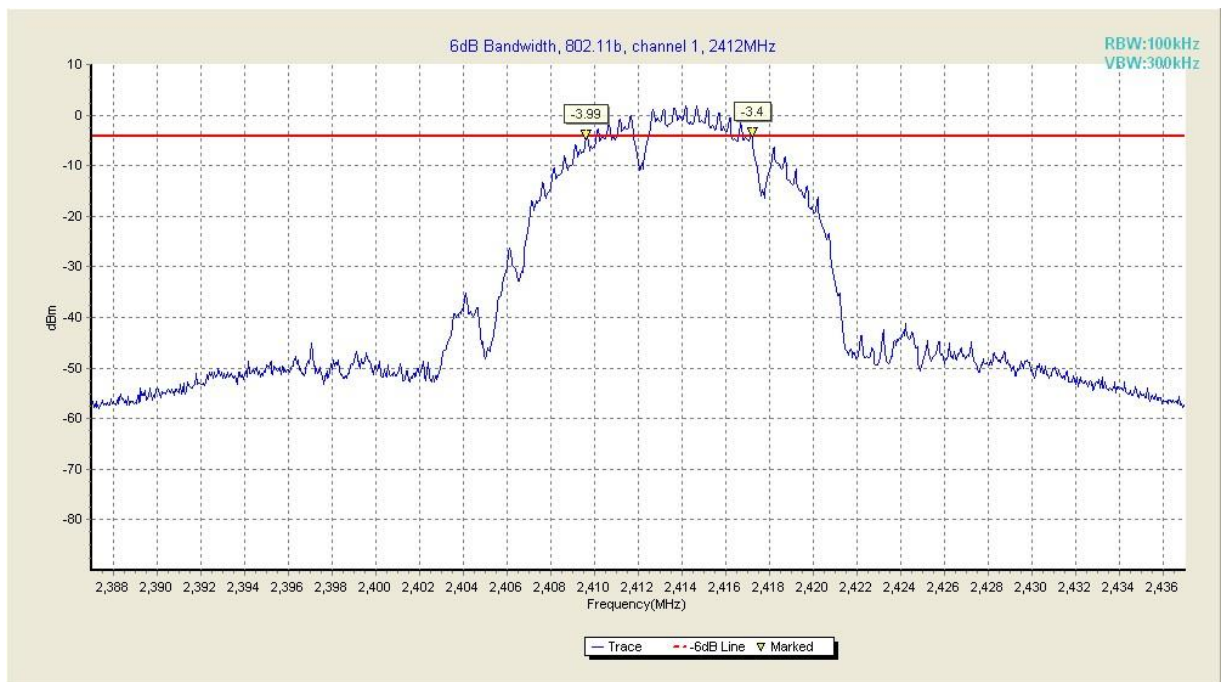
Fig. 7 Occupied 6dB Bandwidth (802.11b, Ch 1)
