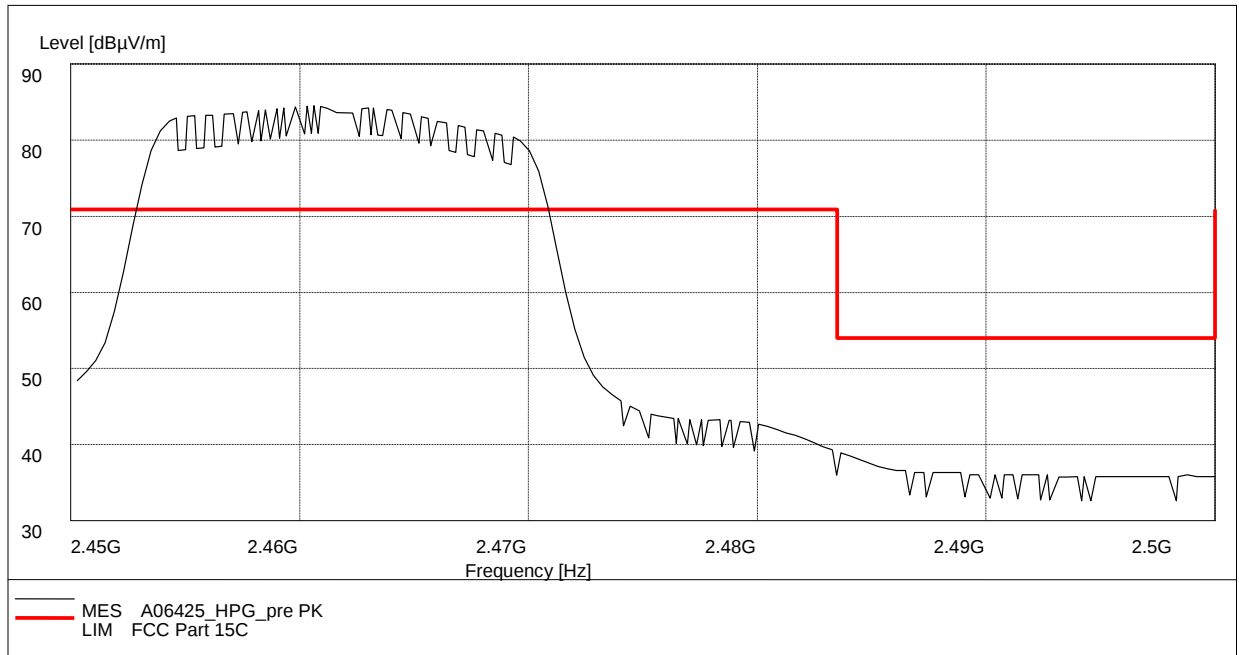
Fig. 47 Radiated Spurious Emission (Power): 802.11g, ch11, 2.45 GHz - 2.50GHz
