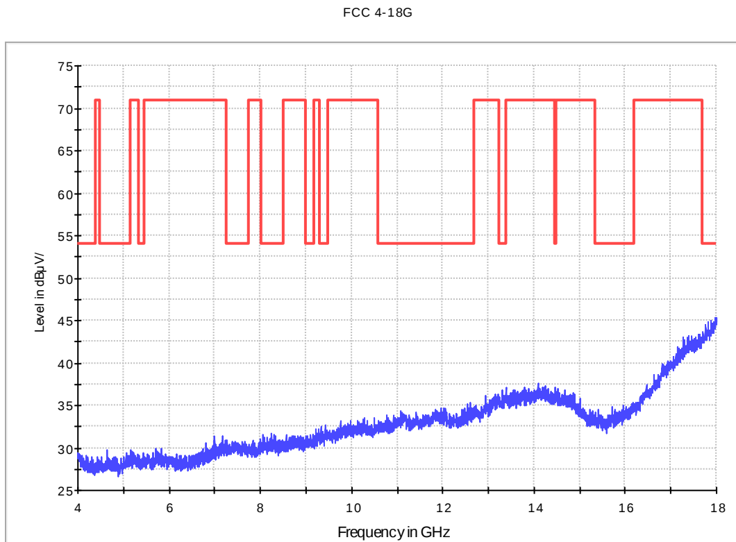
Fig. 50 Radiated Spurious Emission (802.11g, Ch11, 4 GHz-18 GHz)
