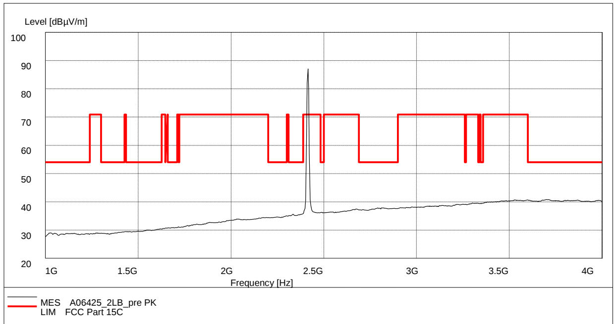
Fig. 31 Radiated Spurious Emission (802.11b, Ch1, 1 GHz-4 GHz)
