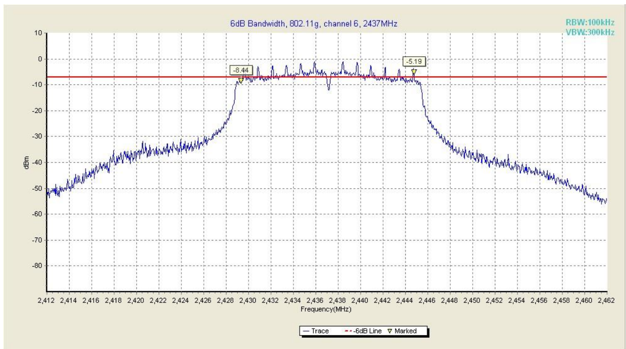
Fig. 11 Occupied 6dB Bandwidth (802.11g, Ch 6)
