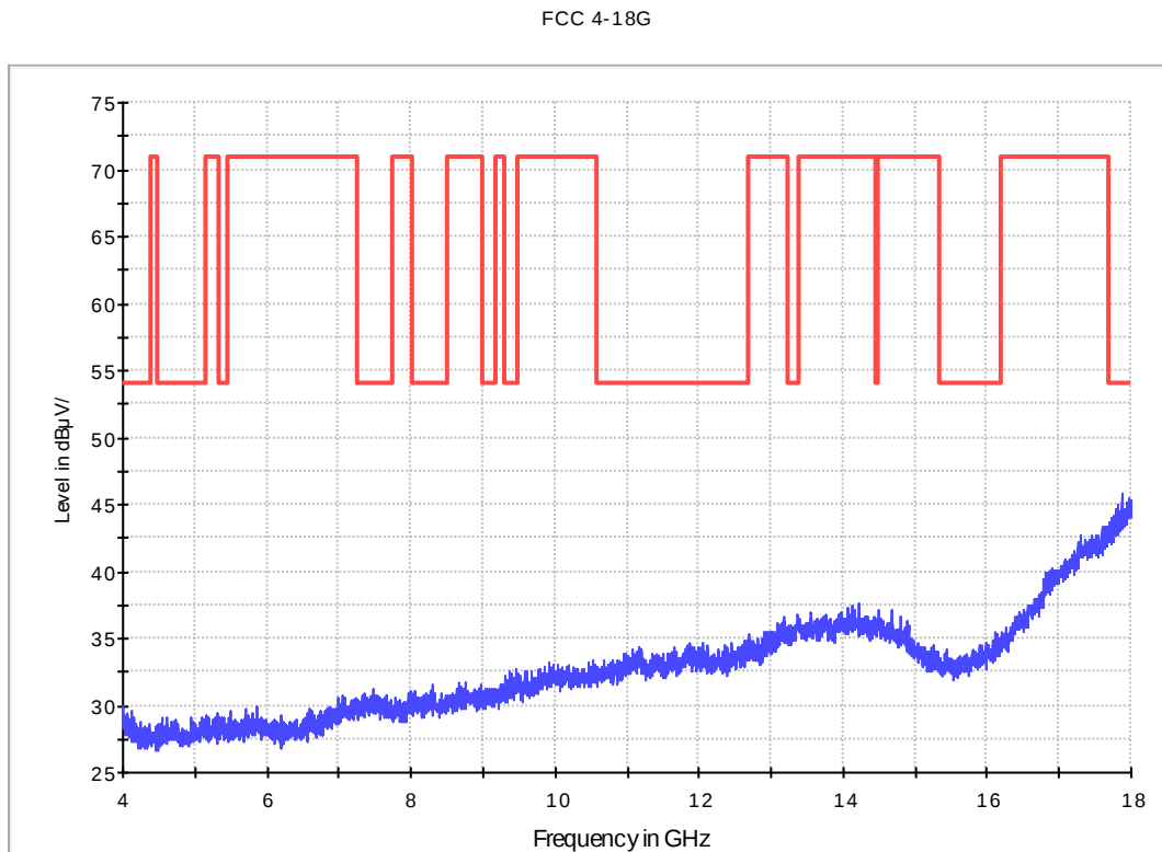
Fig. 43 Radiated Spurious Emission (802.11g, Ch1, 4 GHz-18 GHz)
