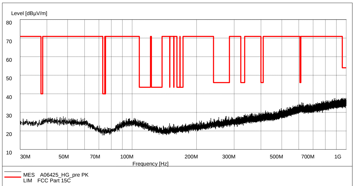
Fig. 48 Radiated Spurious Emission (802.11g, Ch11, 30 MHz-1 GHz)
