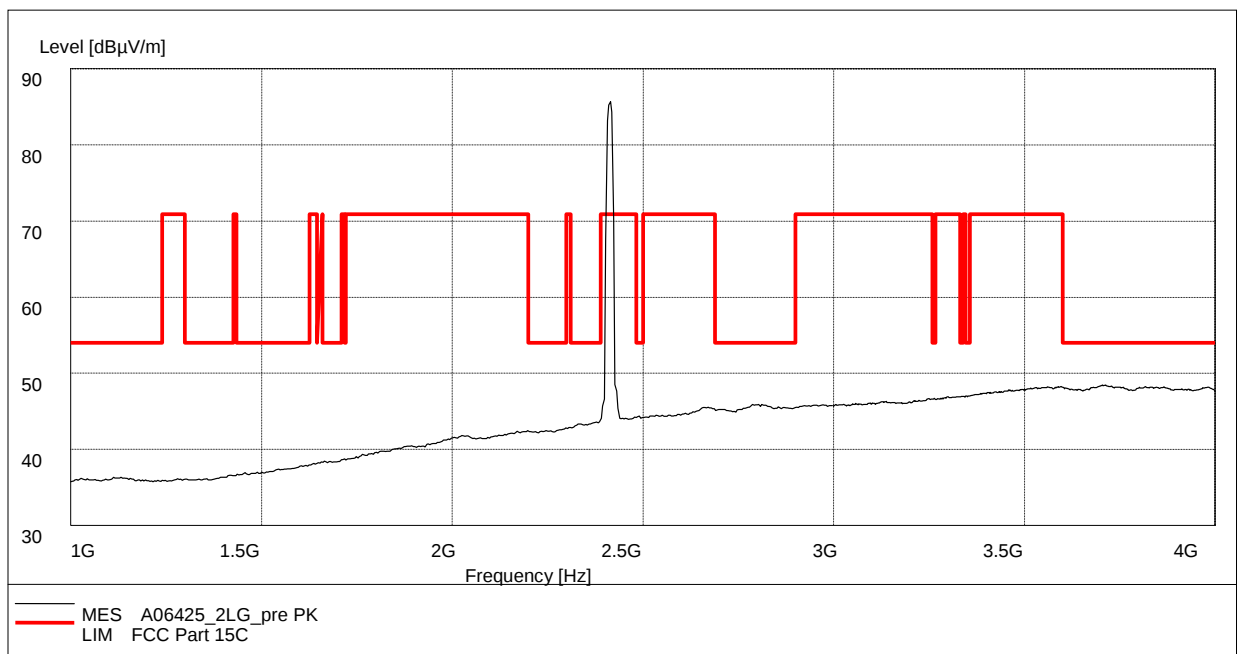
Fig. 42 Radiated Spurious Emission (802.11g, Ch1, 1 GHz-4 GHz)
