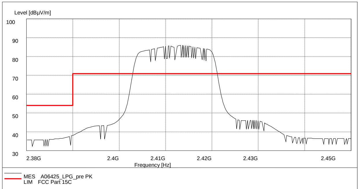
Fig. 40 Radiated Spurious Emission (Power): 802.11g, ch1, 2.38 GHz - 2.45GHz
