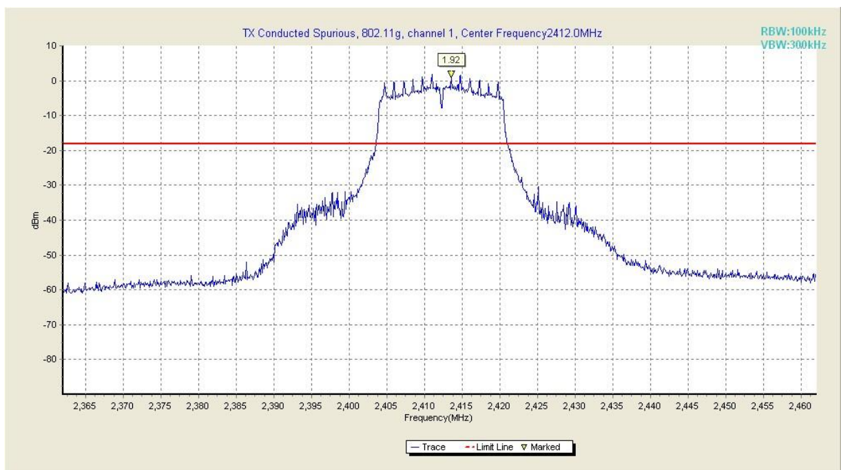
Fig. 23 Conducted Spurious Emission (802.11g, Ch1, Center Frequency)
