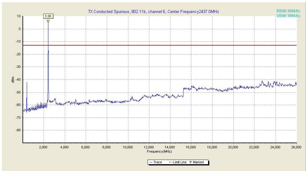
Fig. 20 Conducted Spurious Emission (802.11b, Ch6, 30 MHz-26 GHz)
