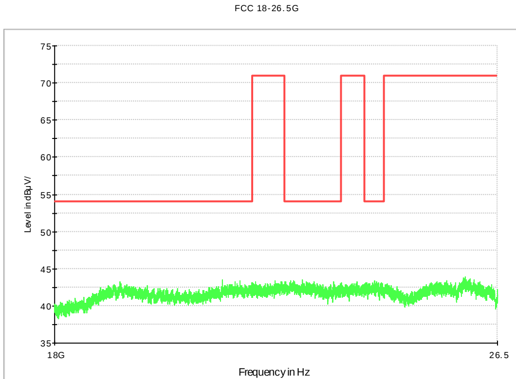
Fig. 51 Radiated emission: 18 GHz - 26.5 GHz
