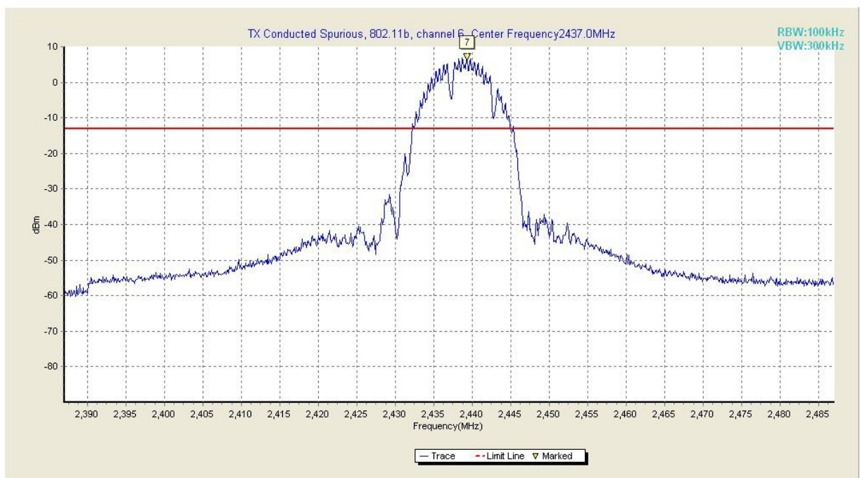
Fig. 19 Conducted Spurious Emission (802.11b, Ch6, Center Frequency)
