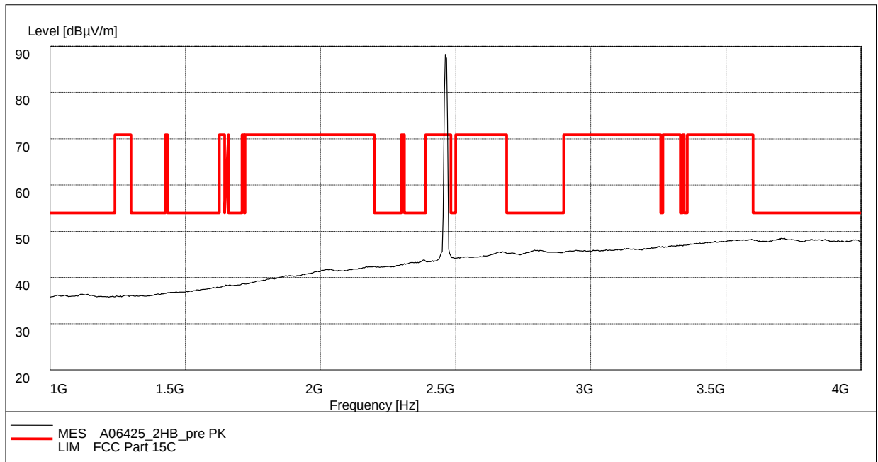
Fig. 38 Radiated Spurious Emission (802.11b, Ch11, 1 GHz-4 GHz)
