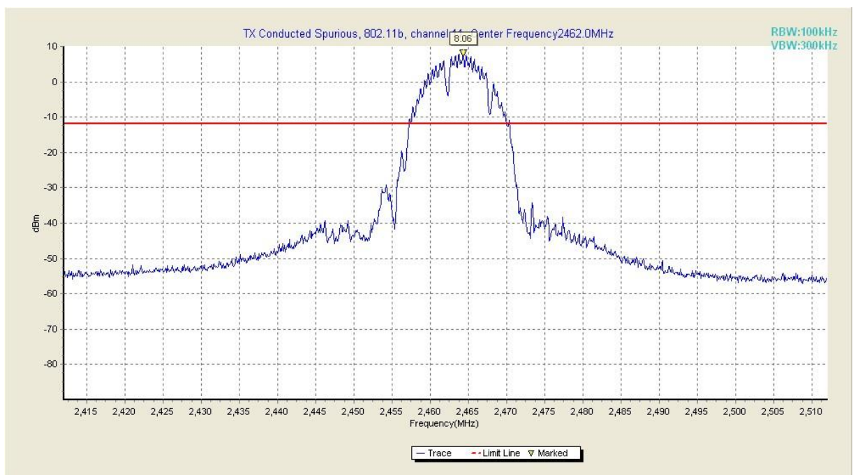
Fig. 21 Conducted Spurious Emission (802.11b, Ch11, Center Frequency)
