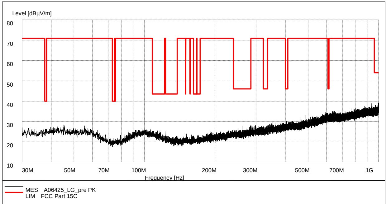
Fig. 41 Radiated Spurious Emission (802.11g, Ch1, 30 MHz-1 GHz)
