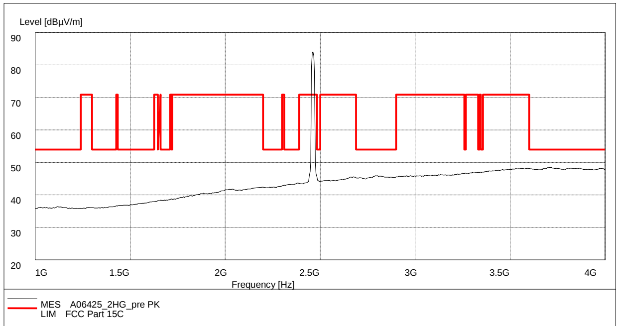
Fig. 49 Radiated Spurious Emission (802.11g, Ch11, 1 GHz-4 GHz)
