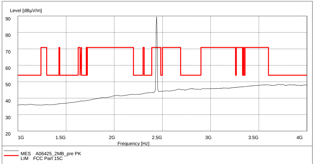
Fig. 34 Radiated Spurious Emission (802.11b, Ch6, 1 GHz-4 GHz)
