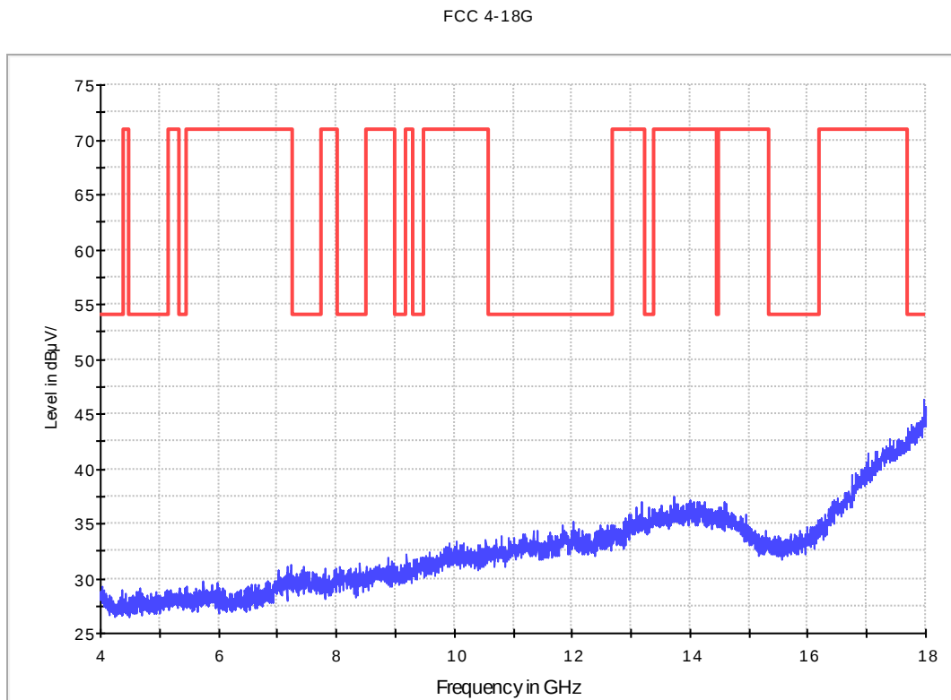
Fig. 32 Radiated Spurious Emission (802.11b, Ch1, 4 GHz-18 GHz)
