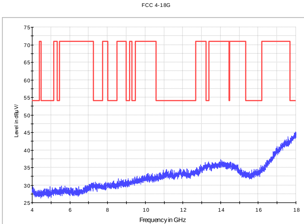
Fig. 46 Radiated Spurious Emission (802.11g, Ch6, 4 GHz-18 GHz)
