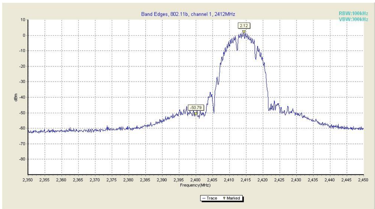
Fig. 13 Band Edges (802.11b, Ch 1)
