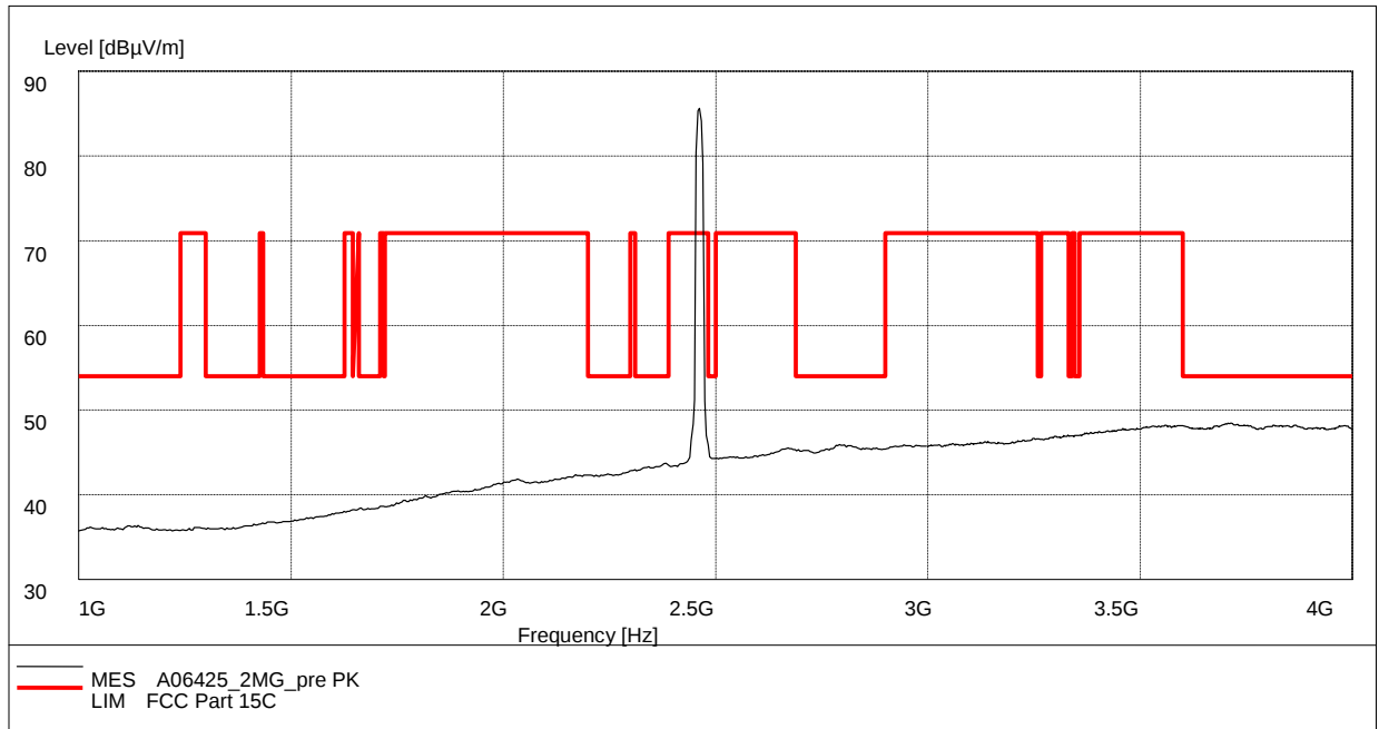
Fig. 45 Radiated Spurious Emission (802.11g, Ch6, 1 GHz-4 GHz)
