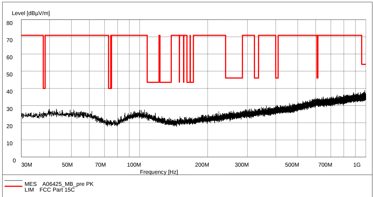
Fig. 33 Radiated Spurious Emission (802.11b, Ch6, 30 MHz-1 GHz)
