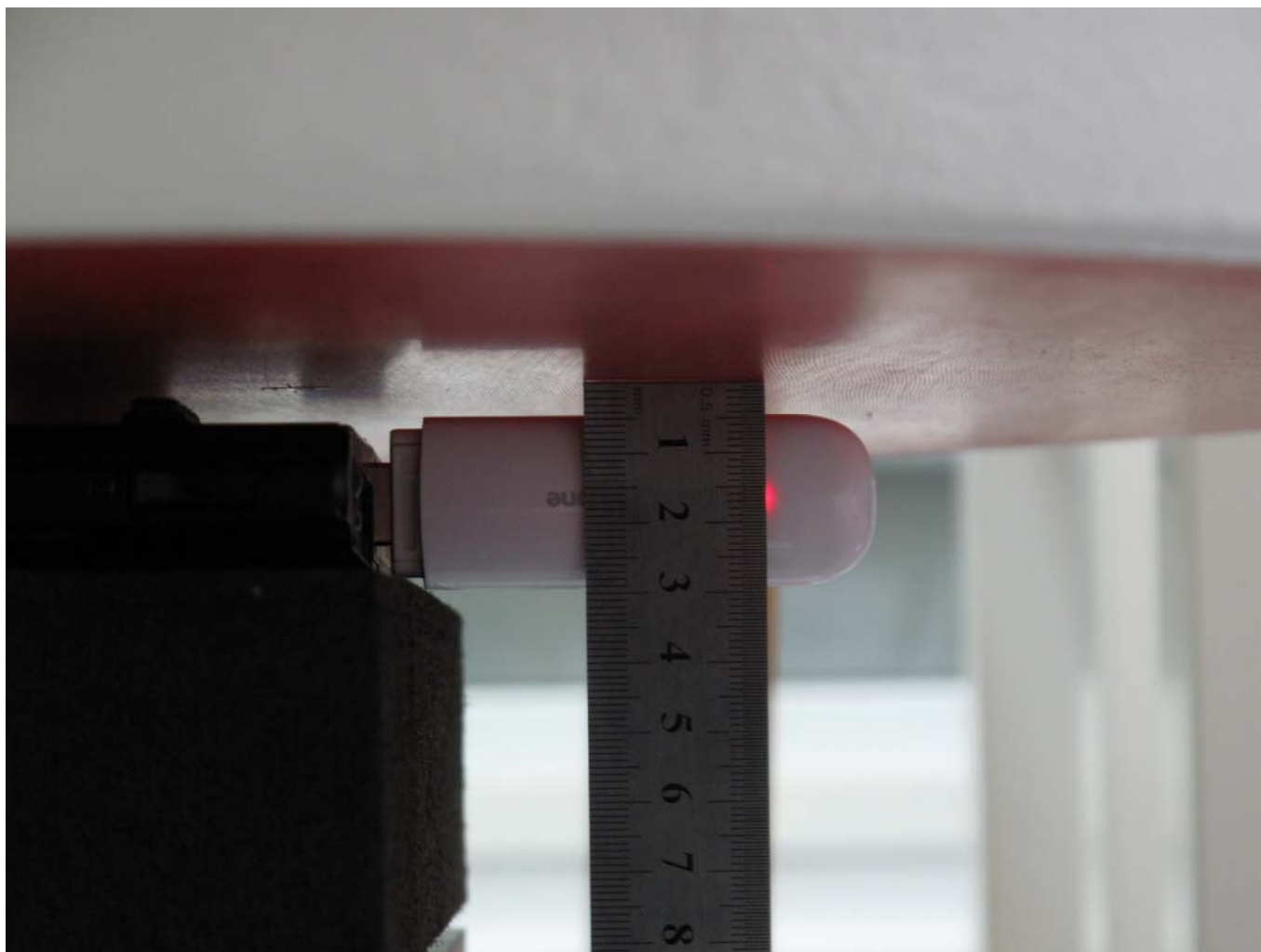
Face 3 to phantom (vertical side) with laptop
