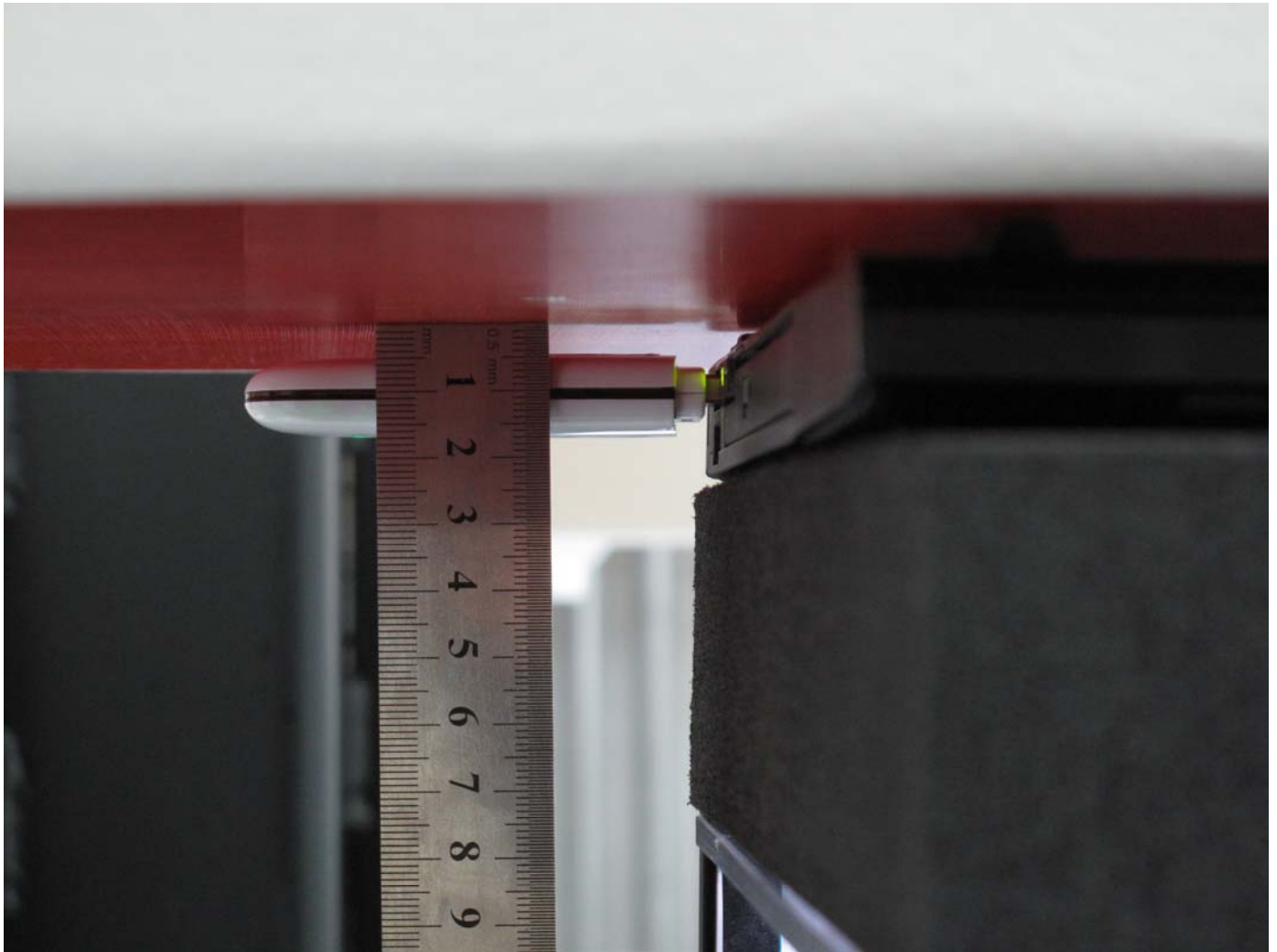
Face 2 to phantom (horizontal-up side) with laptop
