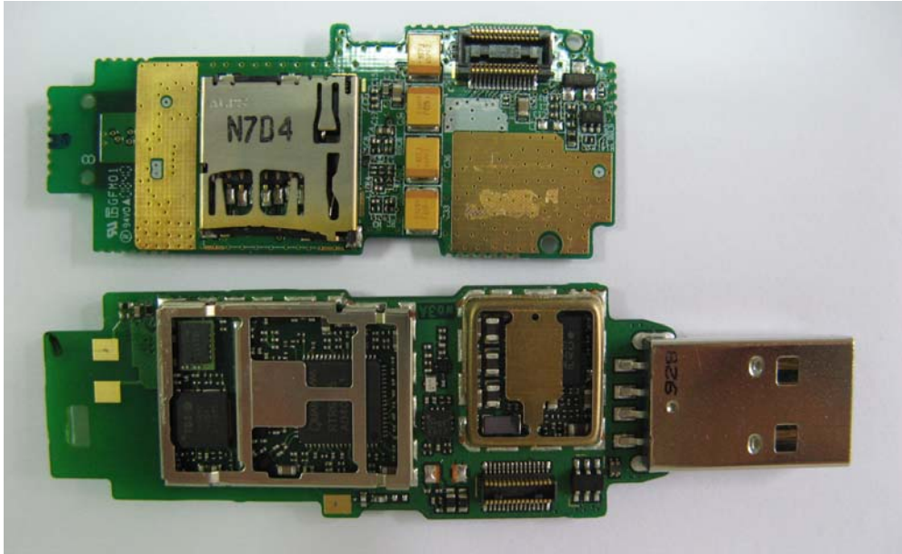
Picture 4: The sample with the shielding cover removed-2
