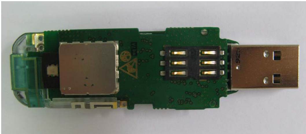
Picture 1: the top view of the PCB
