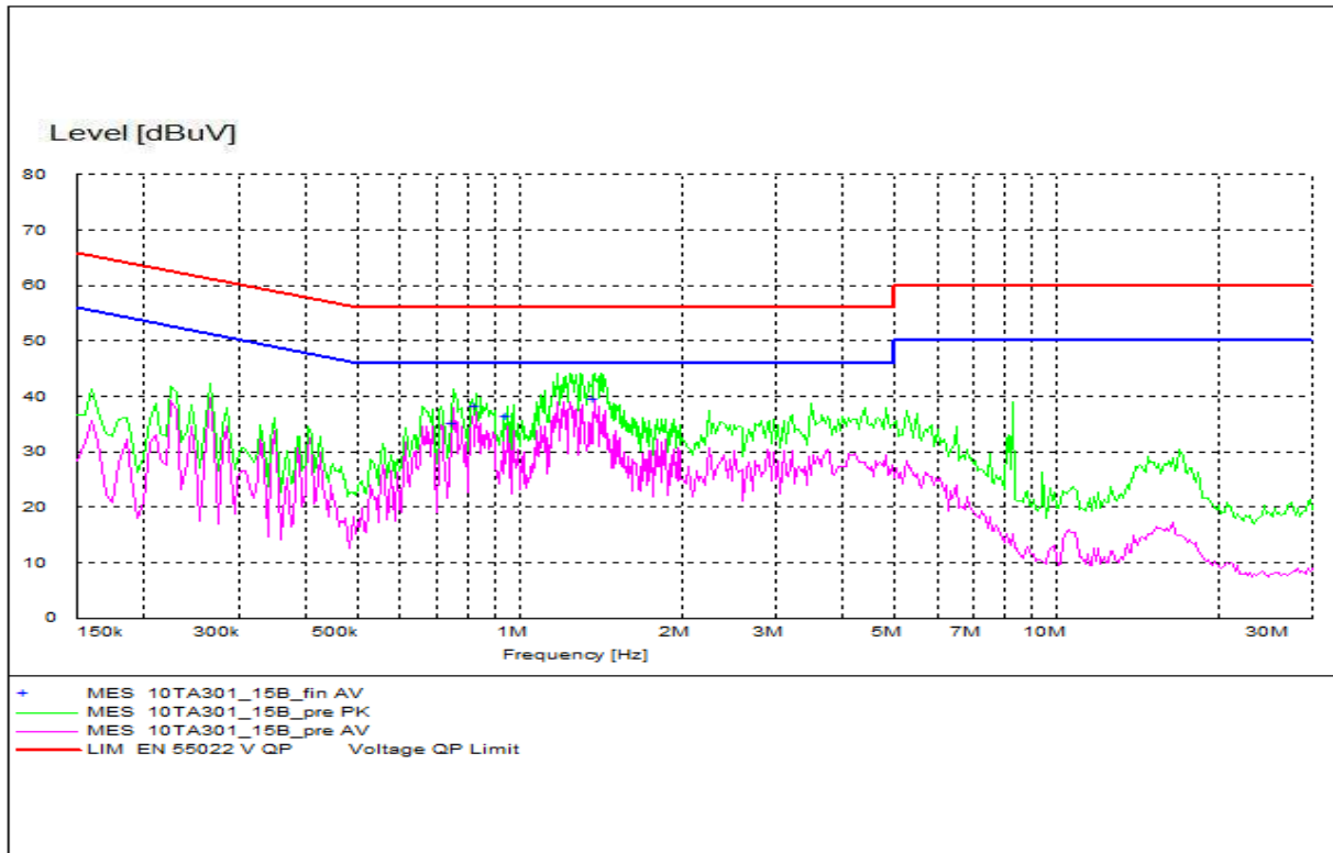
Figure A.3 Conducted Emission
