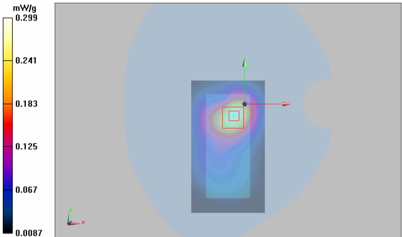
Figure 34 Body with Earphone, Towards Phantom, GSM 1900 Channel 512
