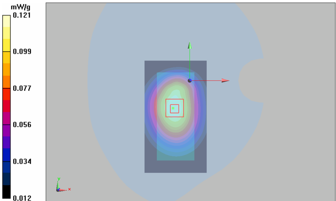
Figure 17 Body, Towards Ground, GSM 850 Channel 251
