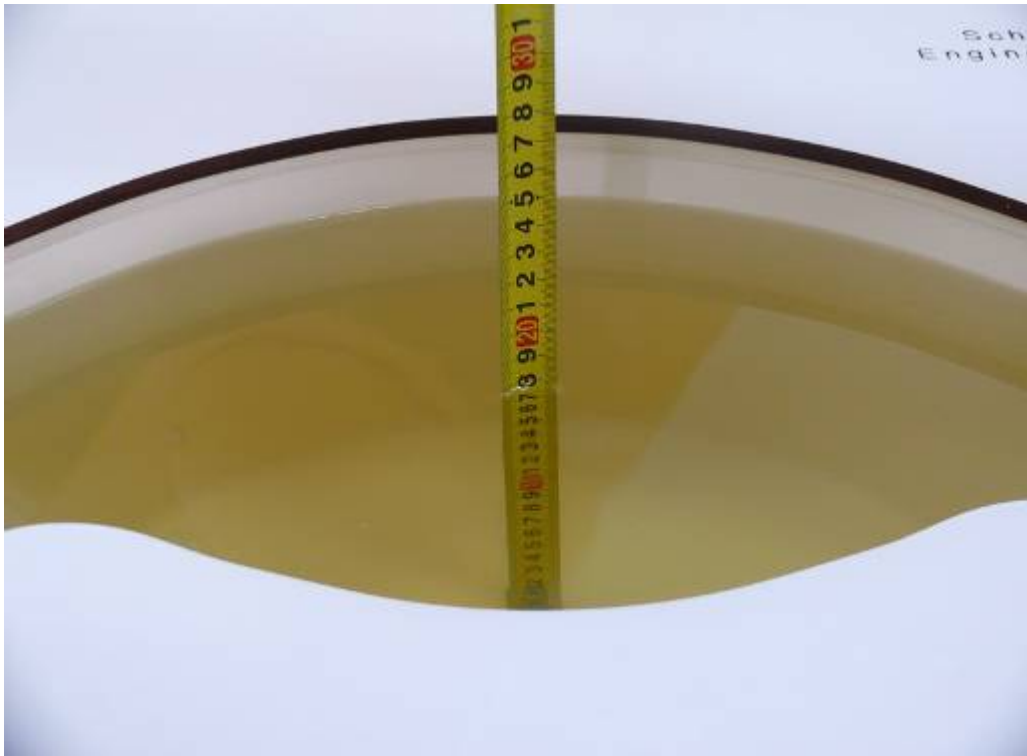
Picture 2: Liquid depth in the flat Phantom (835MHz) (17.5cm deep)
