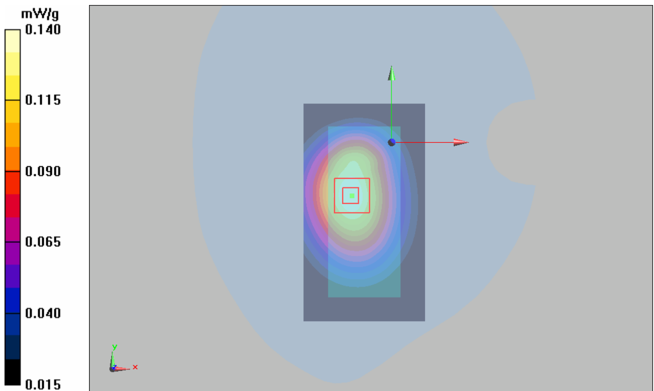
Figure 18 Body, Towards Ground, GSM 850 Channel 190
