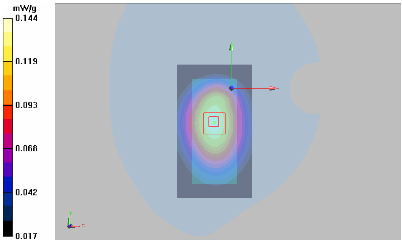
Figure 21 Body with Earphone, Towards Ground, GSM 850 Channel 128
