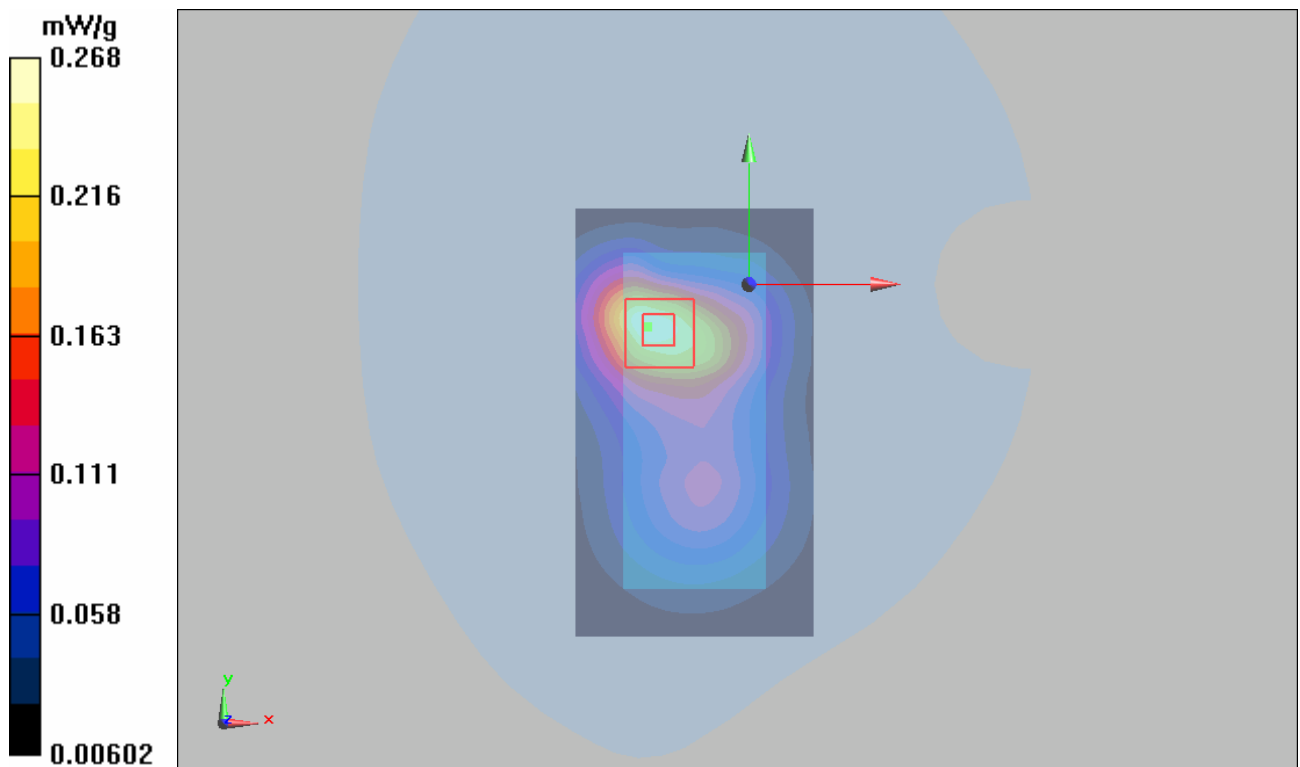
Figure 30 Body, Towards Ground, GSM 1900 Channel 661
