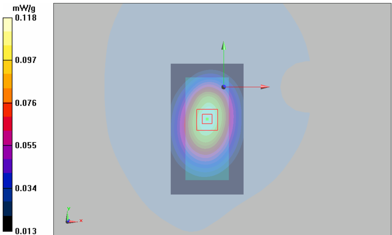
Figure 20 Body, Towards Phantom, GSM 850 Channel 190
