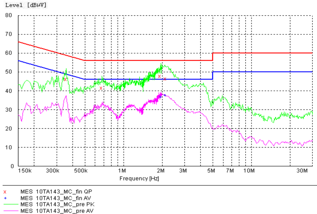
Figure A.5 Conducted Emission
