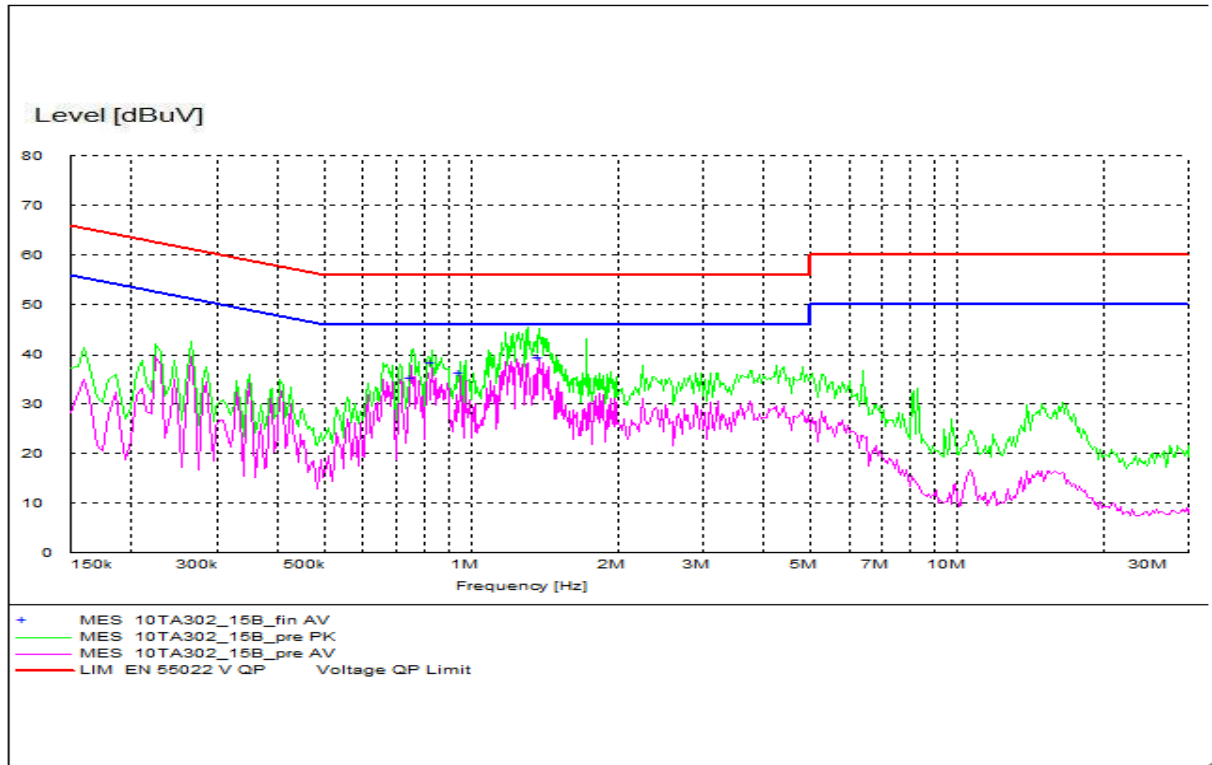
Figure A.6 Conducted Emission
