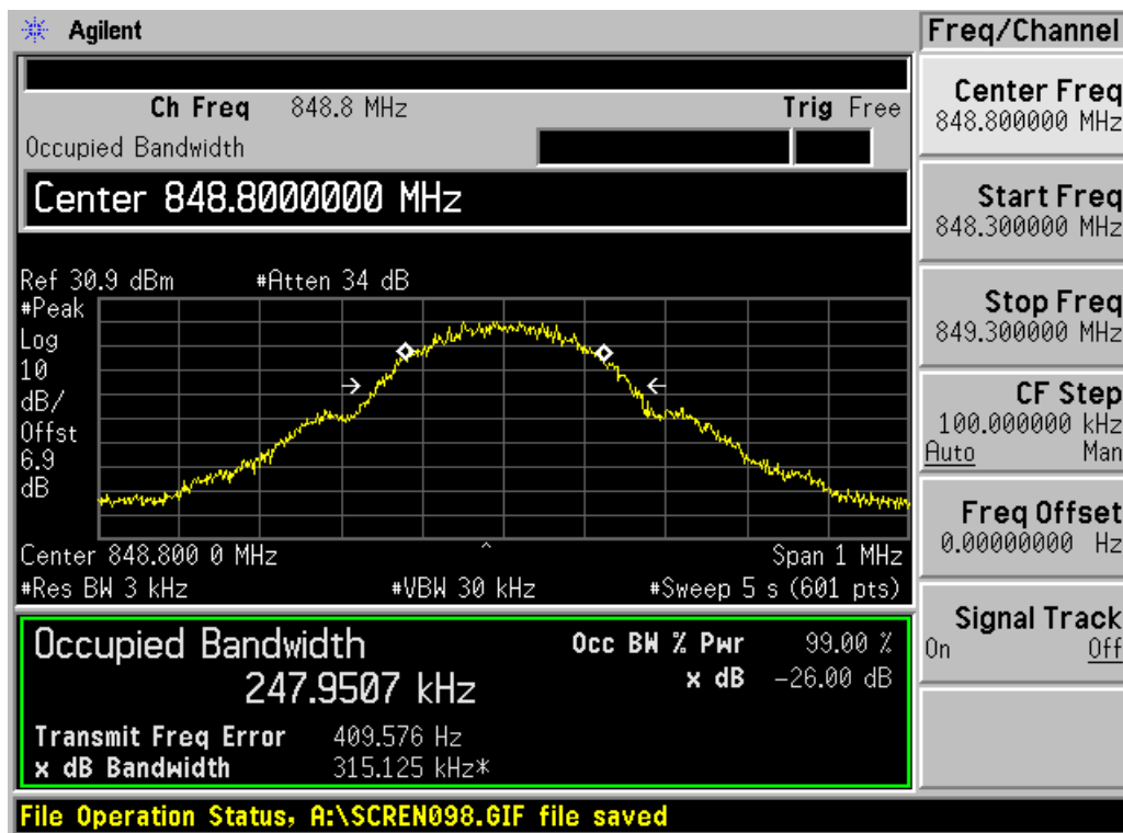
Channel 251
