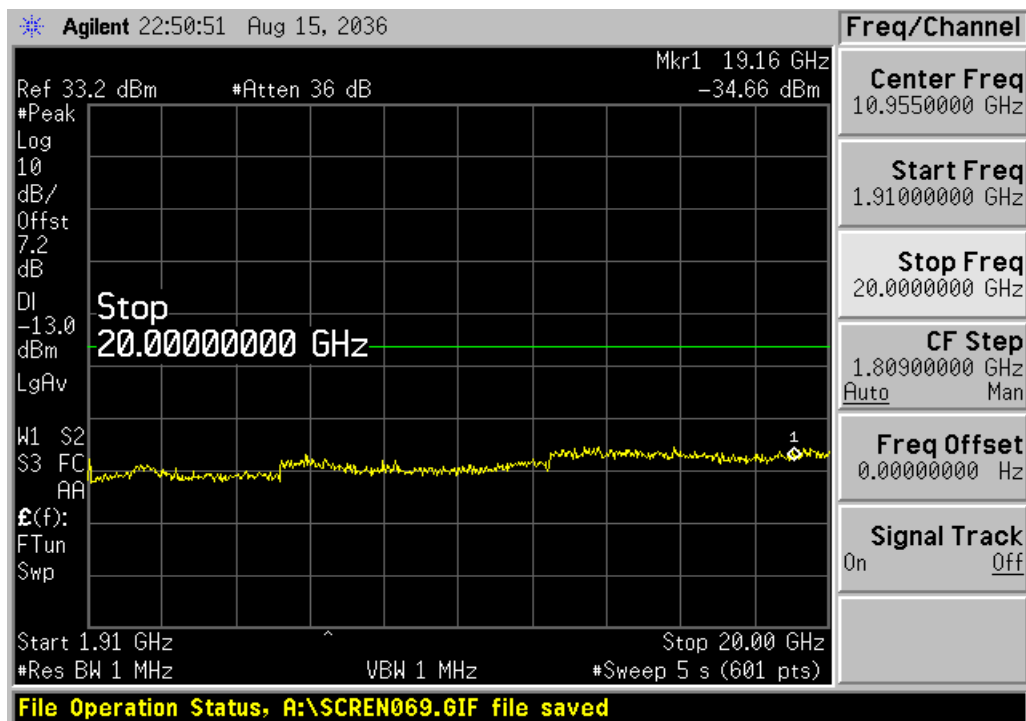
Channel 661, 1910MHz~20GHz
