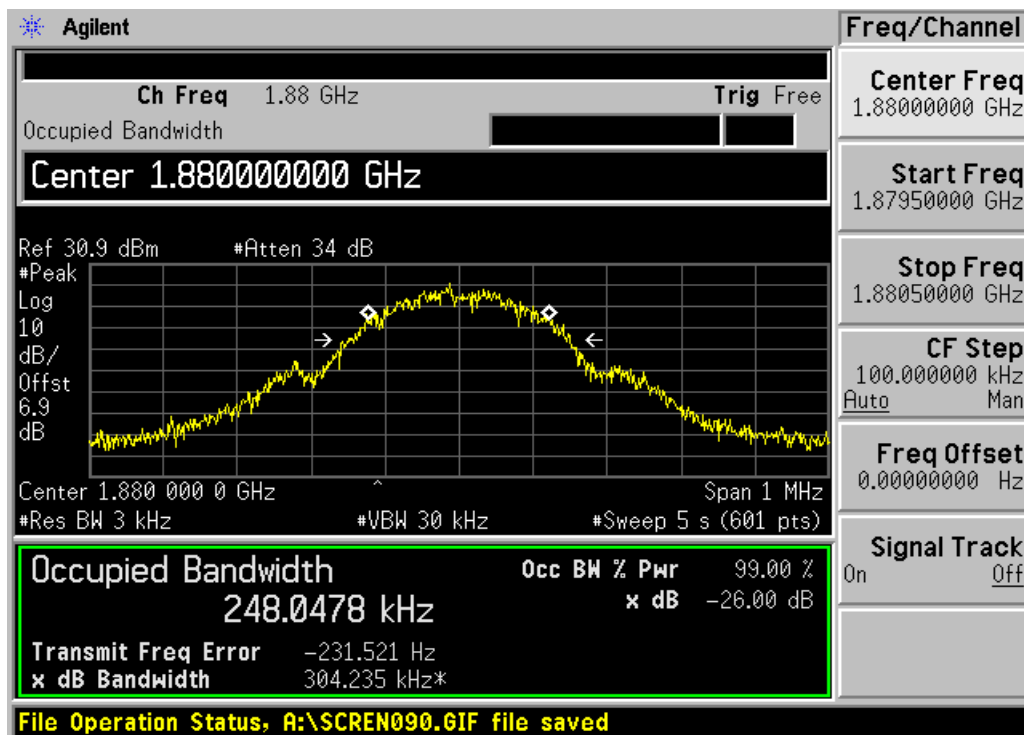
Channel 661
