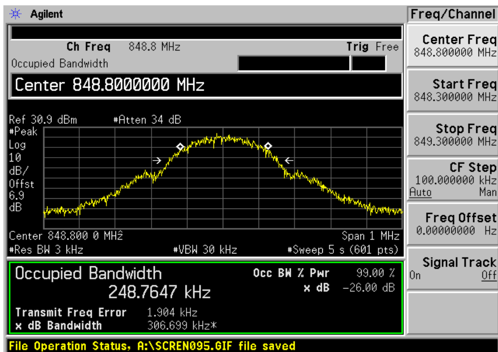
Channel 251
