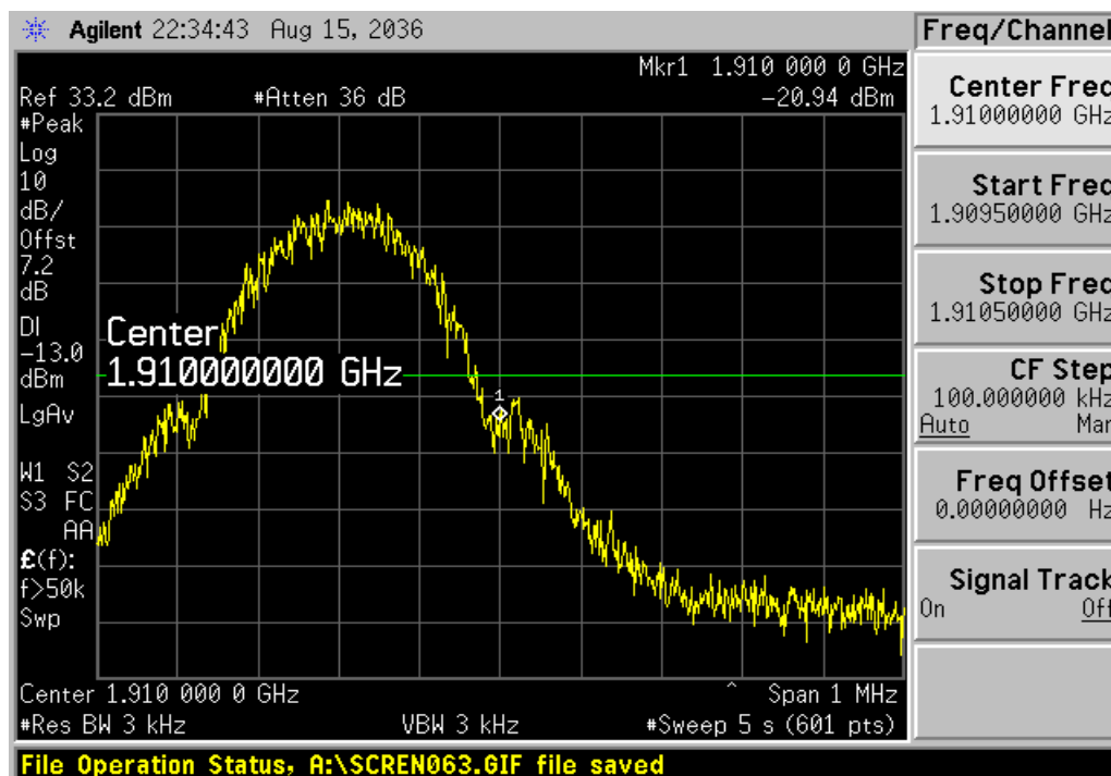
Channel 810
