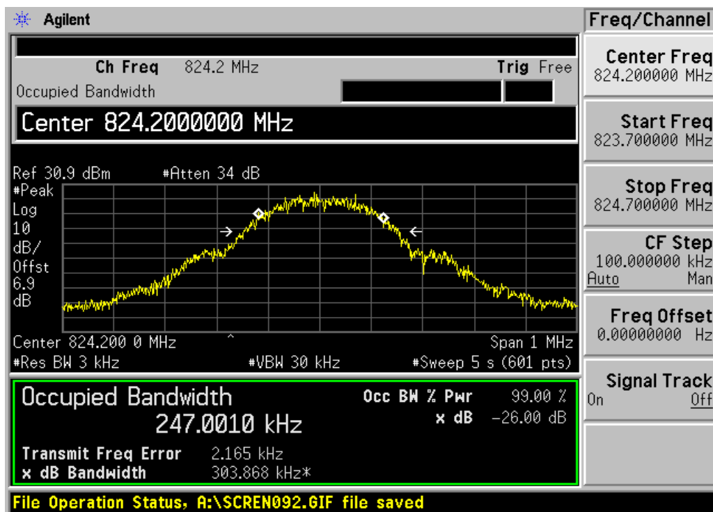
Channel 128
