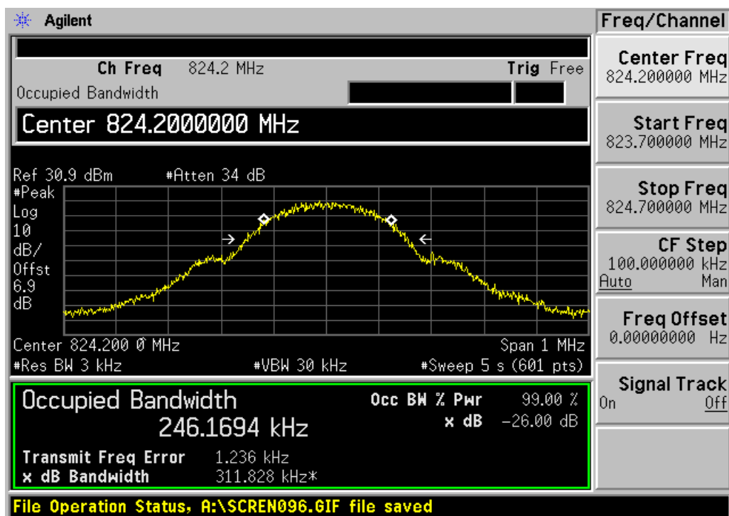
Channel 128
