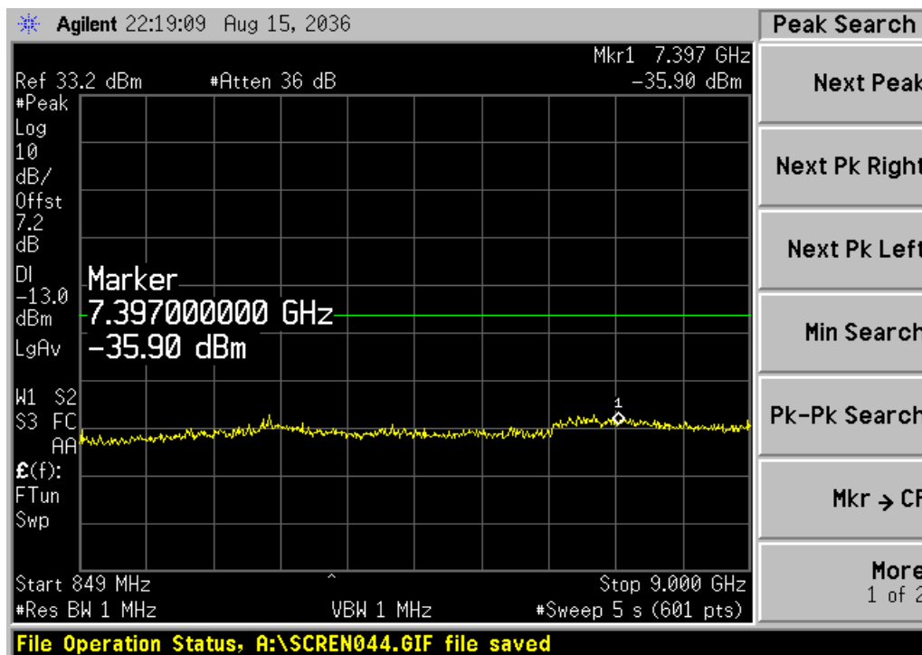
Channel 189, 849MHz~9GHz
