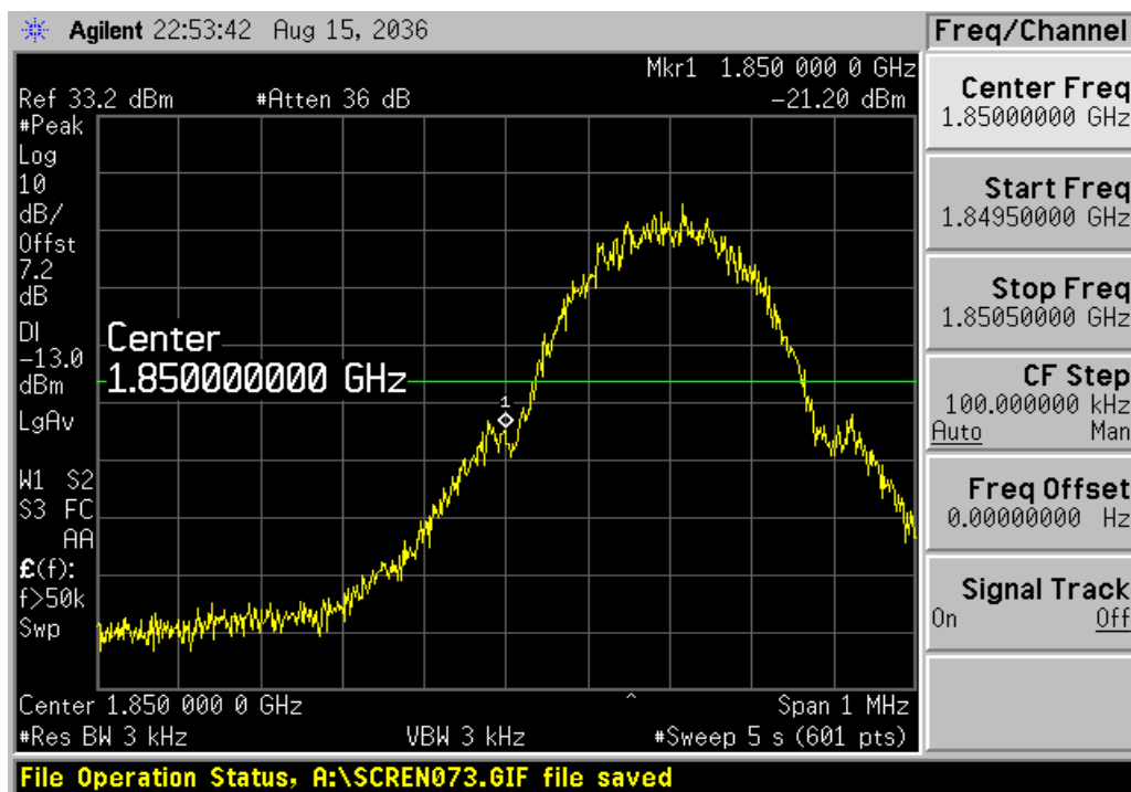
Channel 512
