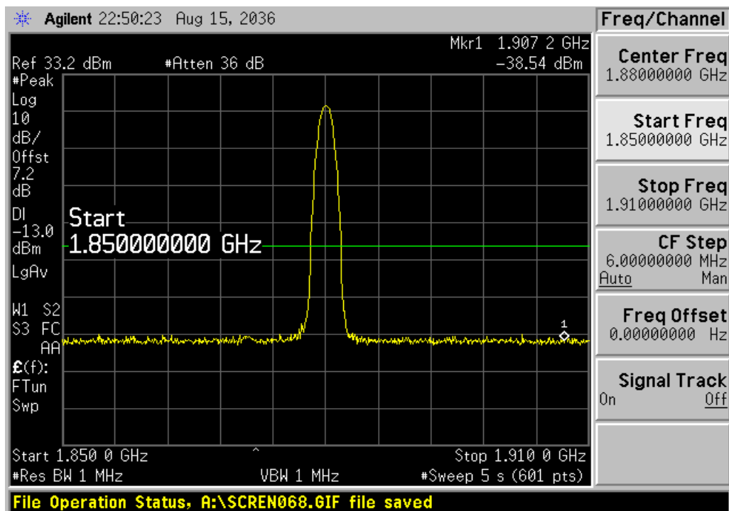
Channel 661, 1850MHz~1910MHz
