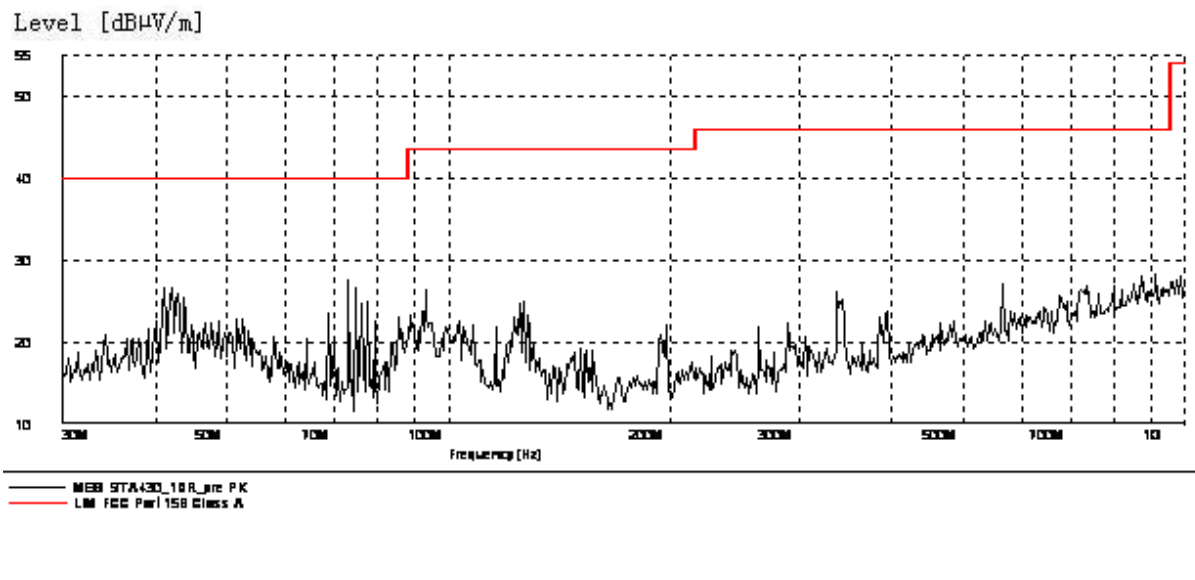
Figure A.3 Radiated Emission from 30MHz to 1GHz
