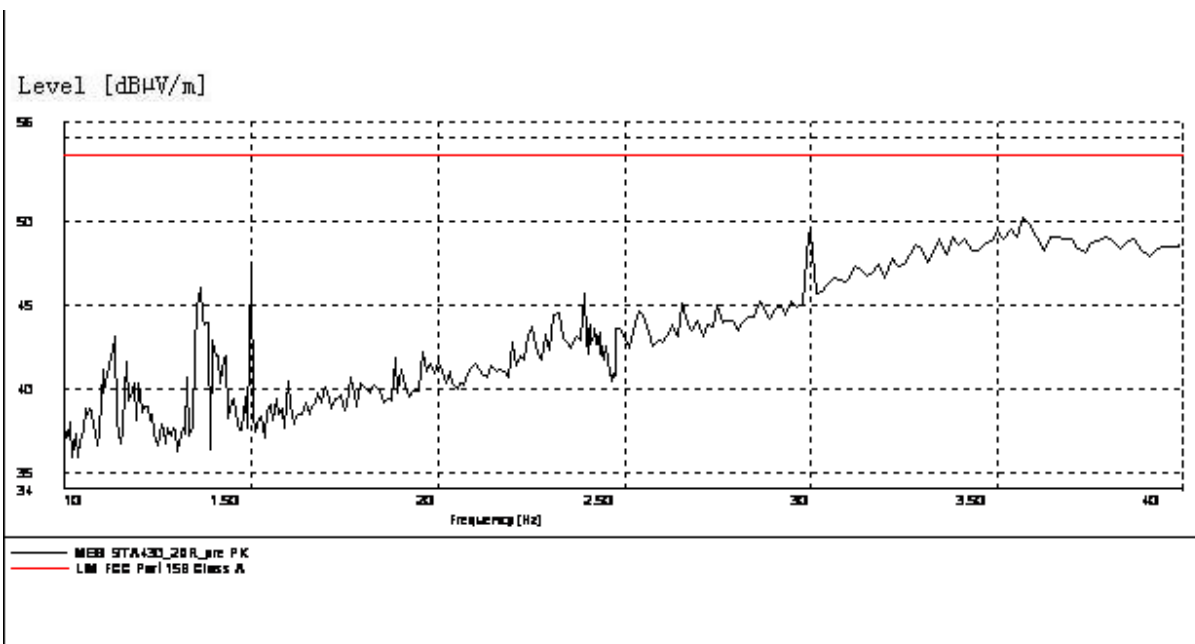
Figure A.4 Radiated Emission from 1GHz to 4GHz
