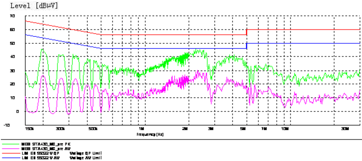
Figure A.5 Conducted Emission
