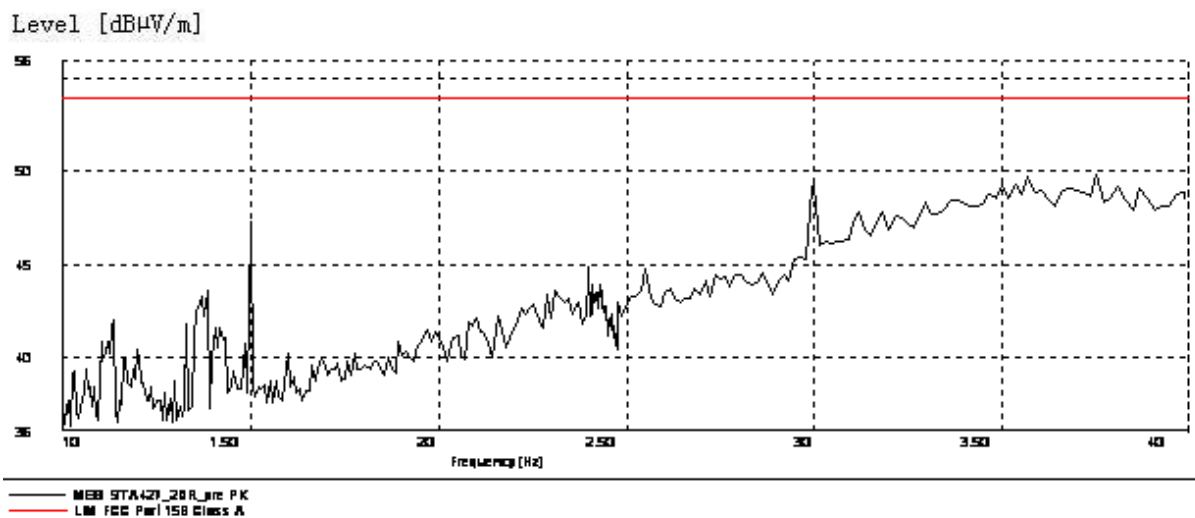
Figure A.4 Radiated Emission from 1GHz to 4GHz
