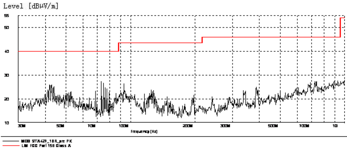
Figure A.3 Radiated Emission from 30MHz to 1GHz
