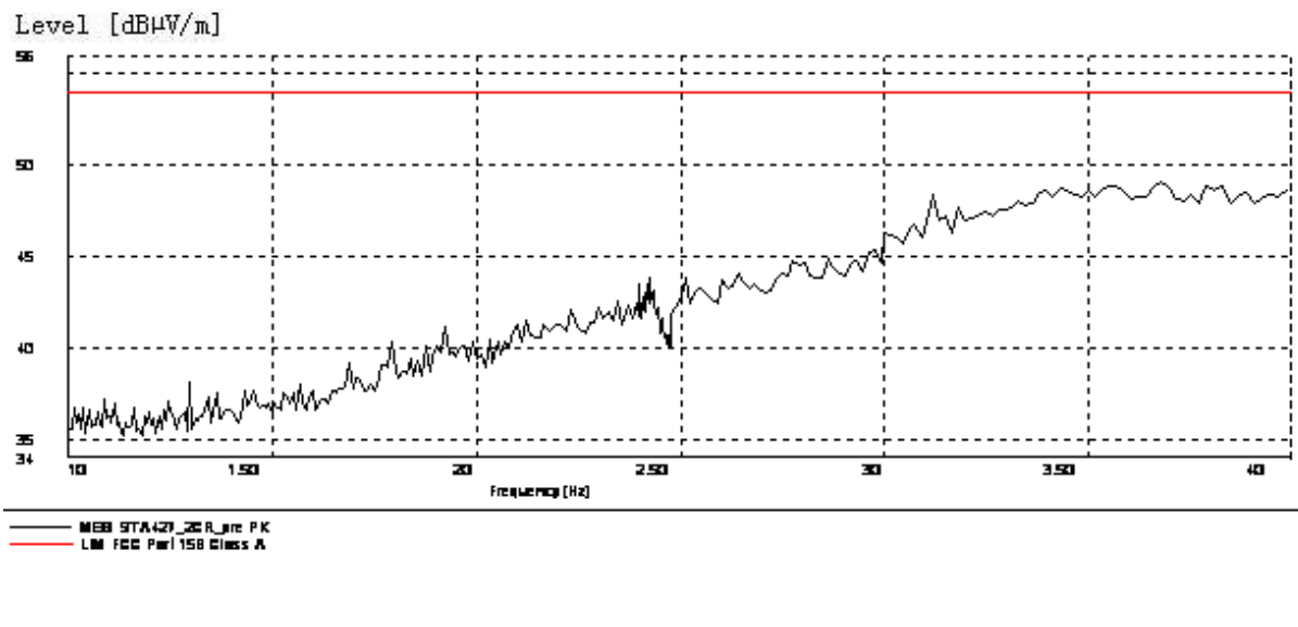
Figure A.2 Radiated Emission from 1GHz to 4GHz
