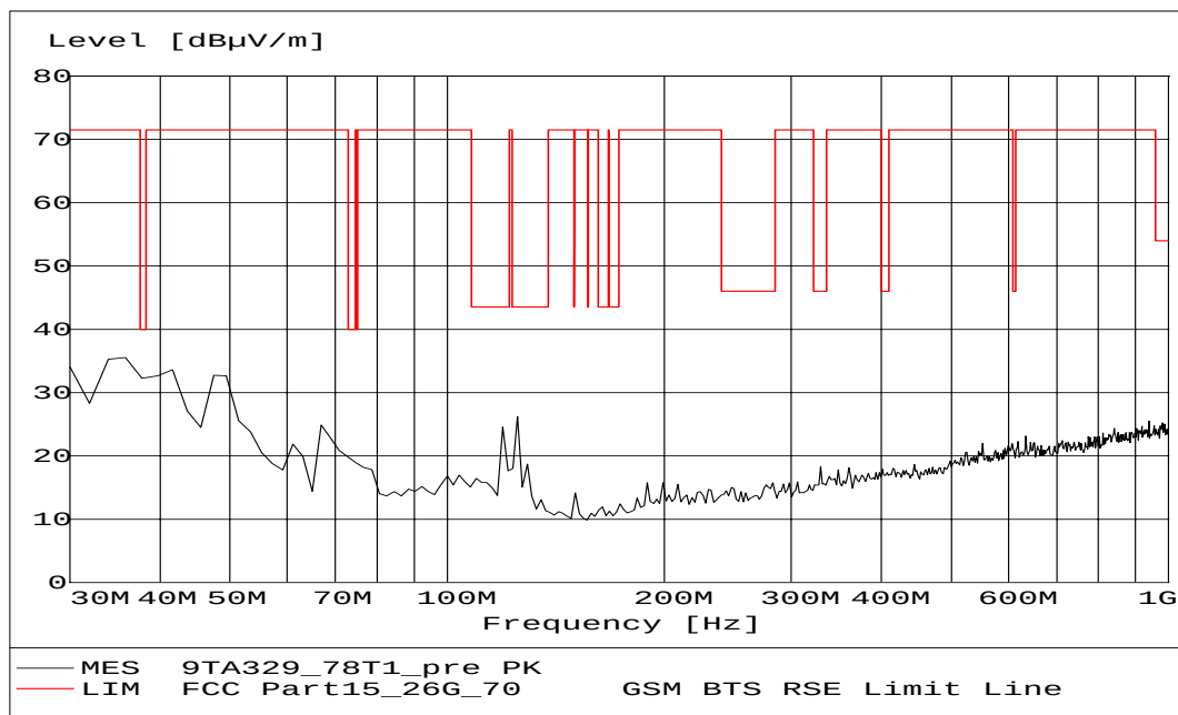
Fig. 20 Radiated emission: Channel 78, 30 MHz - 1 GHz
