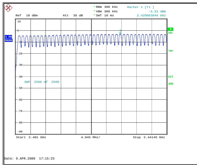
Fig. 32 Number of hopping frequencies: Channel 0 – 39
