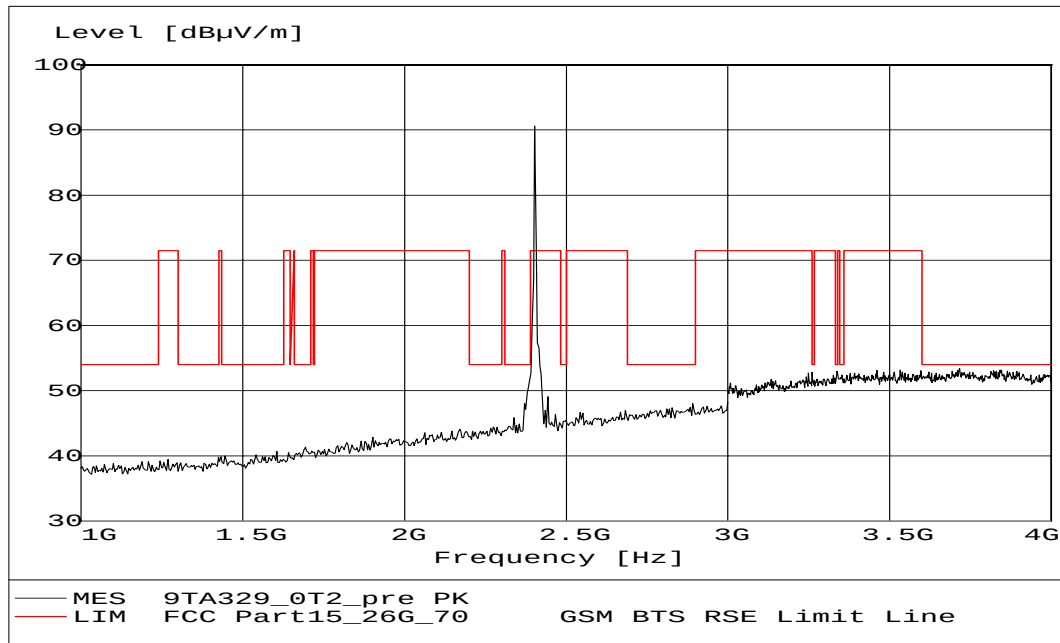
Fig. 15 Radiated emission: Channel 0, 1 GHz - 4 GHz
