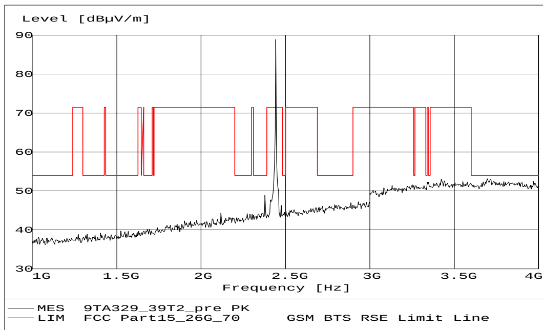
Fig. 18 Radiated emission: Channel 39, 1 GHz - 4 GHz
