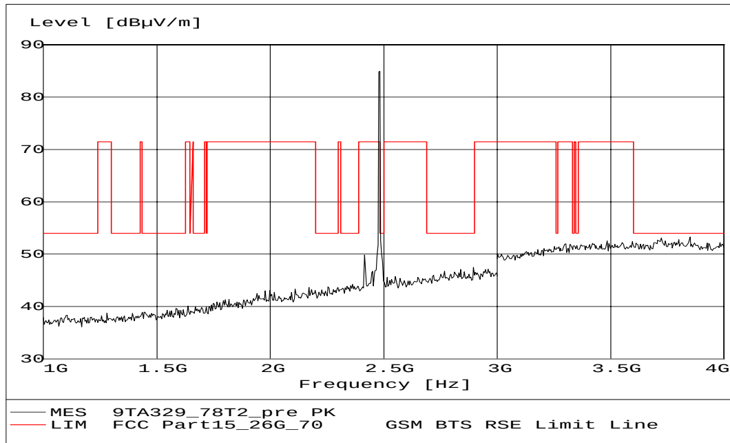
Fig. 21 Radiated emission: Channel 78, 1 GHz - 4 GHz
