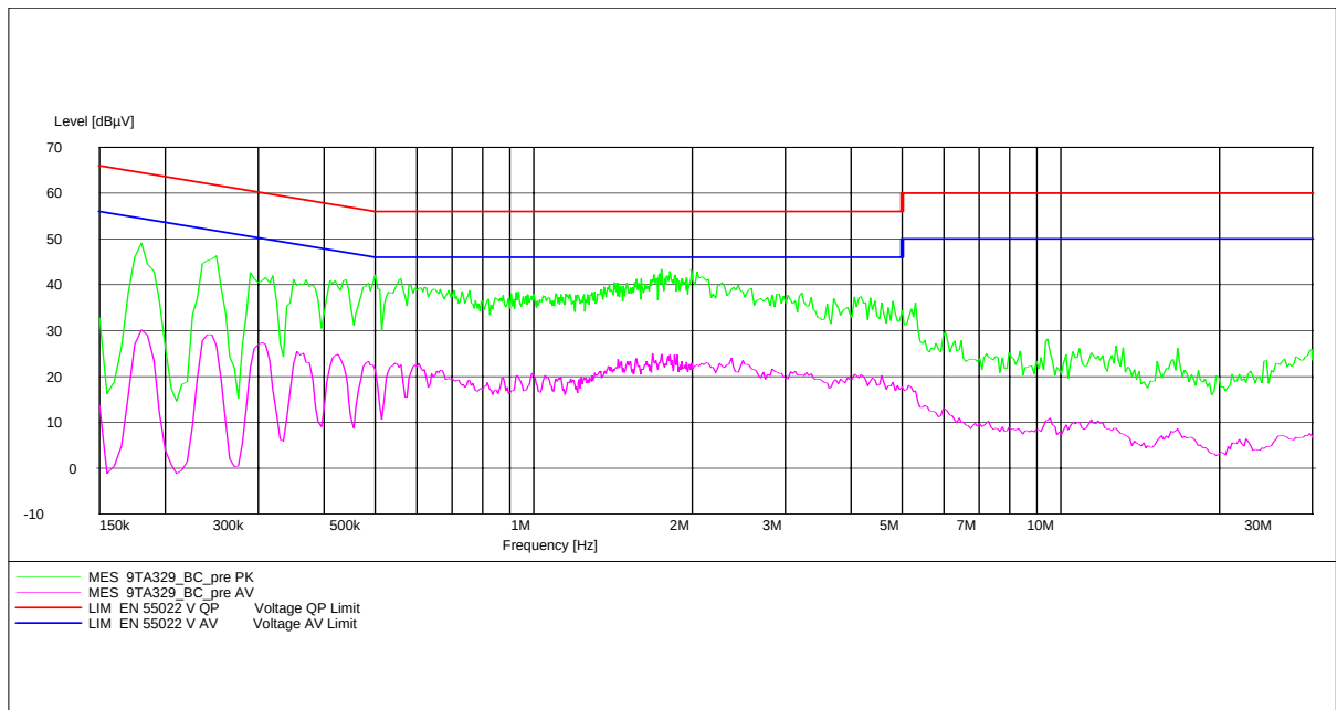
Fig. 34 AC Powerline Conducted Emission
