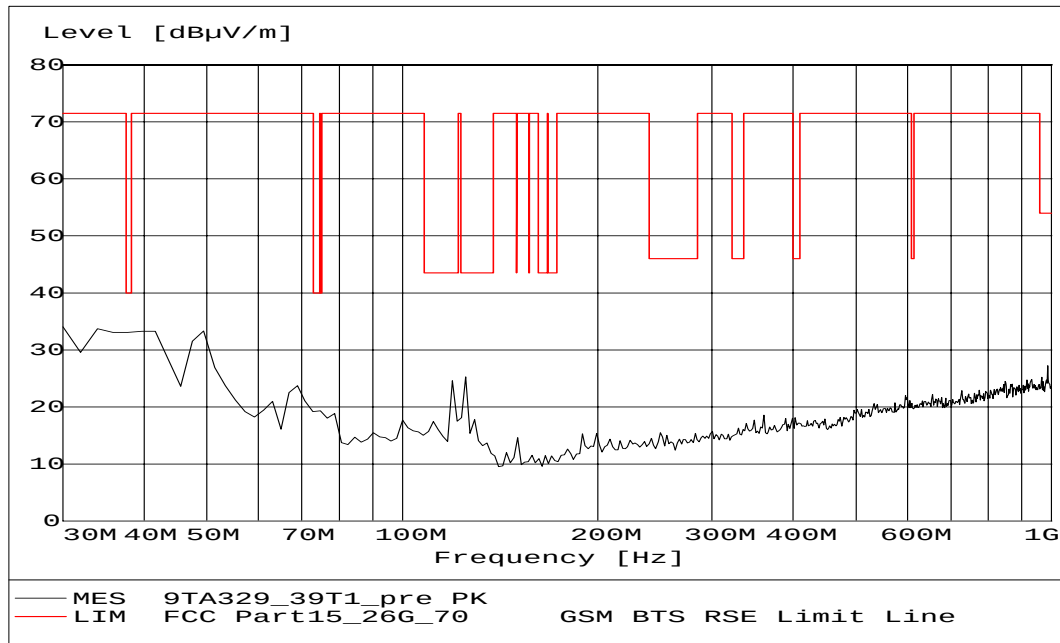
Fig. 17 Radiated emission: Channel 39, 30 MHz - 1 GHz
