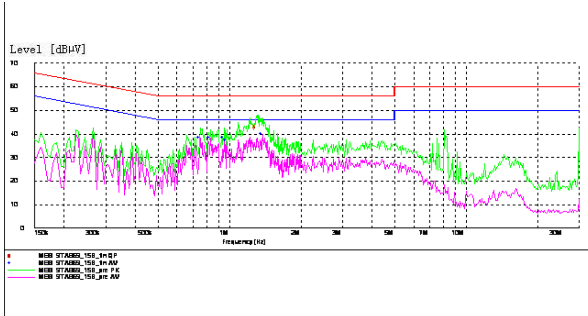
Figure A.3 Conducted Emission
