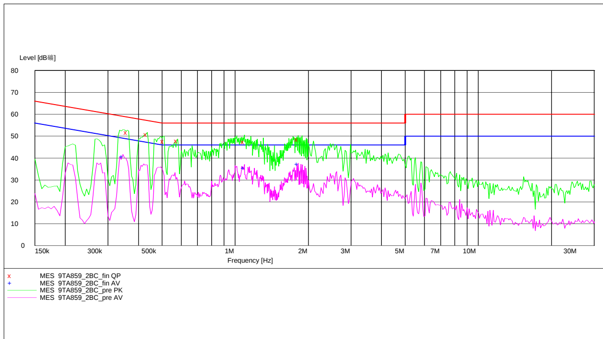
Fig. 37 AC Powerline Conducted Emission with charger
