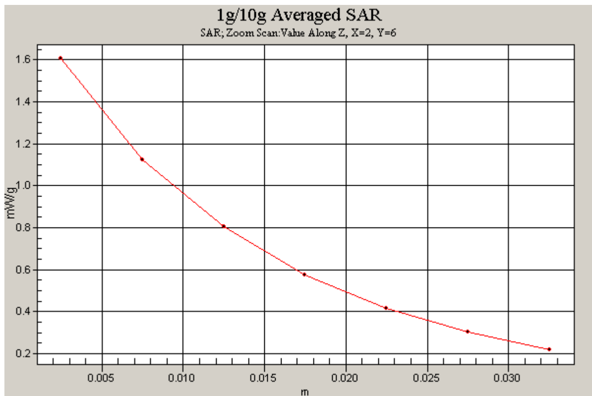
Figure 42 Z-Scan at power reference point (Body, Towards Ground, GSM 850 GPRS (4UP), Channel 128)
