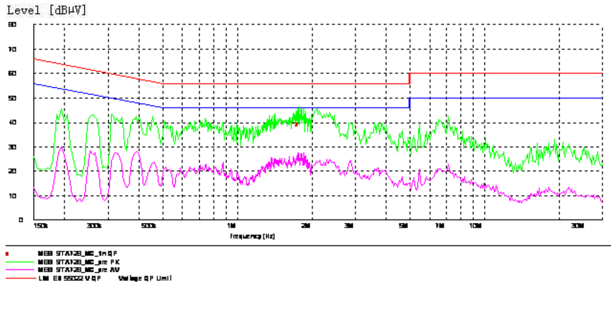
Figure A.5 Conducted Emission
