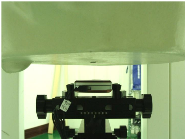
Face of the DUT with Phantom 2.5 cm Gap for Slide Off Mode
