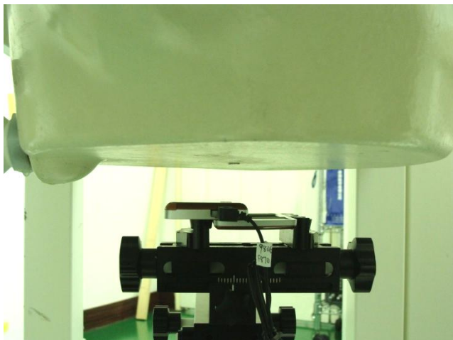
Face of the DUT with Phantom 2.5 cm Gap for Slide Right Mode
